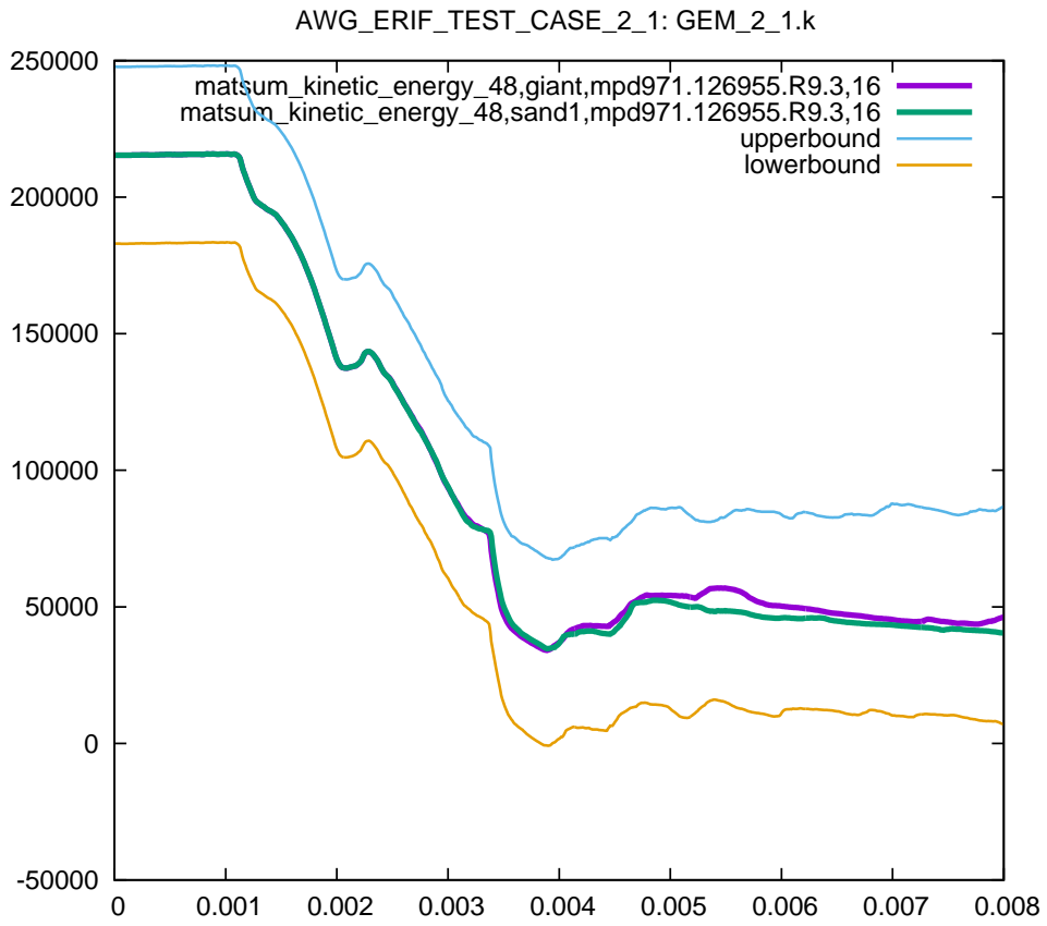
Figure 5: Kinetic energy part 48 (released blade), sub test case ID 1
