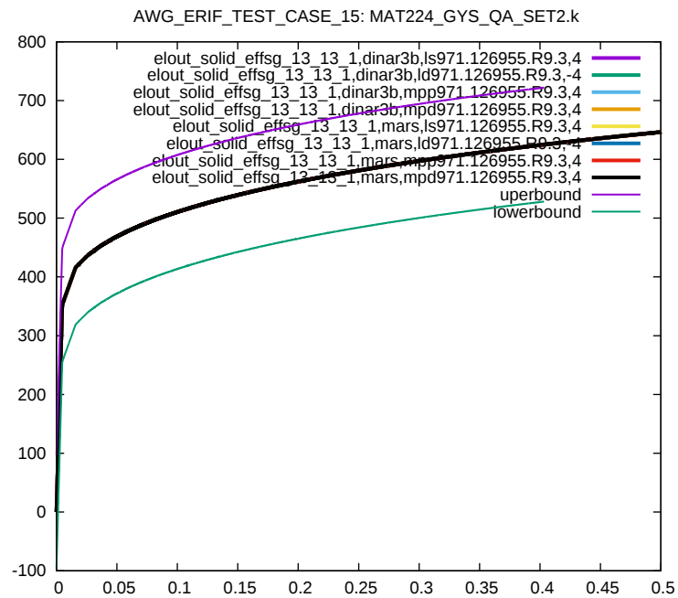
Figure 64: Cross platform results, Von Mises Stress, element ID 13, sub test case ID 3
