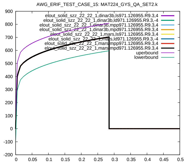
Figure 57: Cross platform results, z-component Stress, element ID 22, sub test case ID 3
