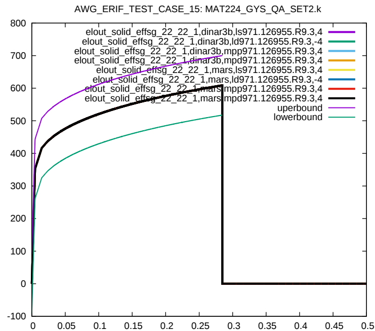
Figure 73: Cross platform results, Von Mises Stress, element ID 22, sub test case ID 3
