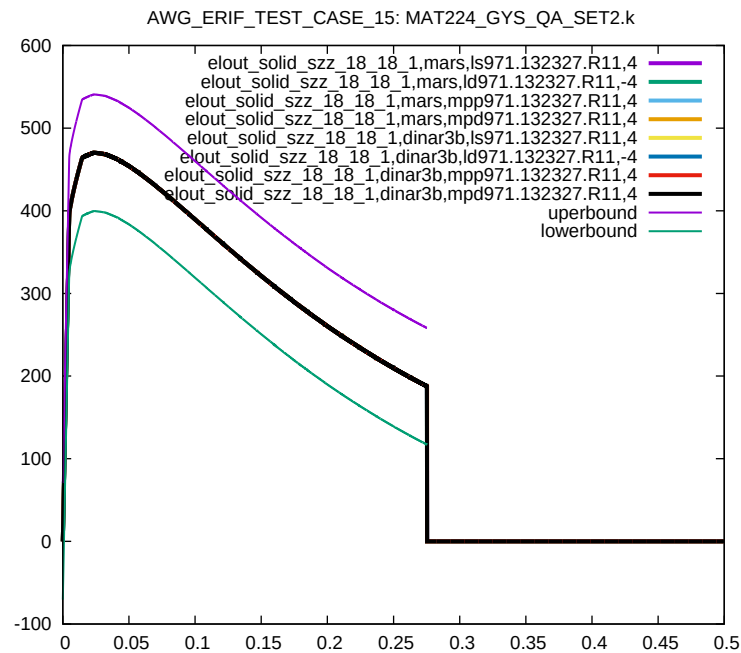
Figure 53: Cross platform results, z-component Stress, element ID 18, sub test case ID 3
