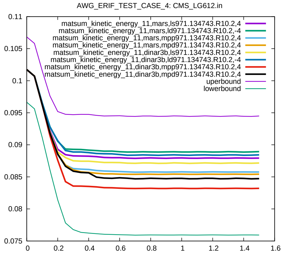
Figure 4: Cross platform results, kinetic energy part 11, sub test case ID 1
