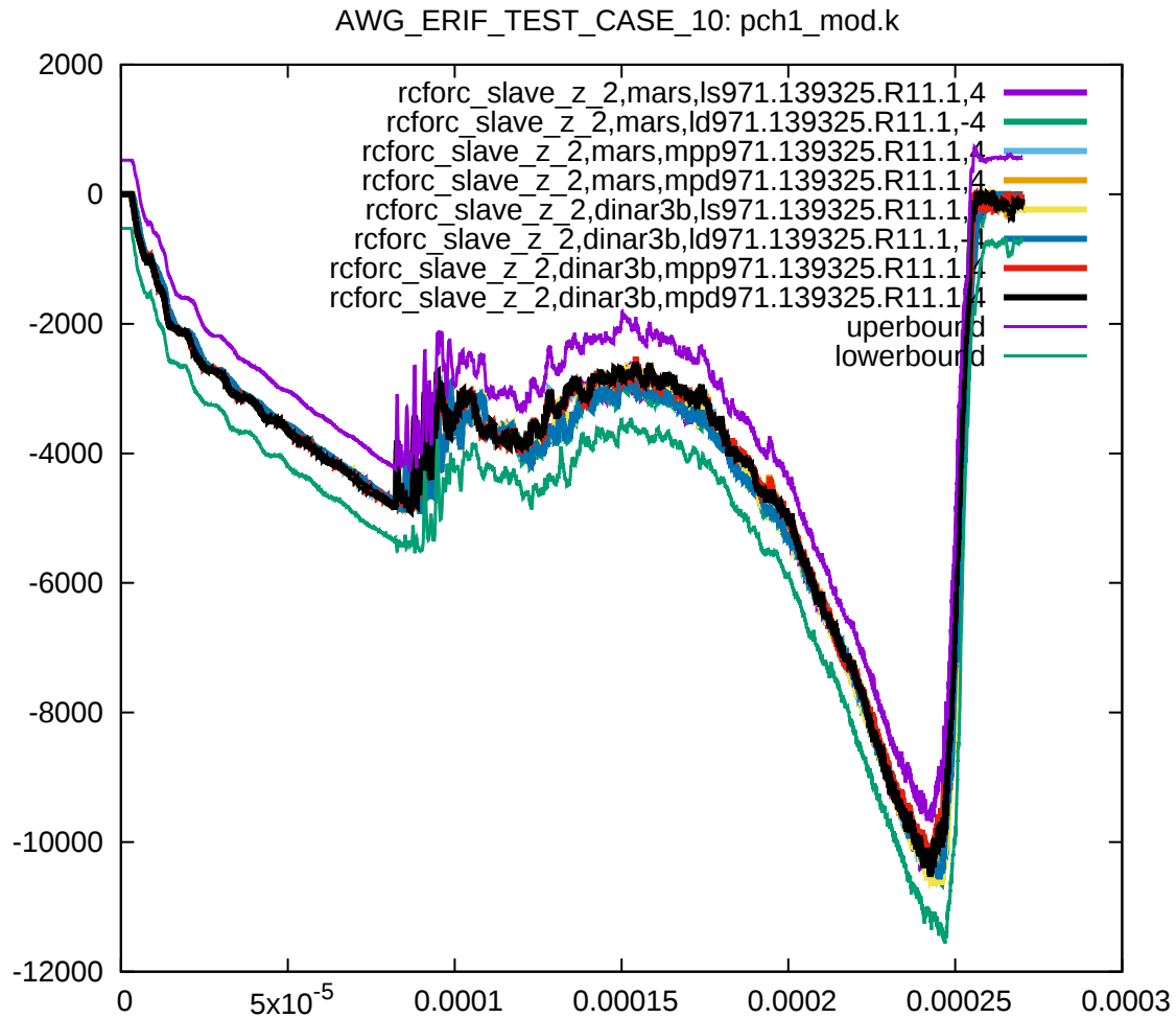
Figure 3: Cross platform results, resultant force in z-direction, sub test case ID 1
