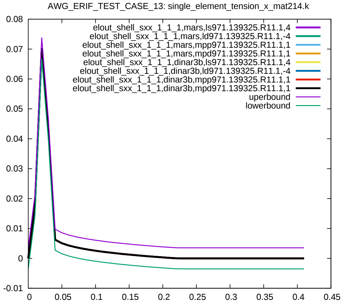
Figure 3: Cross platform results, stress in x-direction, integration point 1, sub test case ID 1
