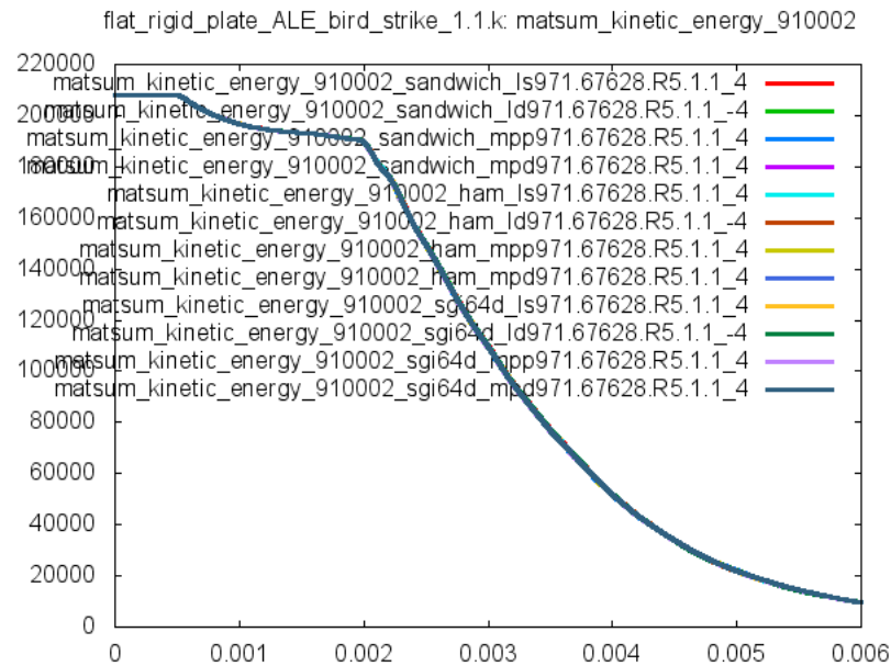
Figure 7: Cross platform results, kinetic energy part 910002 (bird body), sub test case ID 2
