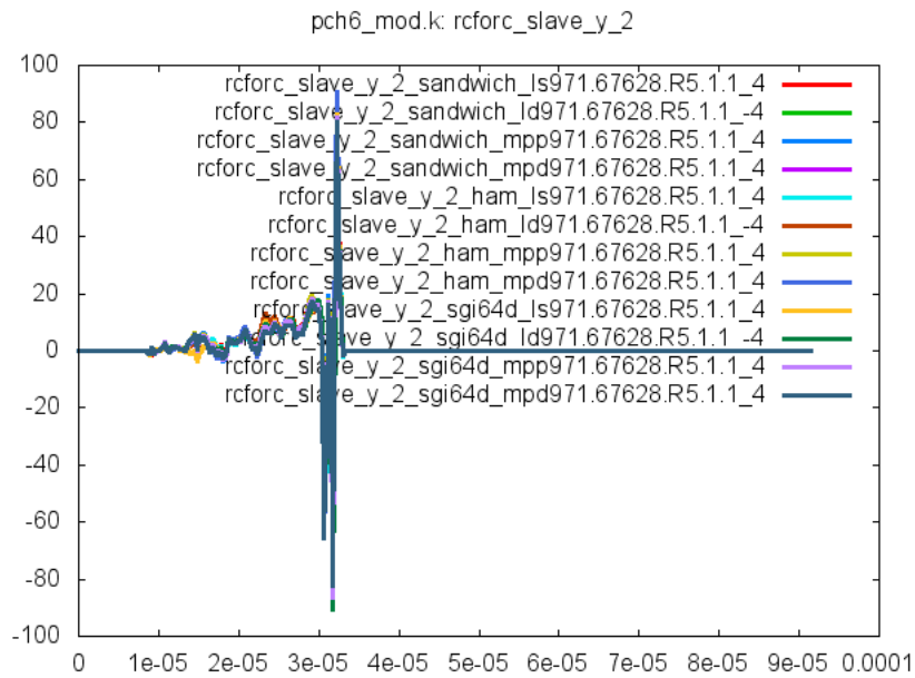
Figure 7: Cross platform results, resultant force in y-direction, sub test case ID 2
