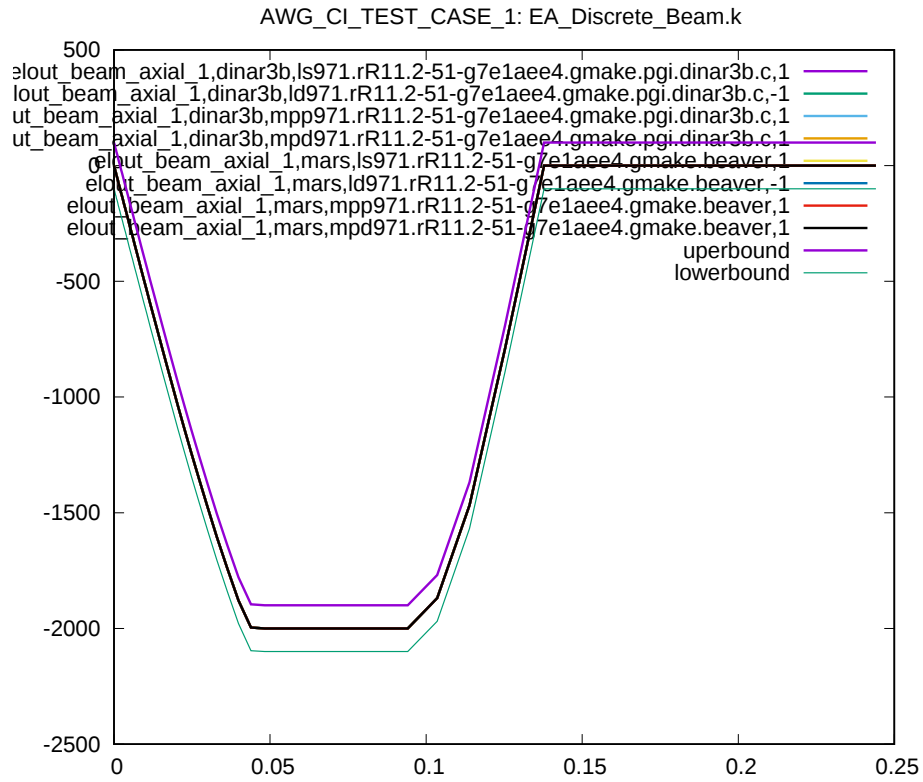
Figure 5: Cross platform results, axial force resultant beam 1
