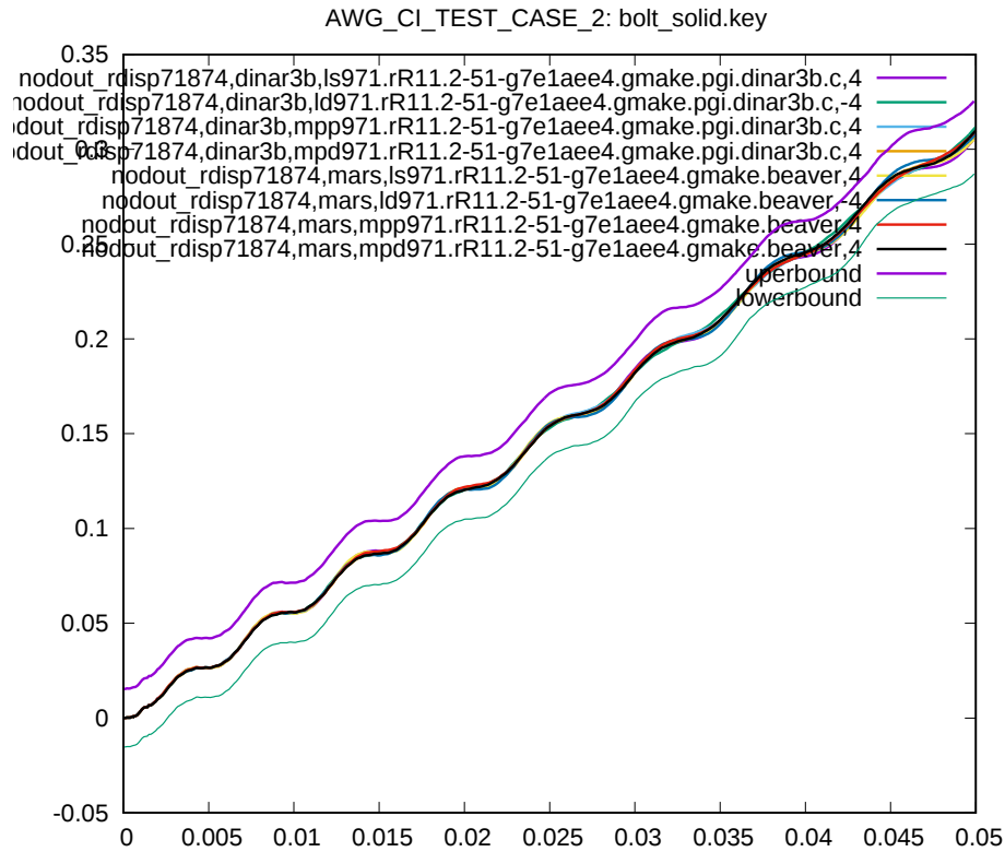
Figure 2: Cross platform results, nodal resultant displacement node 71874, sub test case ID 1
