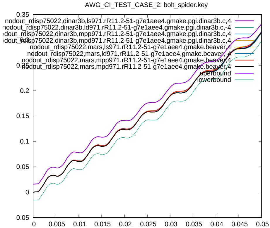
Figure 4: Cross platform results, nodal resultant displacement node 75022, sub test case ID 2
