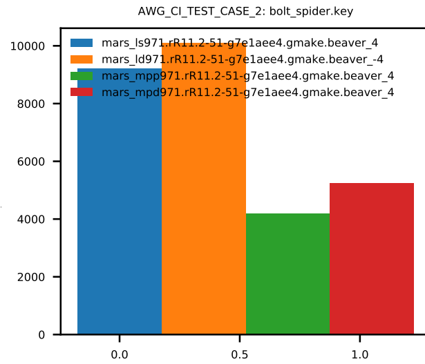
Figure 7: Cross platform results, CPU time (s)
