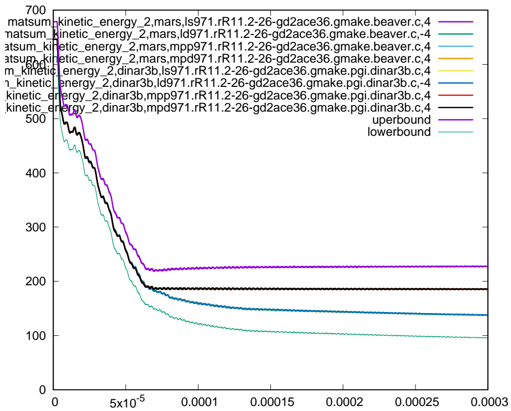
Figure 36: Cross platform results, kinetic energy part 2, sub test case ID 7, 105% ballistic limit
