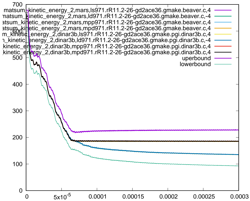
Figure 33: Cross platform results, kinetic energy part 2, sub test case ID 4, 105% ballistic limit
