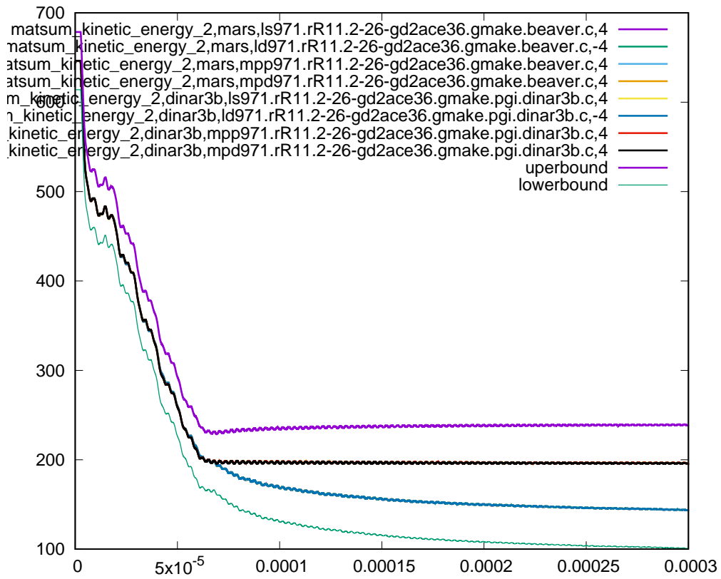
Figure 34: Cross platform results, kinetic energy part 2, sub test case ID 5, 105% ballistic limit
