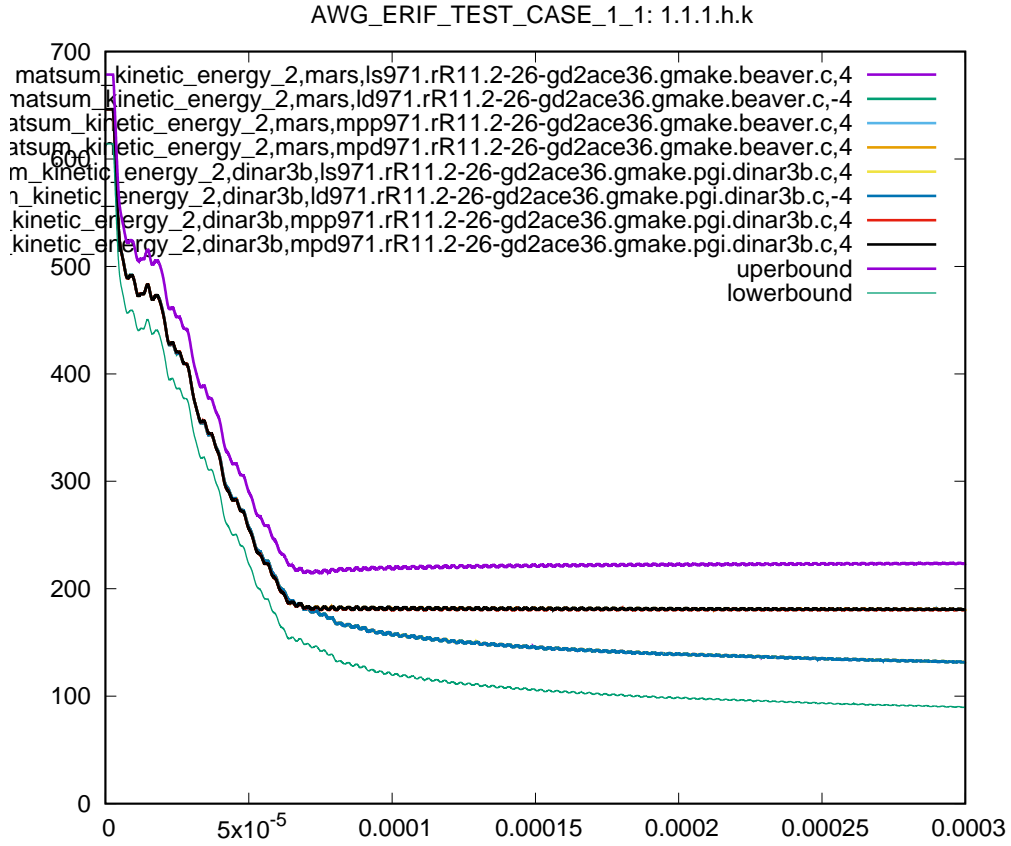
Figure 30: Cross platform results, kinetic energy part 2, sub test case ID 1, 105% ballistic limit
