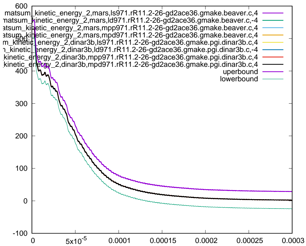
Figure 49: Cross platform results, kinetic energy part 2, sub test case ID 7, 95% ballistic limit
