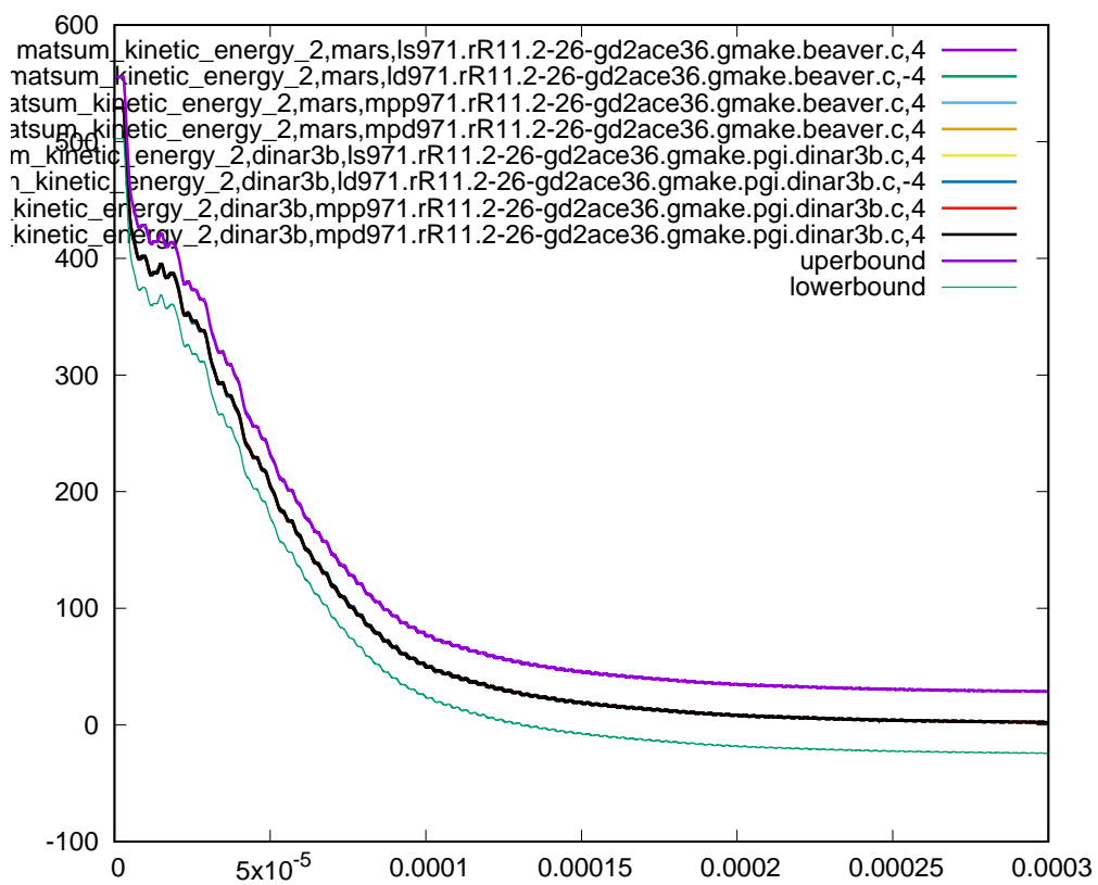
Figure 44: Cross platform results, kinetic energy part 2, sub test case ID 2, 95% ballistic limit
