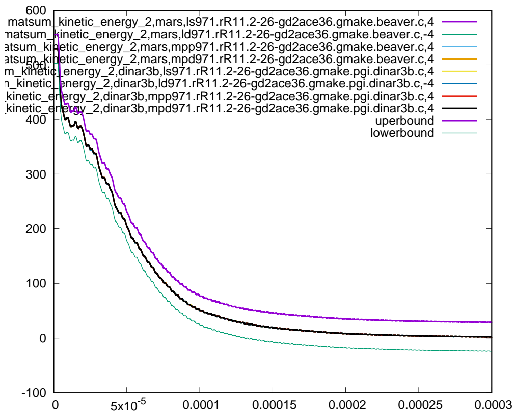
Figure 48: Cross platform results, kinetic energy part 2, sub test case ID 6, 95% ballistic limit
