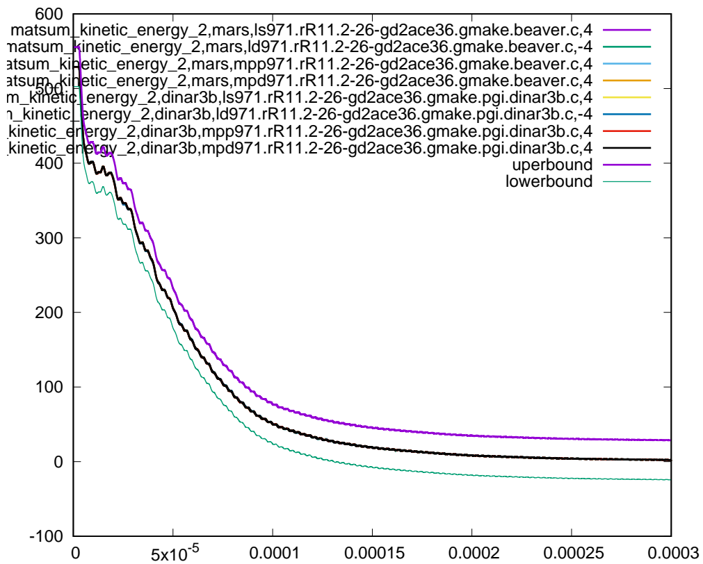
Figure 46: Cross platform results, kinetic energy part 2, sub test case ID 4, 95% ballistic limit
