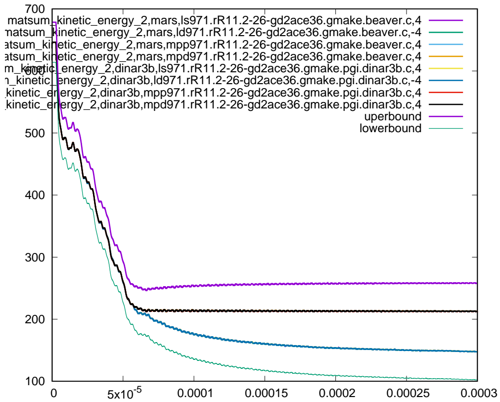
Figure 37: Cross platform results, kinetic energy part 2, sub test case ID 8, 105% ballistic limit
