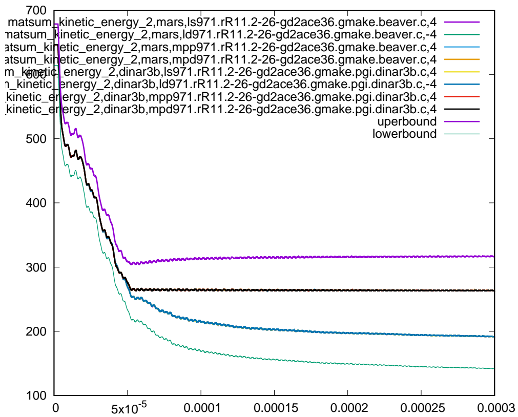
Figure 38: Cross platform results, kinetic energy part 2, sub test case ID 9, 105% ballistic limit
