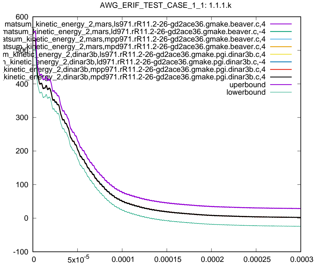
Figure 43: Cross platform results, kinetic energy part 2, sub test case ID 1, 95% ballistic limit
