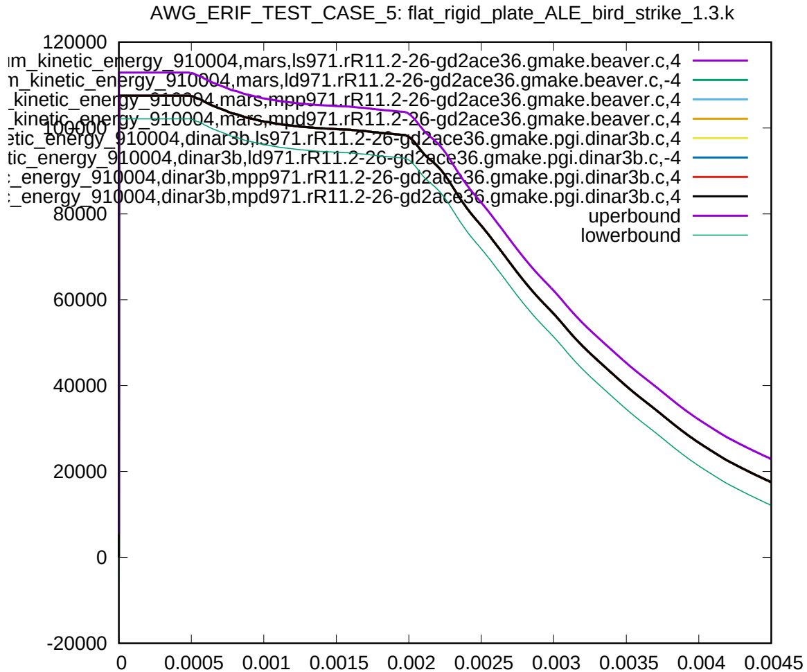
Figure 7: Cross platform results, kinetic energy part 910004 (bird body), sub test case ID 2
