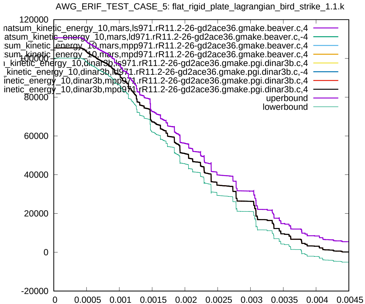
Figure 5: Cross platform results, kinetic energy part 10 (bird body), sub test case ID 1
