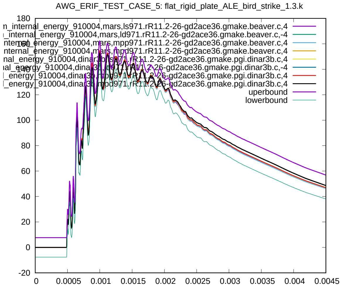
Figure 8: Cross platform results, internal energy part 920004 (bird body), sub test case ID 2
