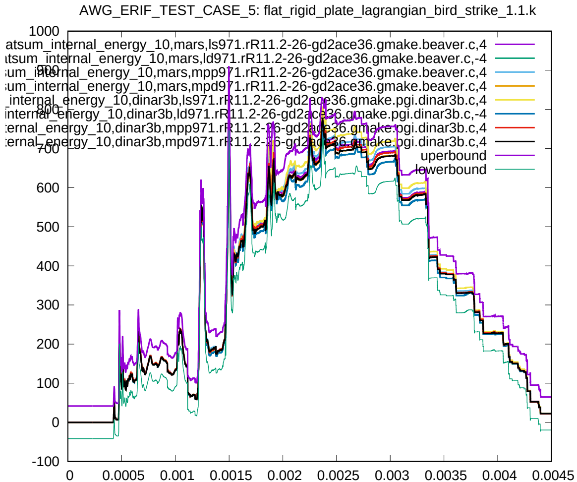
Figure 6: Cross platform results, internal energy part 10 (bird body), sub test case ID 1
