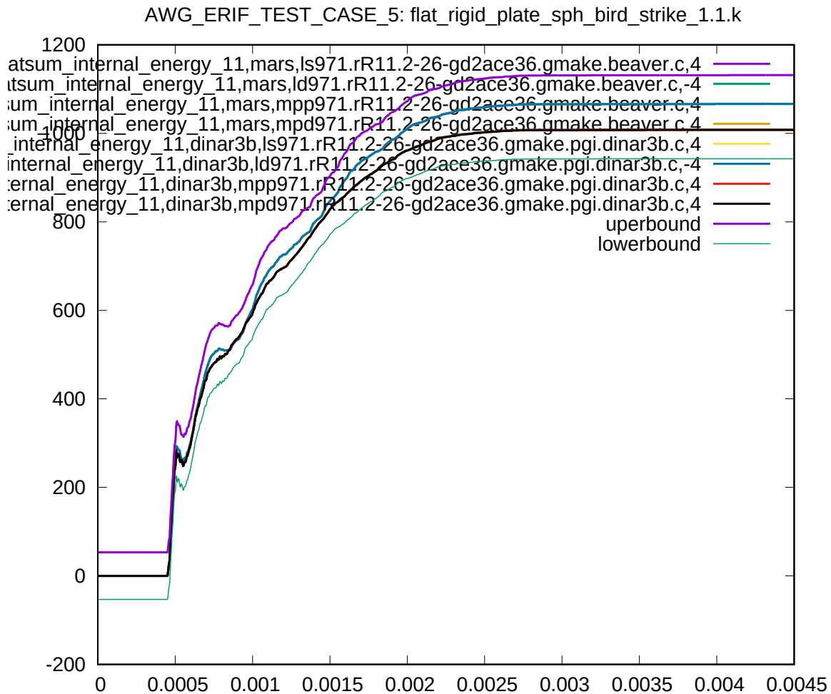
Figure 10: Cross platform results, internal energy part 11 (bird body), sub test case ID 3
