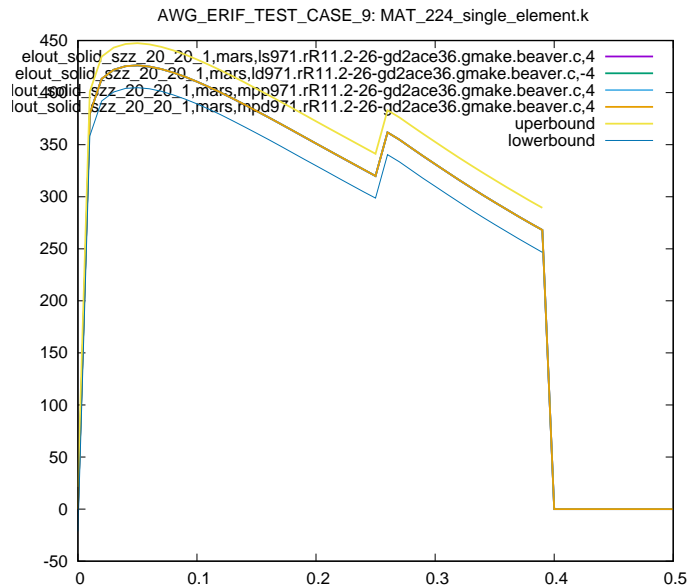
Figure 22: Cross platform results, zz stress element id 20, sub test case ID 1
