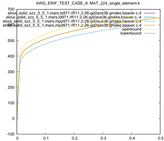
Figure 7: Cross platform results, zz stress element id 5, sub test case ID 1
