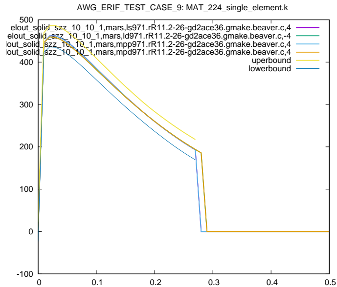
Figure 12: Cross platform results, zz stress element id 10, sub test case ID 1
