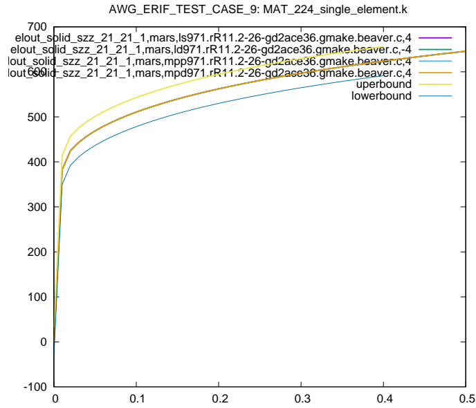
Figure 23: Cross platform results, zz stress element id 21, sub test case ID 1
