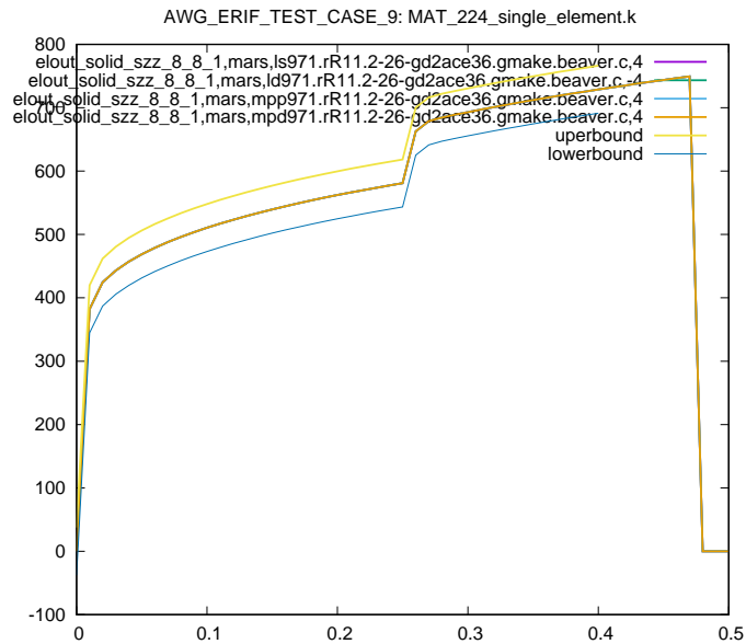
Figure 10: Cross platform results, zz stress element id 8, sub test case ID 1
