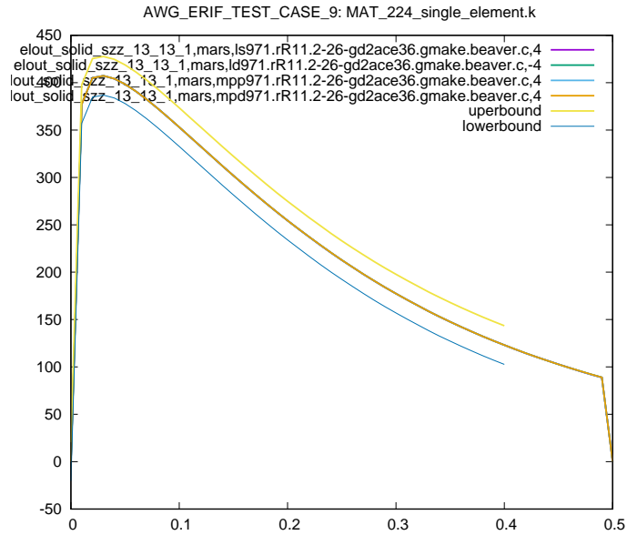
Figure 15: Cross platform results, zz stress element id 13, sub test case ID 1
