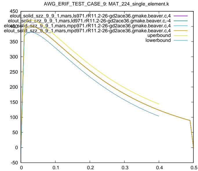
Figure 11: Cross platform results, zz stress element id 9, sub test case ID 1
