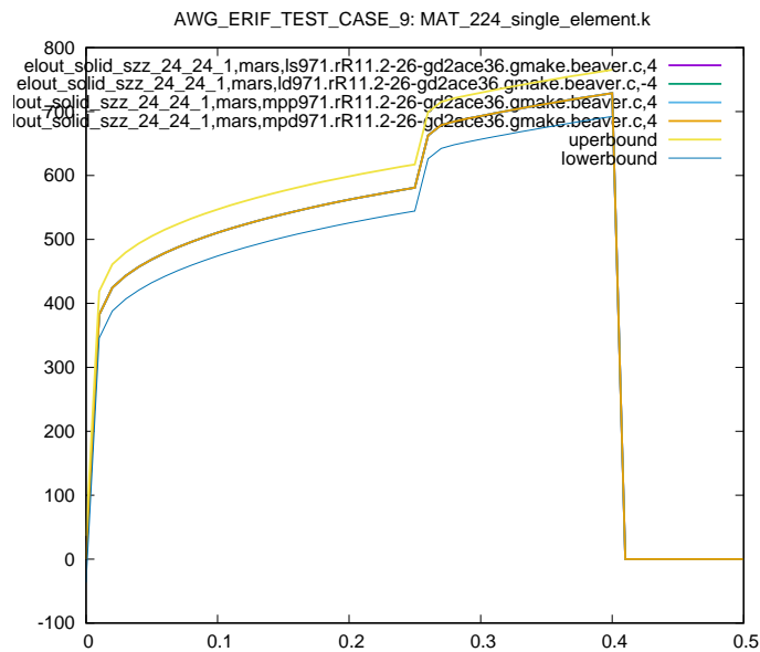
Figure 26: Cross platform results, zz stress element id 24, sub test case ID 1
