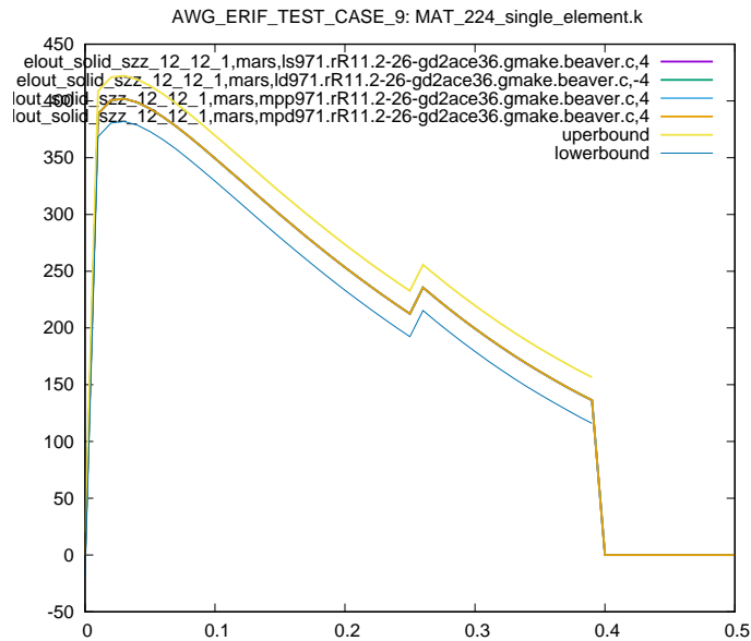
Figure 14: Cross platform results, zz stress element id 12, sub test case ID 1
