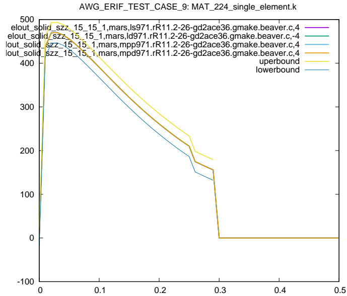
Figure 17: Cross platform results, zz stress element id 15, sub test case ID 1
