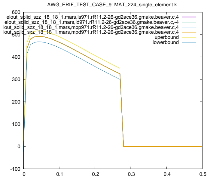
Figure 20: Cross platform results, zz stress element id 18, sub test case ID 1
