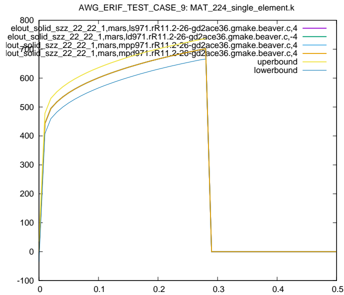
Figure 24: Cross platform results, zz stress element id 22, sub test case ID 1
