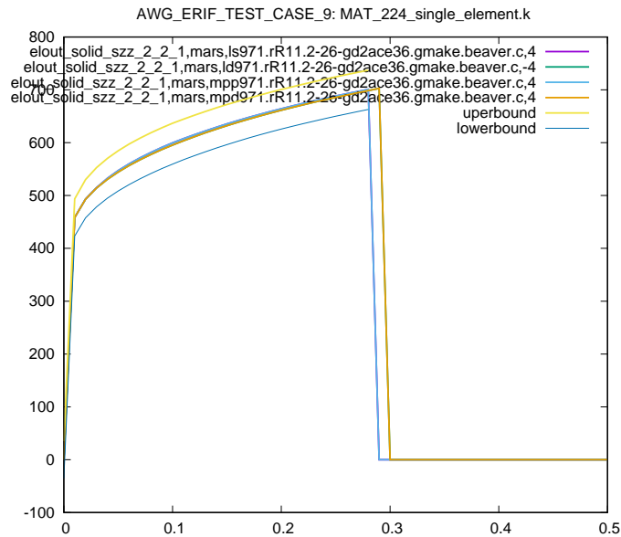
Figure 4: Cross platform results, zz stress element id 2, sub test case ID 1
