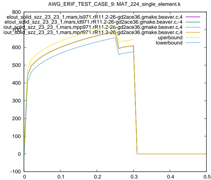
Figure 25: Cross platform results, zz stress element id 23, sub test case ID 1
