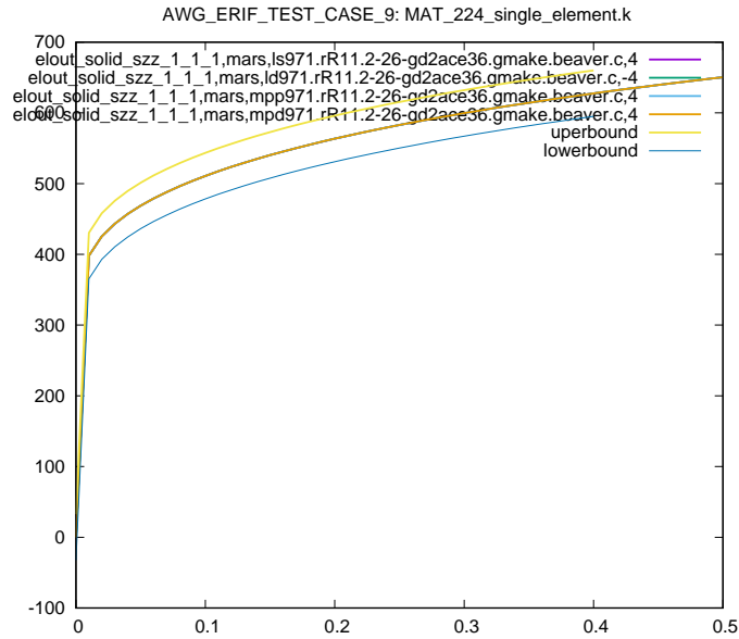
Figure 3: Cross platform results, zz stress element id 1, sub test case ID 1
