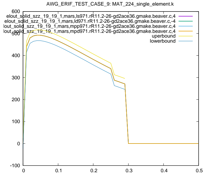
Figure 21: Cross platform results, zz stress element id 19, sub test case ID 1
