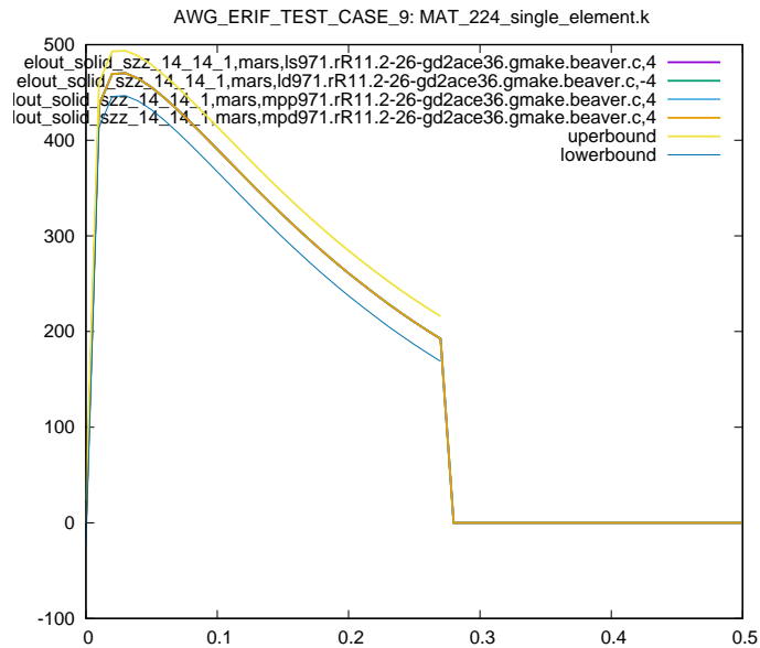
Figure 16: Cross platform results, zz stress element id 14, sub test case ID 1
