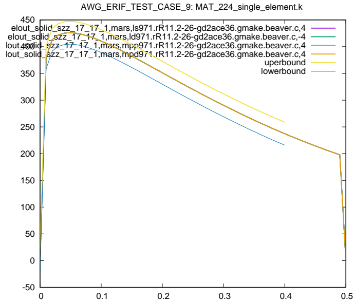
Figure 19: Cross platform results, zz stress element id 17, sub test case ID 1
