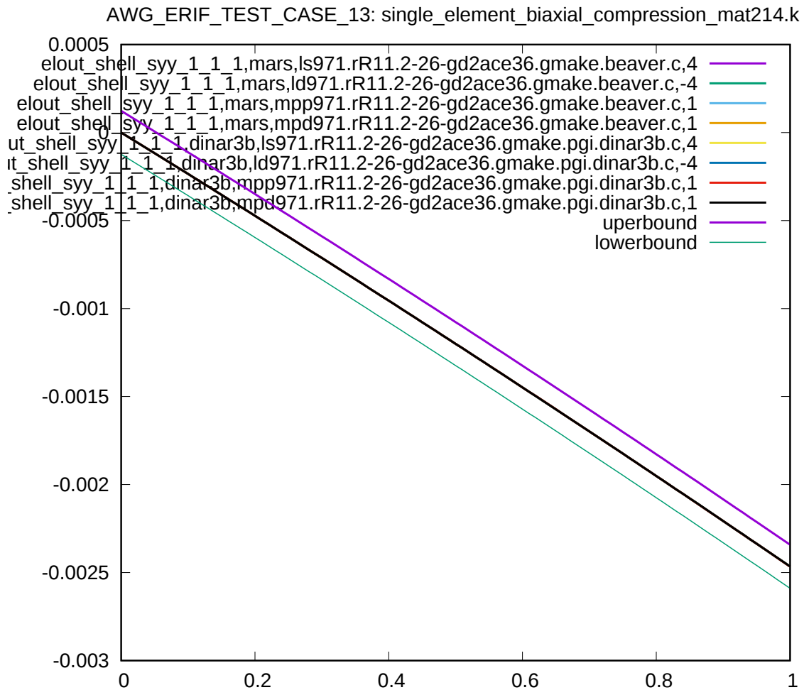
Figure 14: Cross platform results, stress in y-direction, integration point 1, sub test case ID 8
