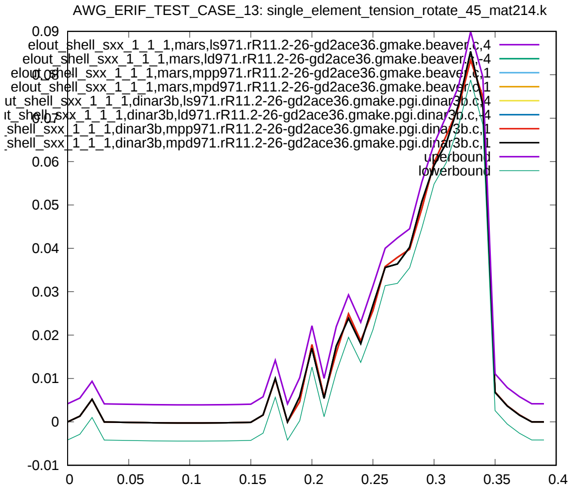
Figure 7: Cross platform results, stress in x-direction, integration point 1, sub test case ID 5
