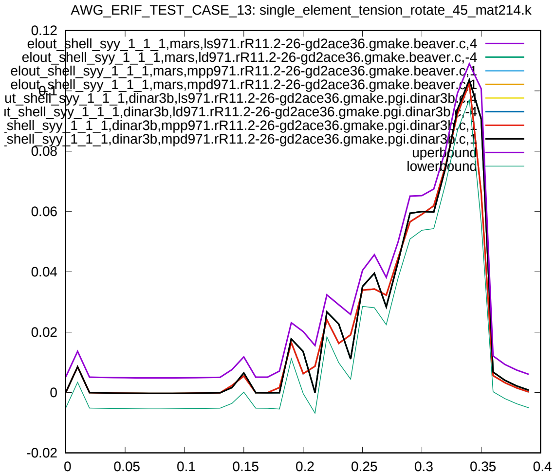
Figure 8: Cross platform results, stress in y-direction, integration point 1, sub test case ID 5
