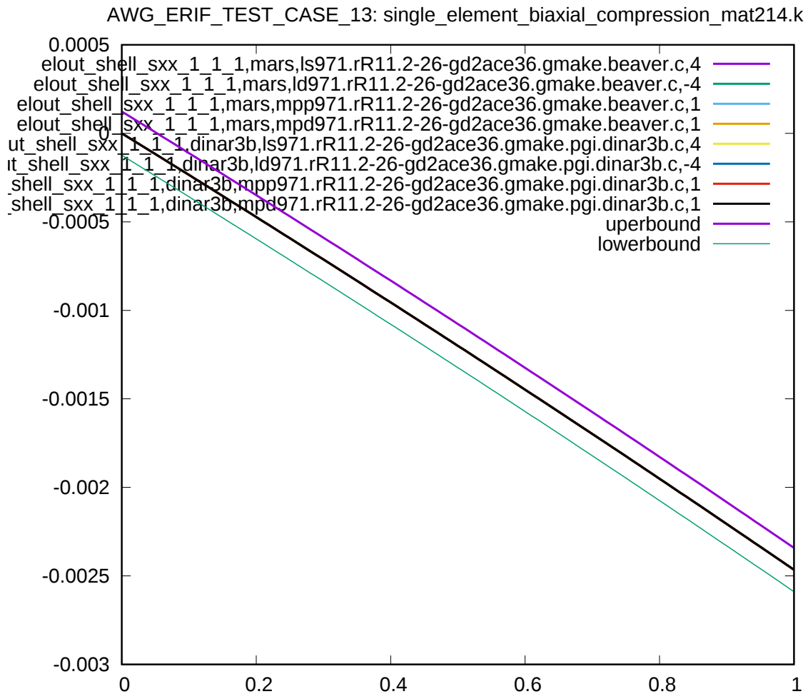
Figure 13: Cross platform results, stress in x-direction, integration point 1, sub test case ID 8
