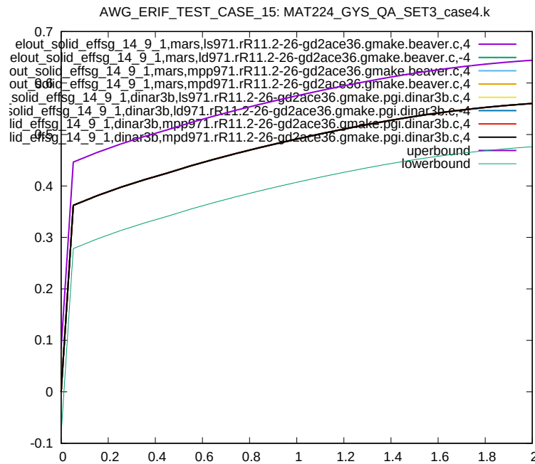
Figure 103: Cross platform results, Von Mises Stress, element ID 14, sub test case ID 6
