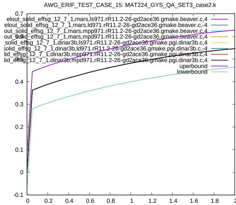
Figure 82: Cross platform results, Von Mises Stress, element ID 12, sub test case ID 4
