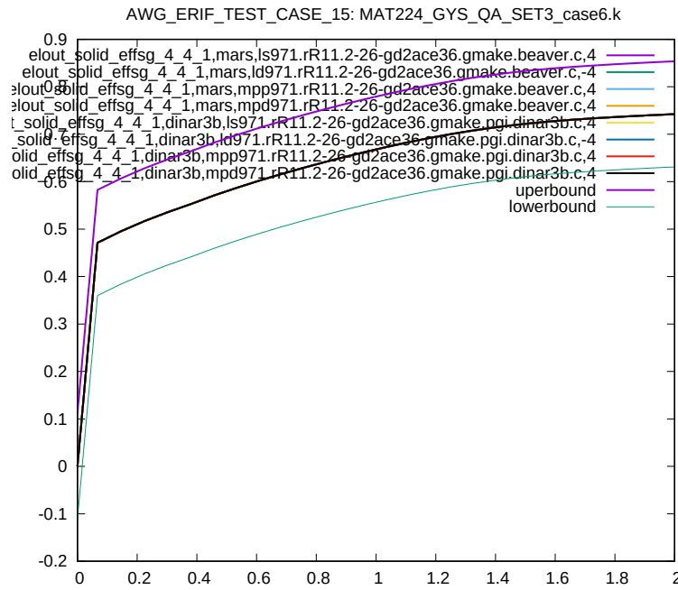
Figure 124: Cross platform results, Von Mises Stress, element ID 4, sub test case ID 8
