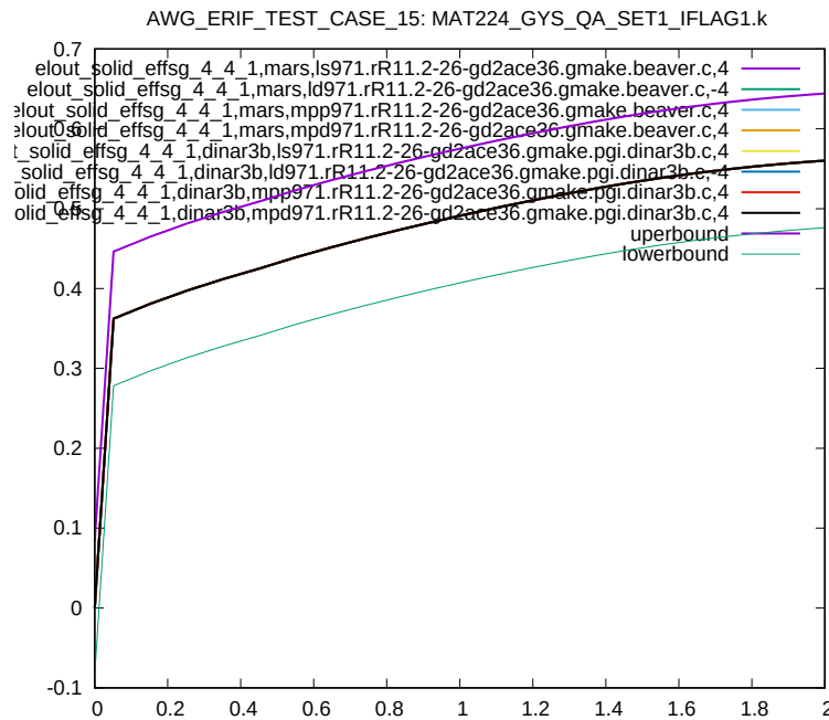
Figure 37: Cross platform results, Von Mises Stress, element ID 4, sub test case ID 2
