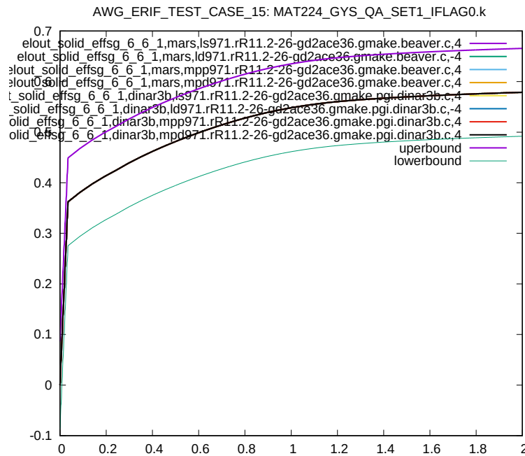
Figure 19: Cross platform results, Von Mises Stress, element ID 6, sub test case ID 1
