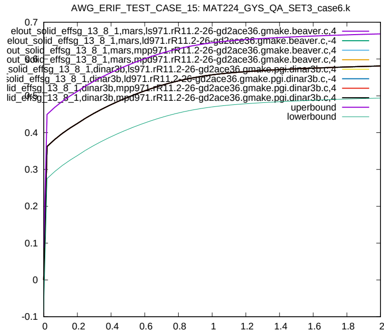
Figure 126: Cross platform results, Von Mises Stress, element ID 13, sub test case ID 8
