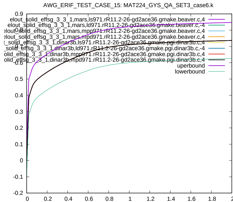
Figure 123: Cross platform results, Von Mises Stress, element ID 3, sub test case ID 8
