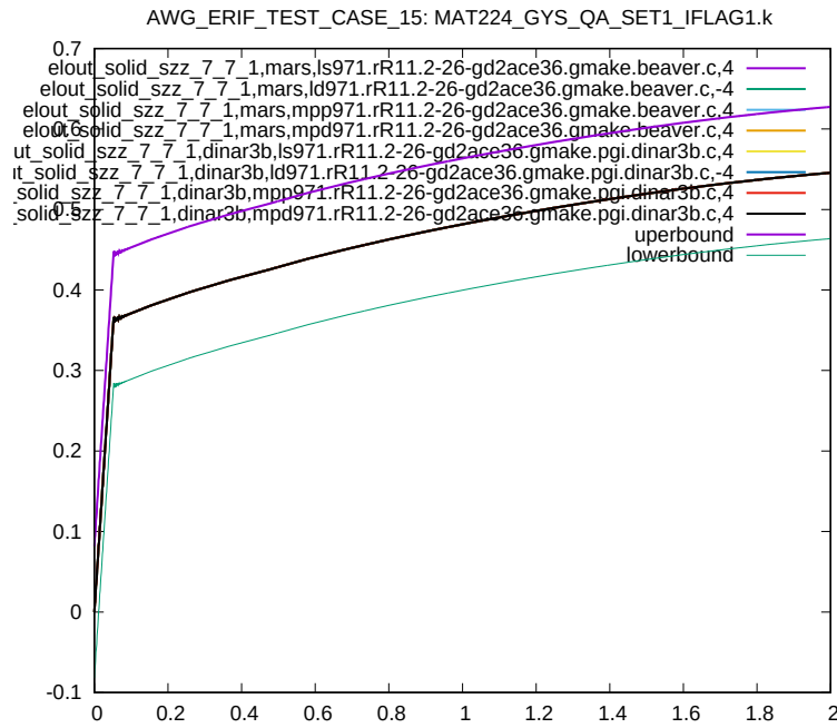
Figure 30: Cross platform results, z-component Stress, element ID 7, sub test case ID 2
