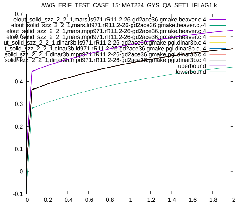
Figure 25: Cross platform results, z-component Stress, element ID 2, sub test case ID 2
