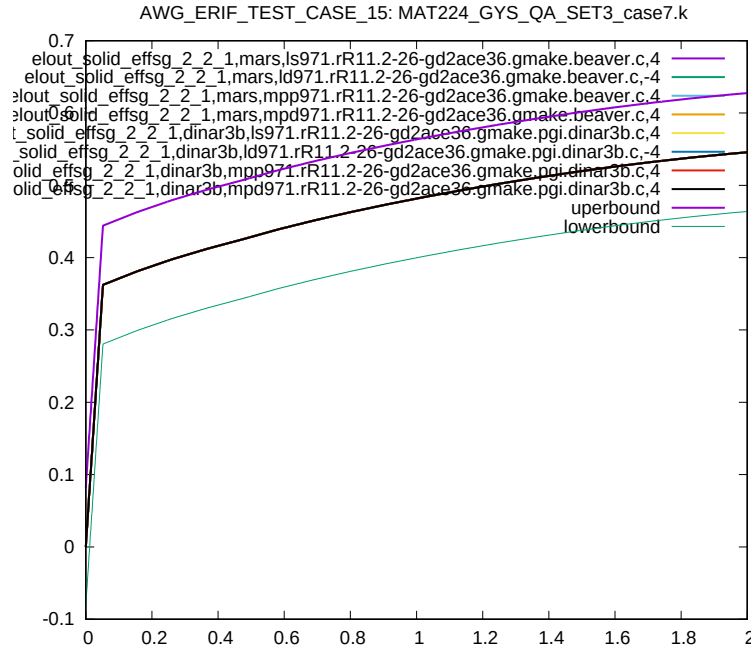
Figure 134: Cross platform results, Von Mises Stress, element ID 2, sub test case ID 9
