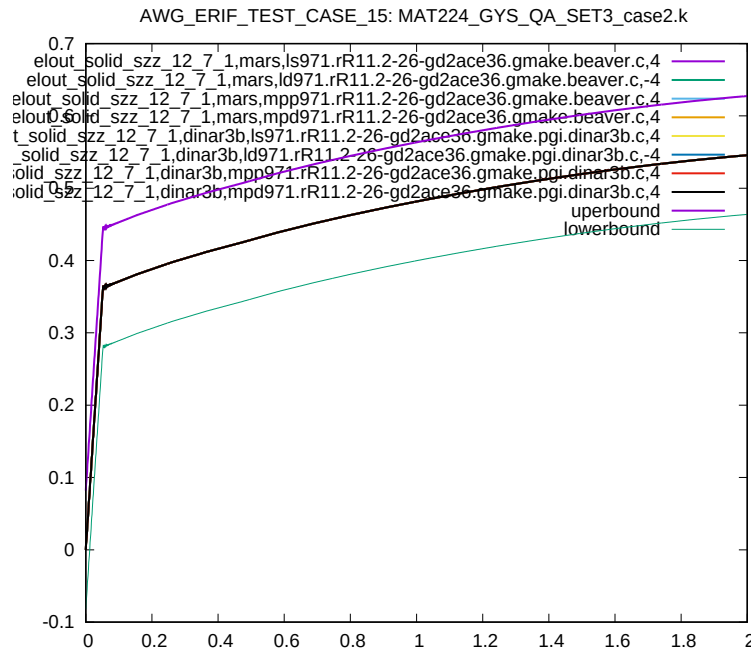
Figure 78: Cross platform results, z-component Stress, element ID 12, sub test case ID 4
