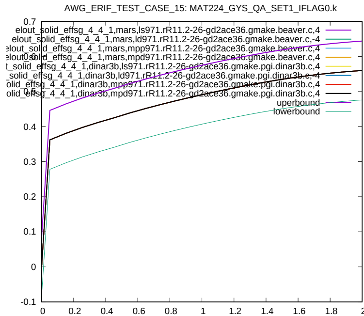
Figure 17: Cross platform results, Von Mises Stress, element ID 4, sub test case ID 1
