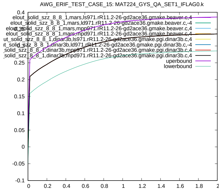
Figure 11: Cross platform results, z-component Stress, element ID 8, sub test case ID 1
