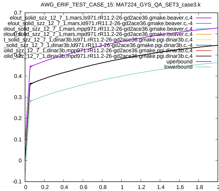
Figure 86: Cross platform results, z-component Stress, element ID 12, sub test case ID 5
