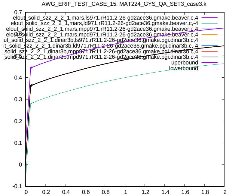
Figure 84: Cross platform results, z-component Stress, element ID 2, sub test case ID 5
