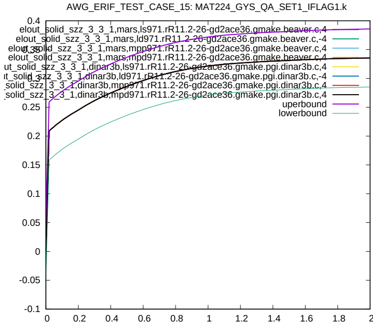
Figure 26: Cross platform results, z-component Stress, element ID 3, sub test case ID 2
