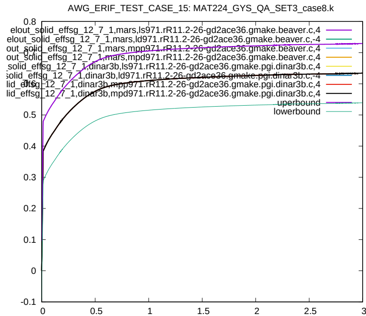
Figure 149: Cross platform results, Von Mises Stress, element ID 12, sub test case ID 10
