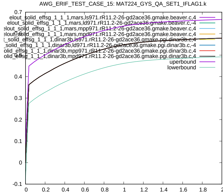
Figure 34: Cross platform results, Von Mises Stress, element ID 1, sub test case ID 2
