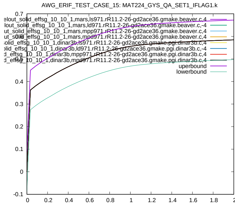
Figure 43: Cross platform results, Von Mises Stress, element ID 10, sub test case ID 2
