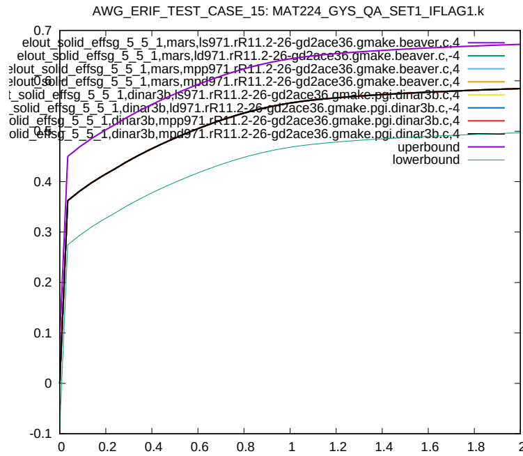
Figure 38: Cross platform results, Von Mises Stress, element ID 5, sub test case ID 2
