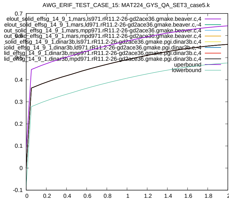
Figure 115: Cross platform results, Von Mises Stress, element ID 14, sub test case ID 7
