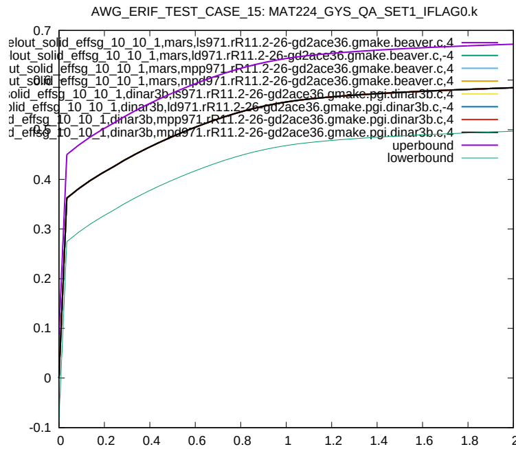
Figure 23: Cross platform results, Von Mises Stress, element ID 10, sub test case ID 1
