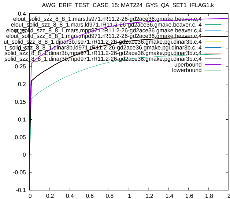
Figure 31: Cross platform results, z-component Stress, element ID 8, sub test case ID 2
