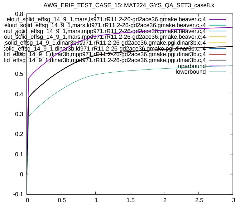
Figure 151: Cross platform results, Von Mises Stress, element ID 14, sub test case ID 10
