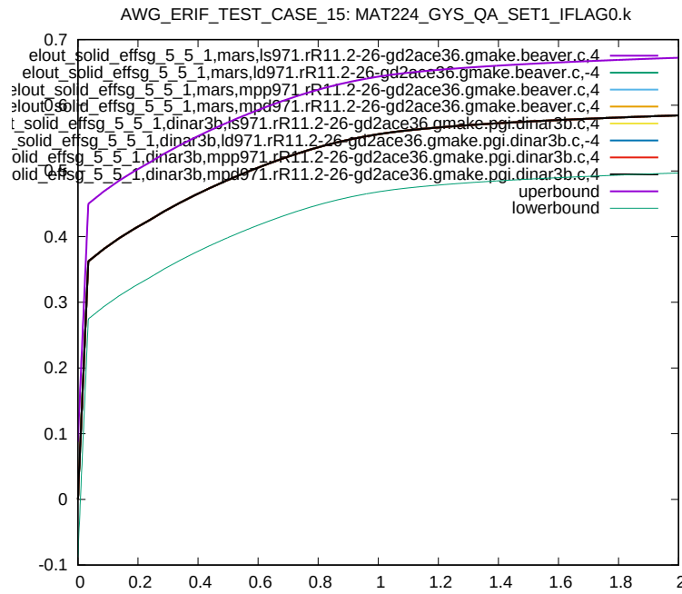
Figure 18: Cross platform results, Von Mises Stress, element ID 5, sub test case ID 1
