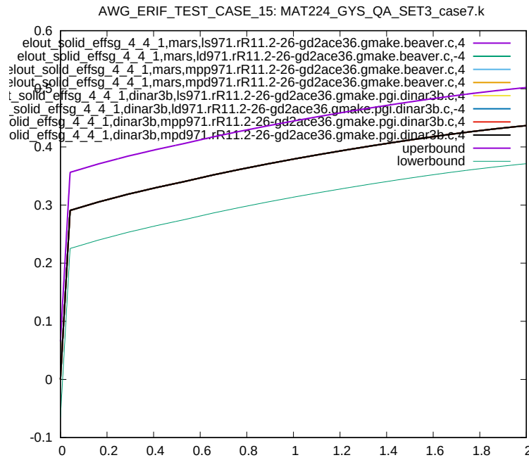
Figure 136: Cross platform results, Von Mises Stress, element ID 4, sub test case ID 9
