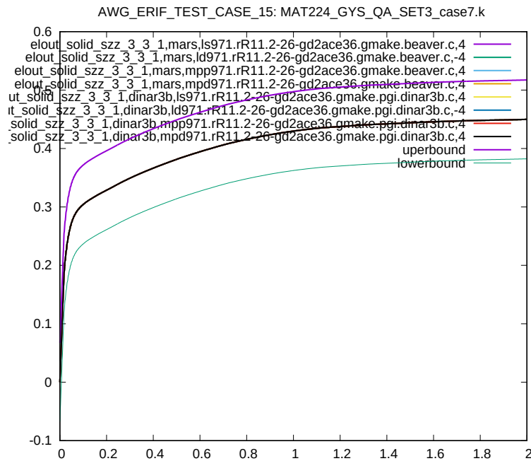
Figure 129: Cross platform results, z-component Stress, element ID 3, sub test case ID 9
