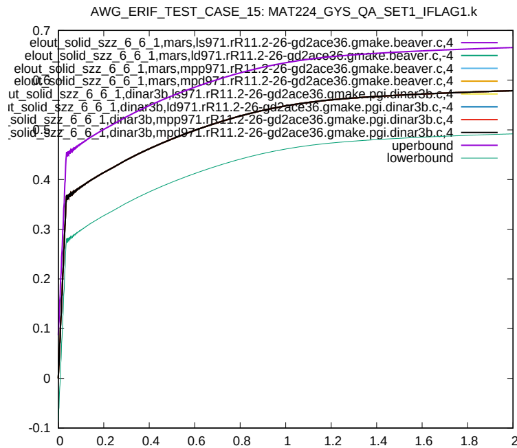
Figure 29: Cross platform results, z-component Stress, element ID 6, sub test case ID 2
