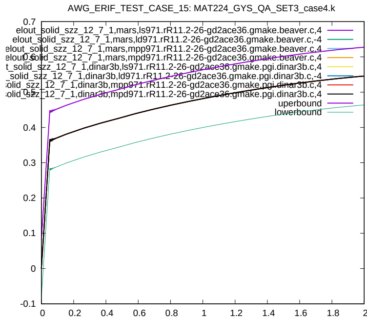
Figure 95: Cross platform results, z-component Stress, element ID 12, sub test case ID 6
