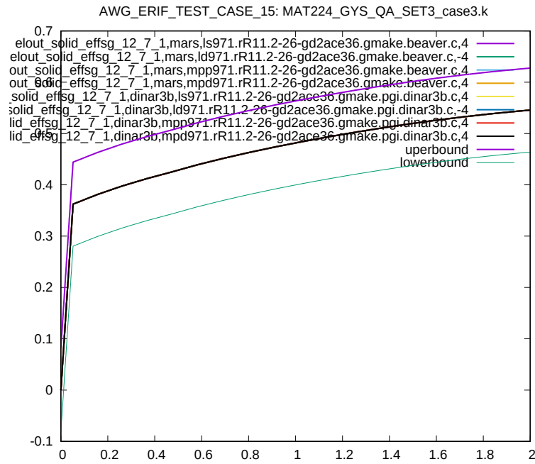
Figure 90: Cross platform results, Von Mises Stress, element ID 12, sub test case ID 5
