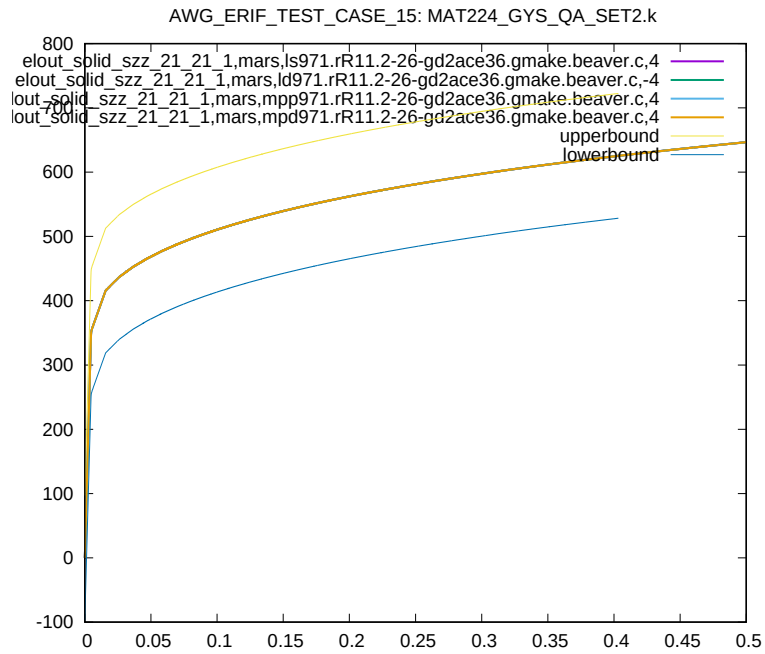
Figure 56: Cross platform results, z-component Stress, element ID 21, sub test case ID 3
