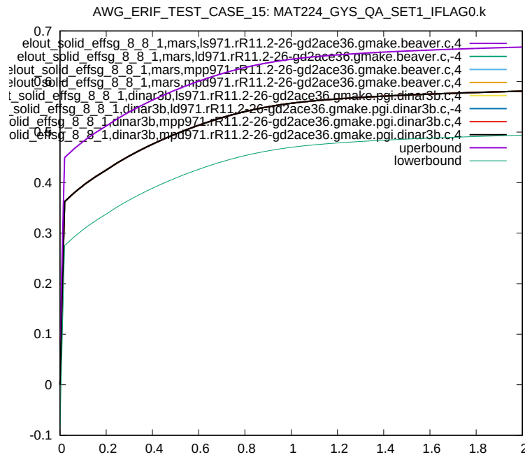
Figure 21: Cross platform results, Von Mises Stress, element ID 8, sub test case ID 1
