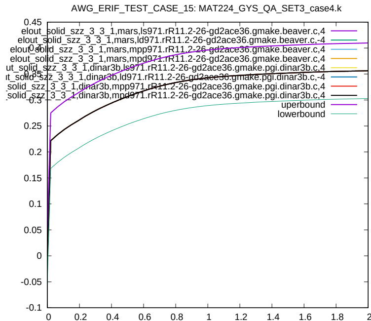
Figure 93: Cross platform results, z-component Stress, element ID 3, sub test case ID 6
