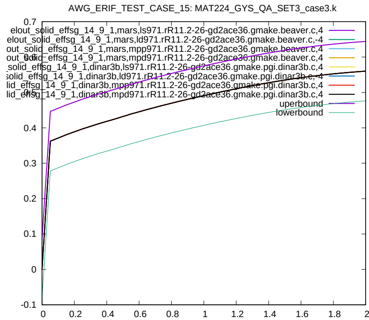
Figure 91: Cross platform results, Von Mises Stress, element ID 14, sub test case ID 5
