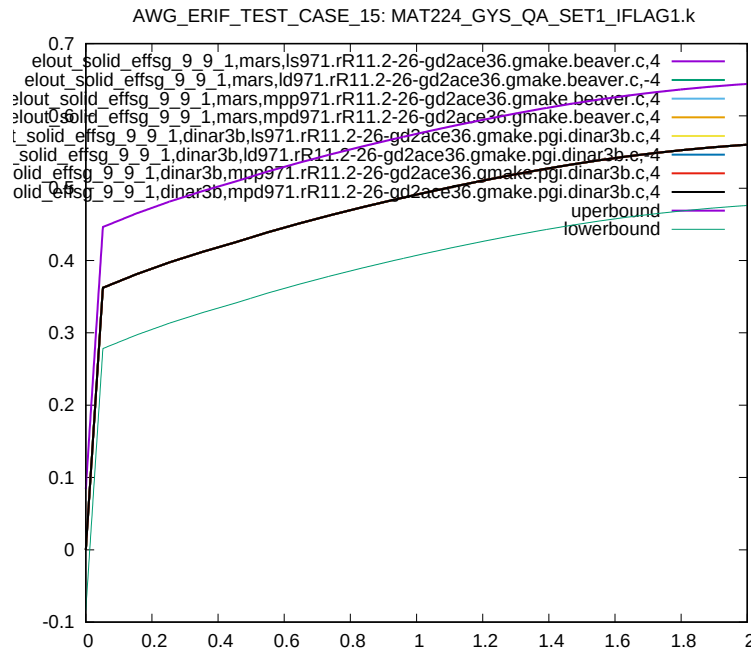
Figure 42: Cross platform results, Von Mises Stress, element ID 9, sub test case ID 2
