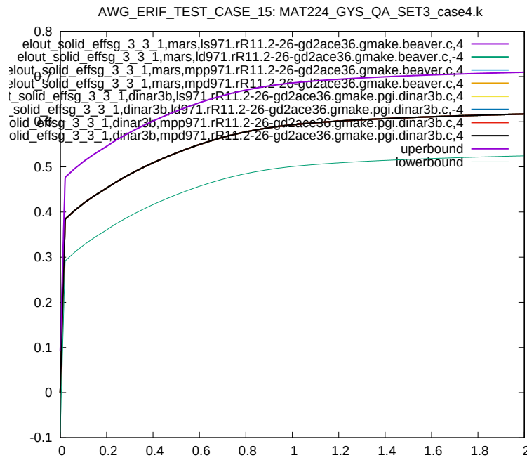
Figure 99: Cross platform results, Von Mises Stress, element ID 3, sub test case ID 6
