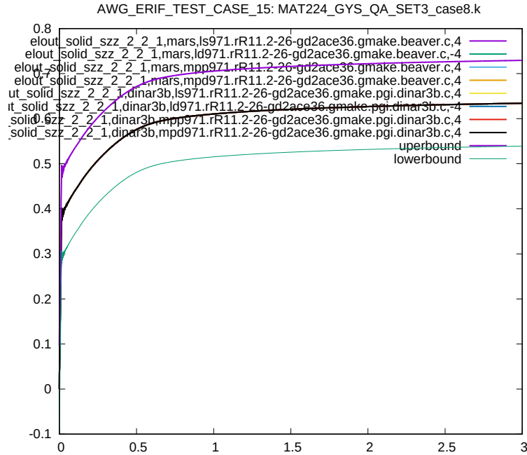
Figure 140: Cross platform results, z-component Stress, element ID 2, sub test case ID 10
