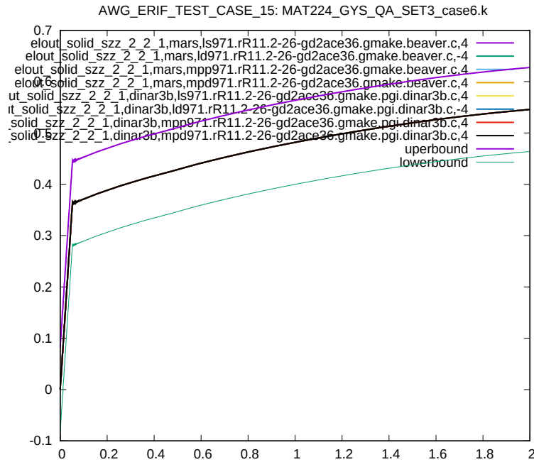
Figure 116: Cross platform results, z-component Stress, element ID 2, sub test case ID 8
