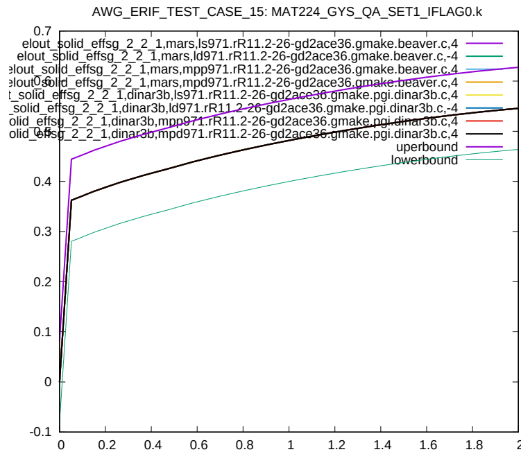
Figure 15: Cross platform results, Von Mises Stress, element ID 2, sub test case ID 1
