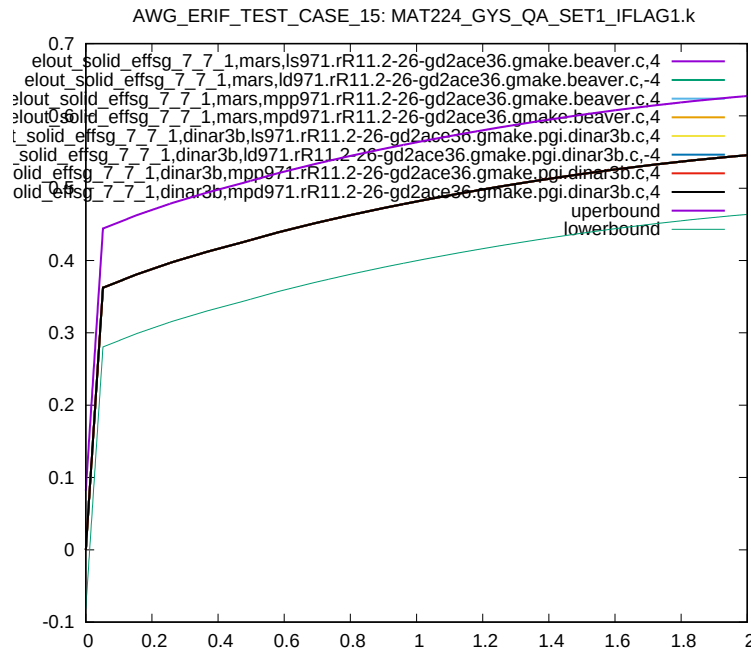
Figure 40: Cross platform results, Von Mises Stress, element ID 7, sub test case ID 2
