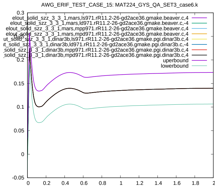
Figure 117: Cross platform results, z-component Stress, element ID 3, sub test case ID 8
