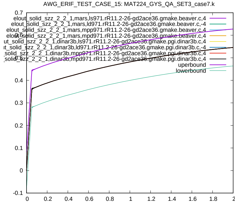
Figure 128: Cross platform results, z-component Stress, element ID 2, sub test case ID 9
