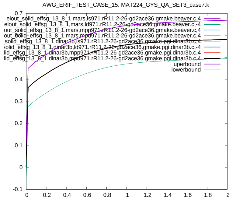
Figure 138: Cross platform results, Von Mises Stress, element ID 13, sub test case ID 9
