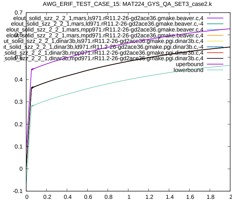
Figure 76: Cross platform results, z-component Stress, element ID 2, sub test case ID 4
