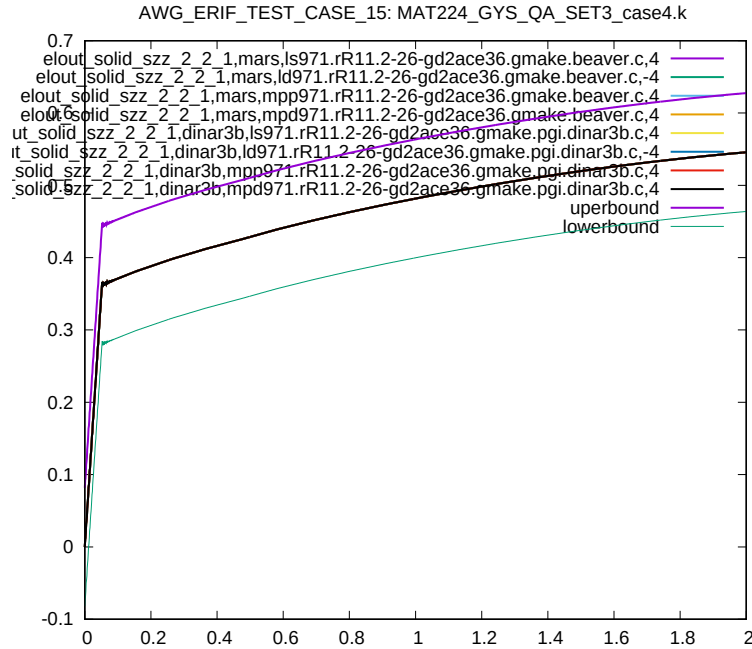
Figure 92: Cross platform results, z-component Stress, element ID 2, sub test case ID 6
