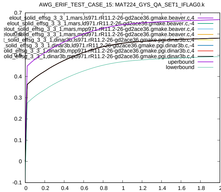
Figure 16: Cross platform results, Von Mises Stress, element ID 3, sub test case ID 1
