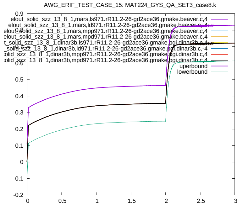
Figure 144: Cross platform results, z-component Stress, element ID 13, sub test case ID 10
