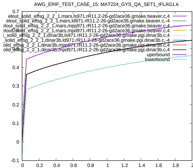
Figure 35: Cross platform results, Von Mises Stress, element ID 2, sub test case ID 2
