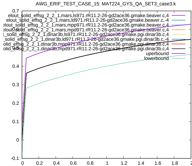
Figure 88: Cross platform results, Von Mises Stress, element ID 2, sub test case ID 5
