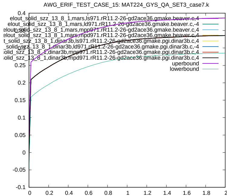
Figure 132: Cross platform results, z-component Stress, element ID 13, sub test case ID 9
