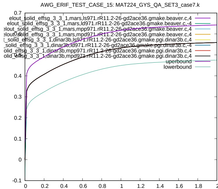
Figure 135: Cross platform results, Von Mises Stress, element ID 3, sub test case ID 9
