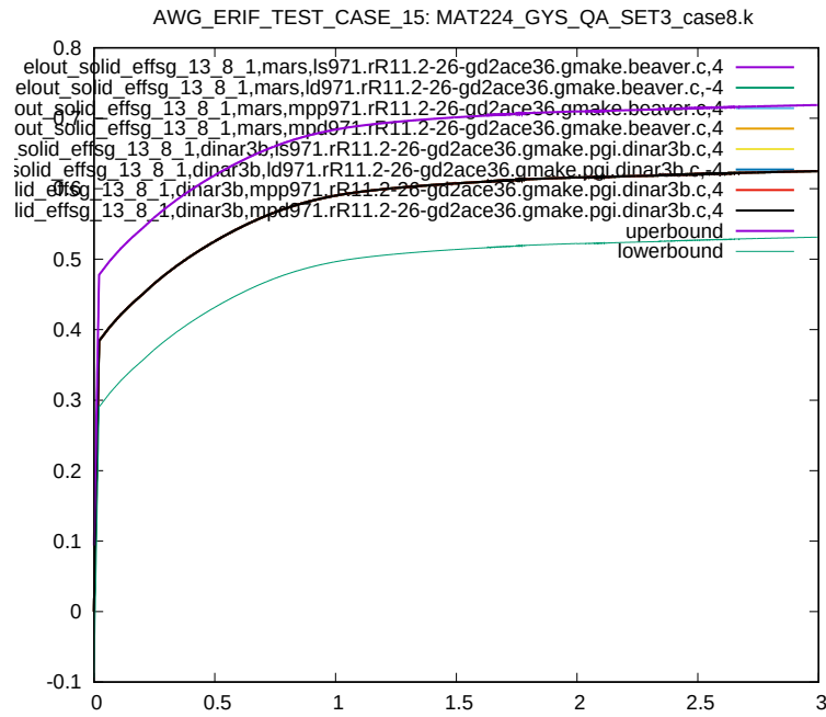
Figure 150: Cross platform results, Von Mises Stress, element ID 13, sub test case ID 10
