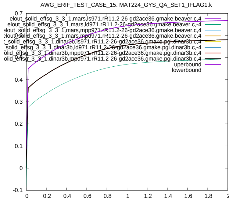
Figure 36: Cross platform results, Von Mises Stress, element ID 3, sub test case ID 2
