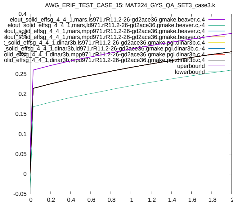
Figure 89: Cross platform results, Von Mises Stress, element ID 4, sub test case ID 5
