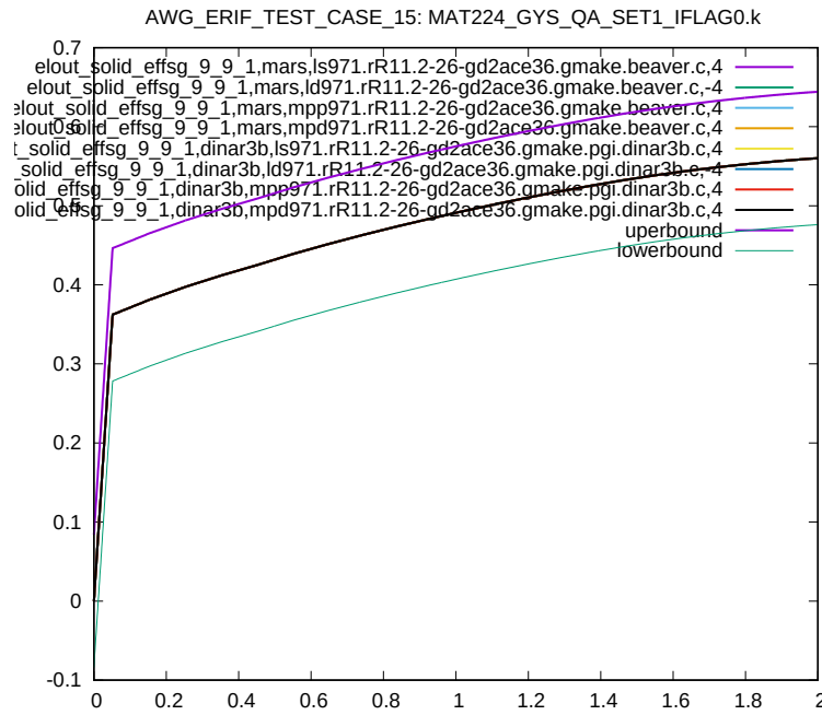
Figure 22: Cross platform results, Von Mises Stress, element ID 9, sub test case ID 1
