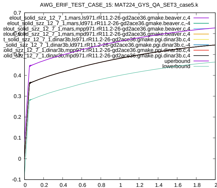
Figure 107: Cross platform results, z-component Stress, element ID 12, sub test case ID 7
