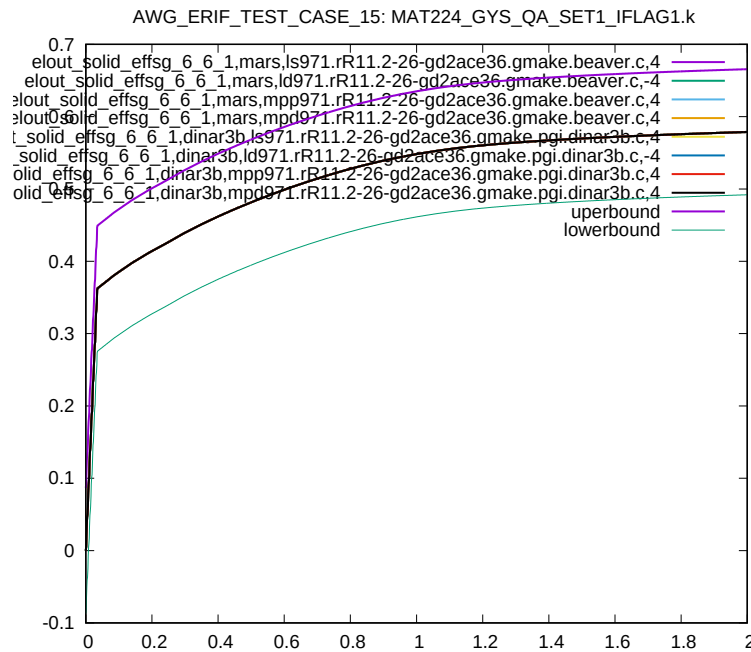
Figure 39: Cross platform results, Von Mises Stress, element ID 6, sub test case ID 2
