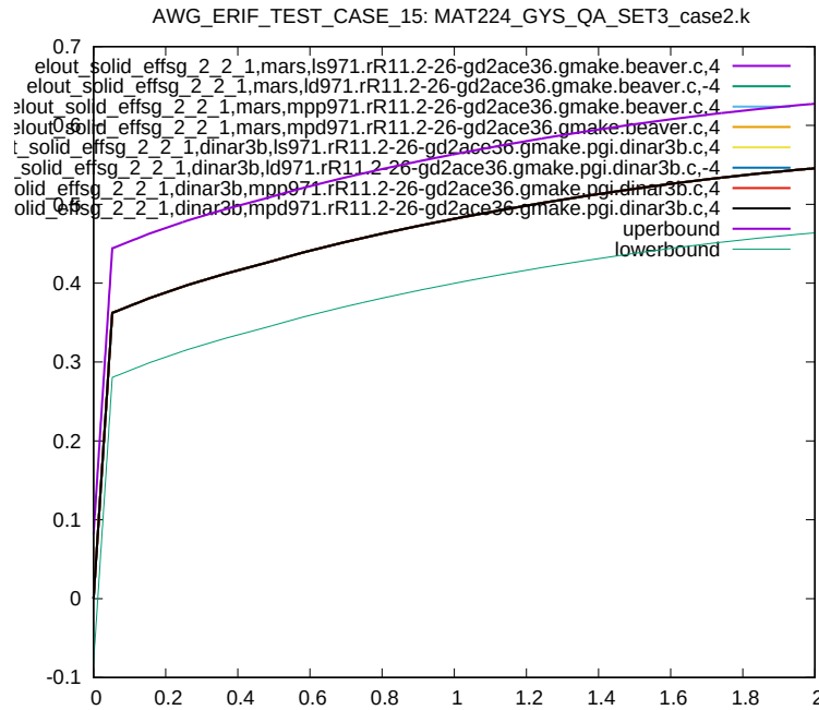
Figure 80: Cross platform results, Von Mises Stress, element ID 2, sub test case ID 4
