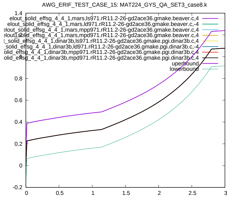
Figure 148: Cross platform results, Von Mises Stress, element ID 4, sub test case ID 10
