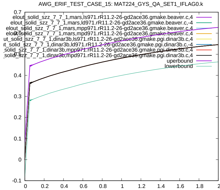
Figure 10: Cross platform results, z-component Stress, element ID 7, sub test case ID 1
