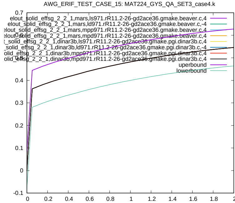
Figure 98: Cross platform results, Von Mises Stress, element ID 2, sub test case ID 6
