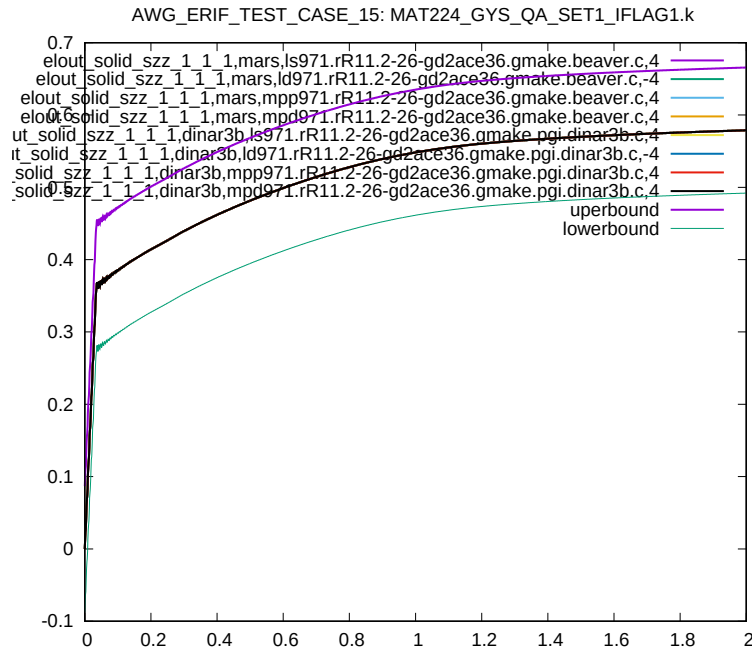
Figure 24: Cross platform results, z-component Stress, element ID 1, sub test case ID 2
