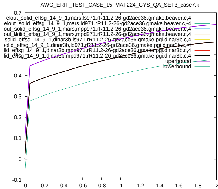
Figure 139: Cross platform results, Von Mises Stress, element ID 14, sub test case ID 9
