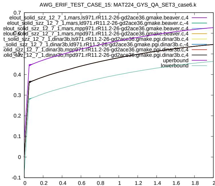
Figure 119: Cross platform results, z-component Stress, element ID 12, sub test case ID 8
