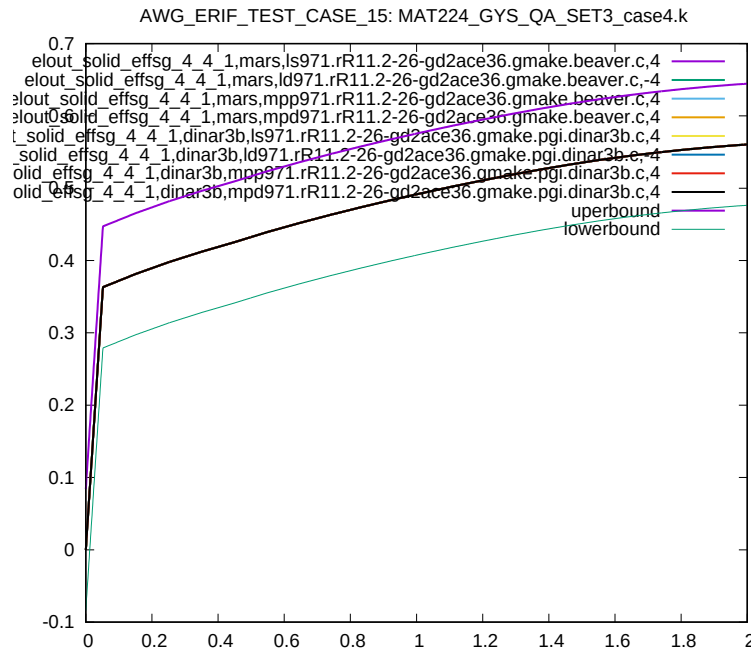
Figure 100: Cross platform results, Von Mises Stress, element ID 4, sub test case ID 6
