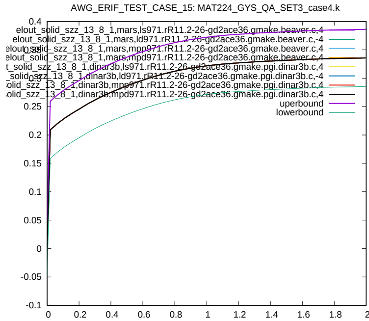
Figure 96: Cross platform results, z-component Stress, element ID 13, sub test case ID 6
