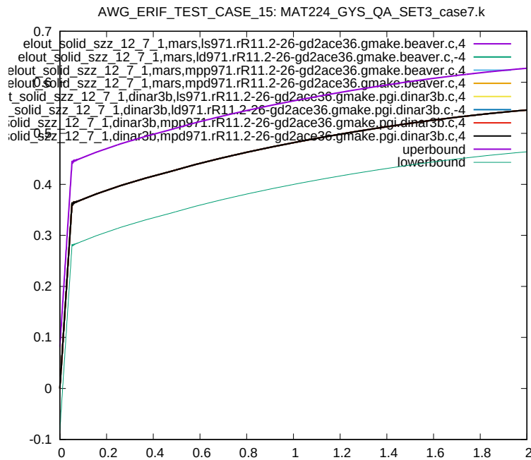
Figure 131: Cross platform results, z-component Stress, element ID 12, sub test case ID 9
