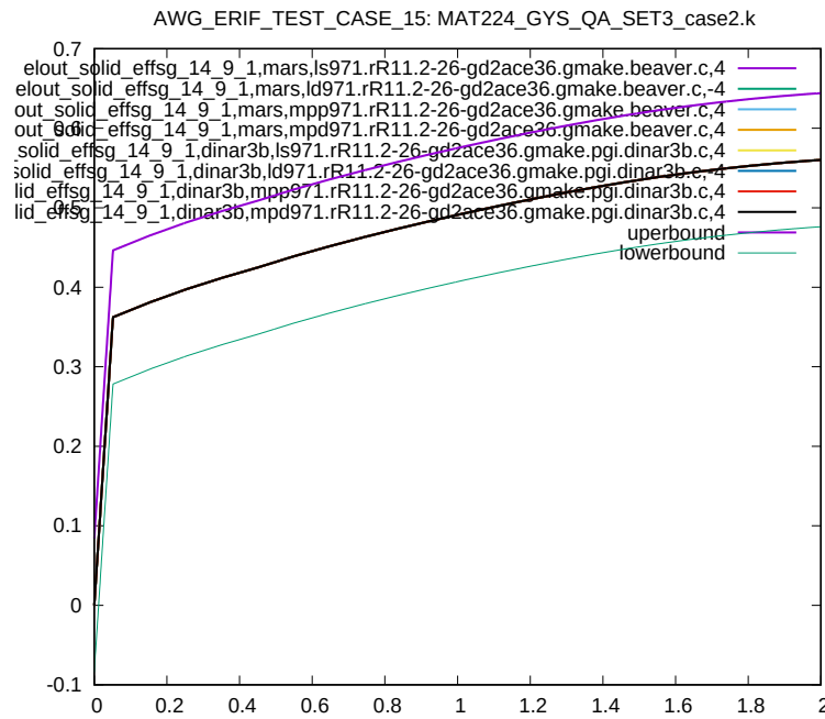
Figure 83: Cross platform results, Von Mises Stress, element ID 14, sub test case ID 4
