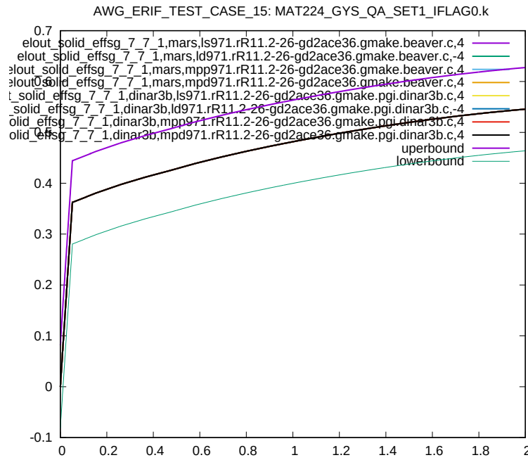
Figure 20: Cross platform results, Von Mises Stress, element ID 7, sub test case ID 1
