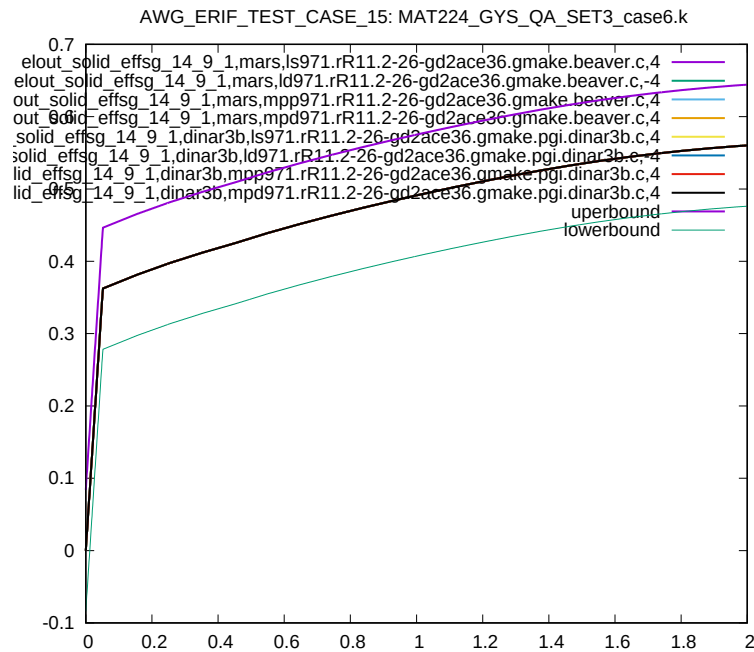
Figure 127: Cross platform results, Von Mises Stress, element ID 14, sub test case ID 8
