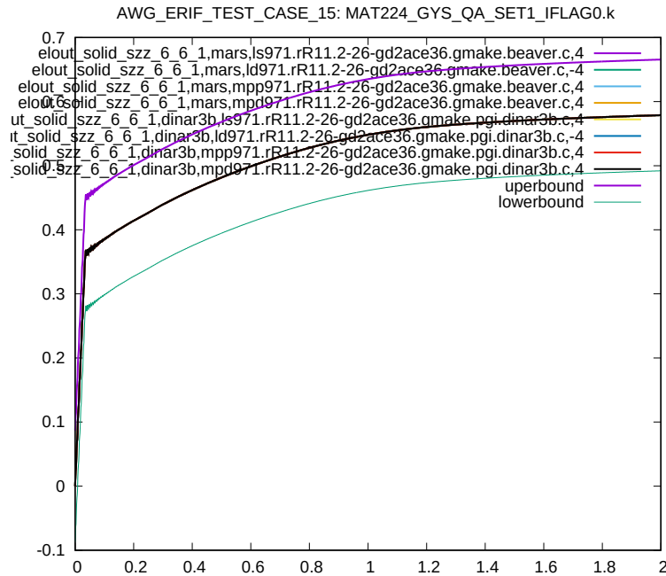
Figure 9: Cross platform results, z-component Stress, element ID 6, sub test case ID 1
