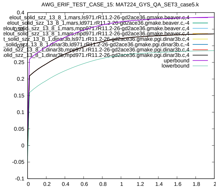
Figure 108: Cross platform results, z-component Stress, element ID 13, sub test case ID 7
