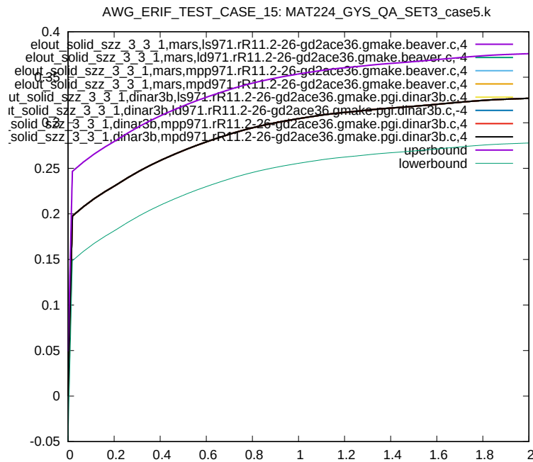
Figure 105: Cross platform results, z-component Stress, element ID 3, sub test case ID 7
