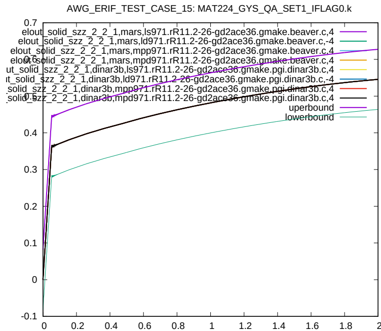
Figure 5: Cross platform results, z-component Stress, element ID 2, sub test case ID 1
