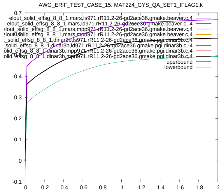
Figure 41: Cross platform results, Von Mises Stress, element ID 8, sub test case ID 2
