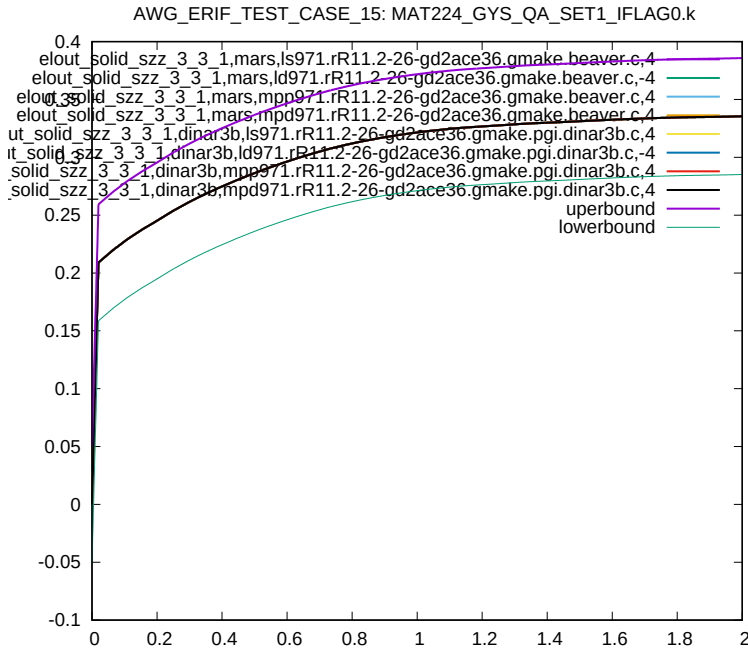
Figure 6: Cross platform results, z-component Stress, element ID 3, sub test case ID 1
