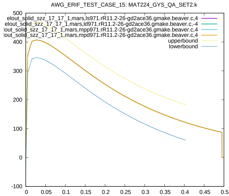
Figure 52: Cross platform results, z-component Stress, element ID 17, sub test case ID 3
