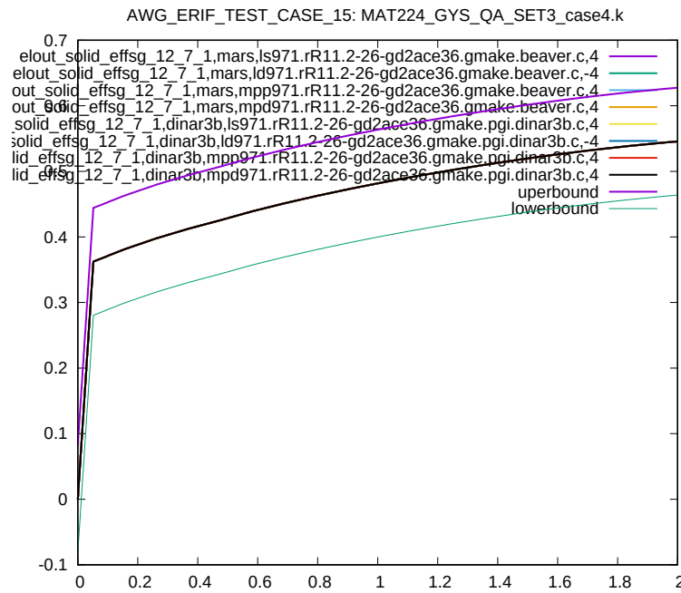
Figure 101: Cross platform results, Von Mises Stress, element ID 12, sub test case ID 6
