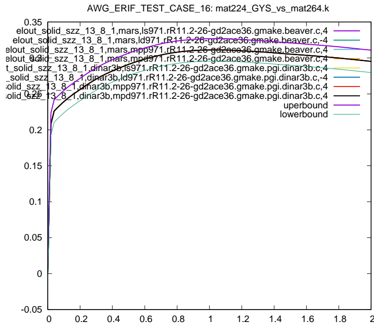
Figure 9: Cross platform results, z-component Stress, element ID 13, sub test case ID 1
