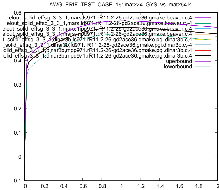
Figure 14: Cross platform results, Von Mises Stress, element ID 3, sub test case ID 1
