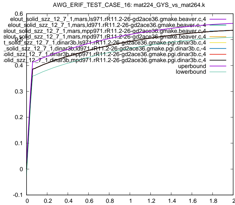
Figure 8: Cross platform results, z-component Stress, element ID 12, sub test case ID 1
