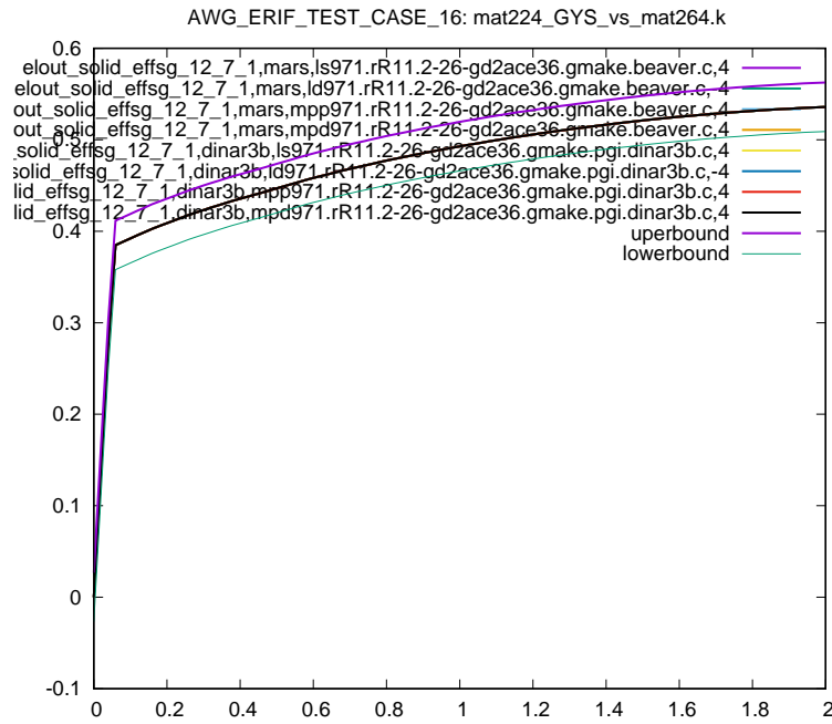
Figure 18: Cross platform results, Von Mises Stress, element ID 12, sub test case ID 1
