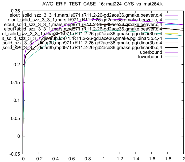
Figure 4: Cross platform results, z-component Stress, element ID 3, sub test case ID 1
