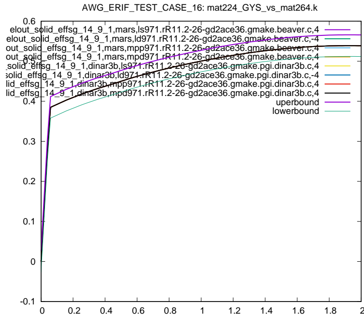
Figure 20: Cross platform results, Von Mises Stress, element ID 14, sub test case ID 1
