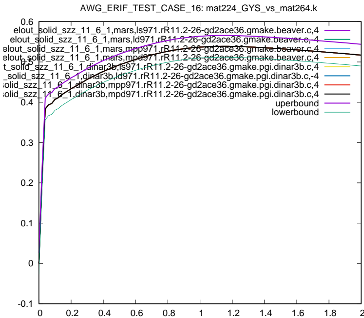
Figure 7: Cross platform results, z-component Stress, element ID 11, sub test case ID 1
