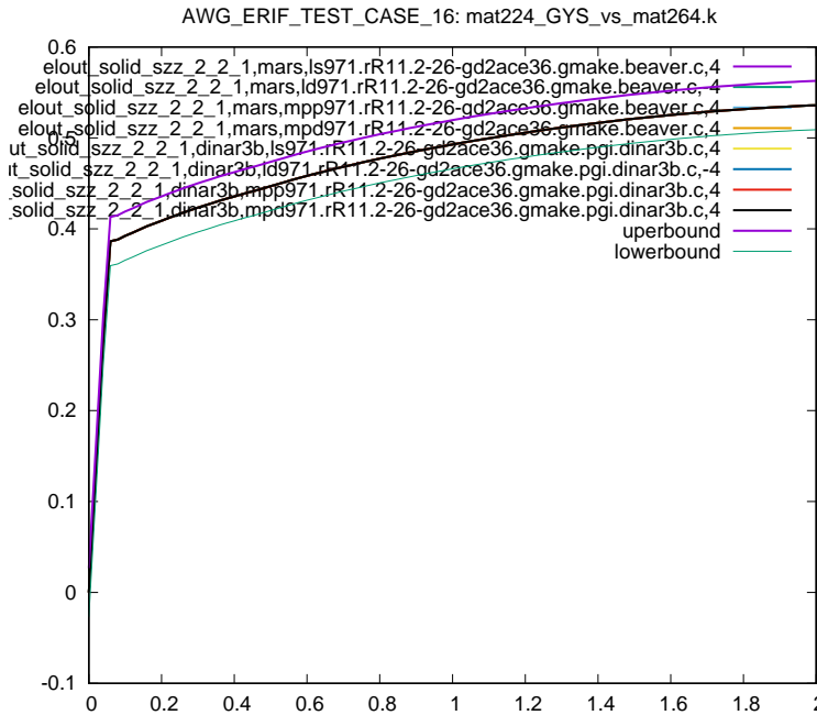
Figure 3: Cross platform results, z-component Stress, element ID 2, sub test case ID 1
