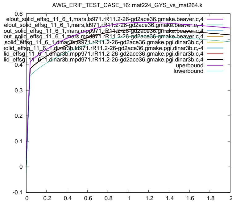
Figure 17: Cross platform results, Von Mises Stress, element ID 11, sub test case ID 1
