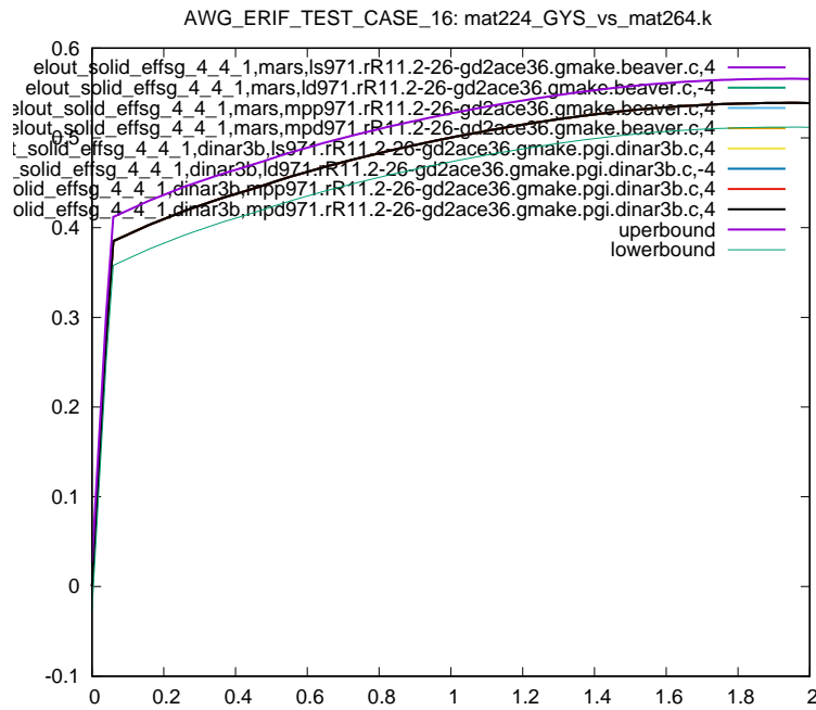
Figure 15: Cross platform results, Von Mises Stress, element ID 4, sub test case ID 1
