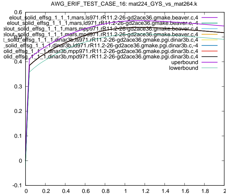
Figure 12: Cross platform results, Von Mises Stress, element ID 1, sub test case ID 1
