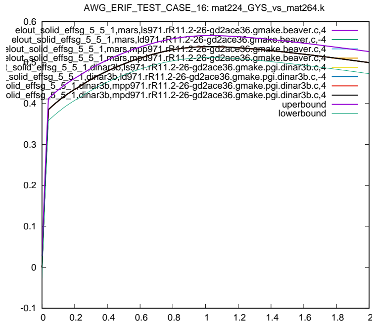
Figure 16: Cross platform results, Von Mises Stress, element ID 5, sub test case ID 1
