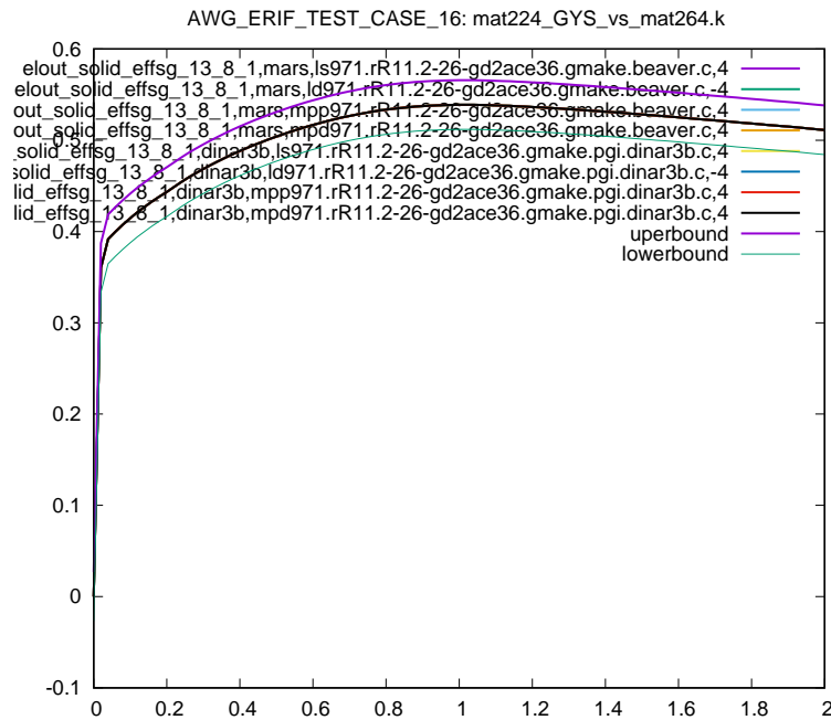
Figure 19: Cross platform results, Von Mises Stress, element ID 13, sub test case ID 1
