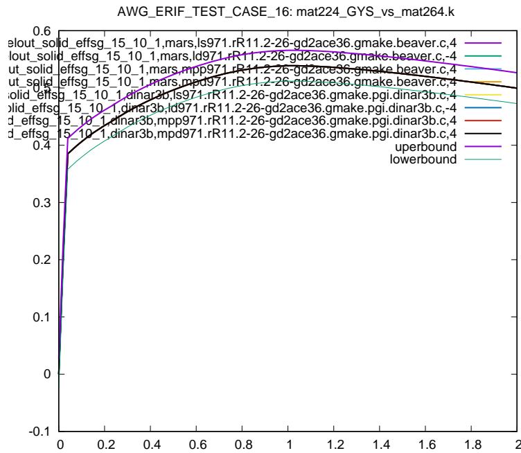
Figure 21: Cross platform results, Von Mises Stress, element ID 10, sub test case ID 1
