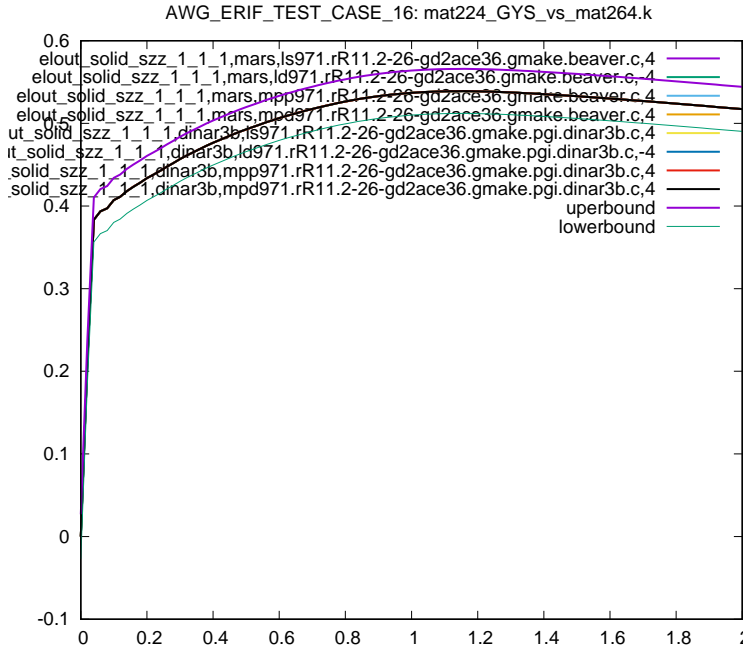
Figure 2: Cross platform results, z-component Stress, element ID 1, sub test case ID 1
