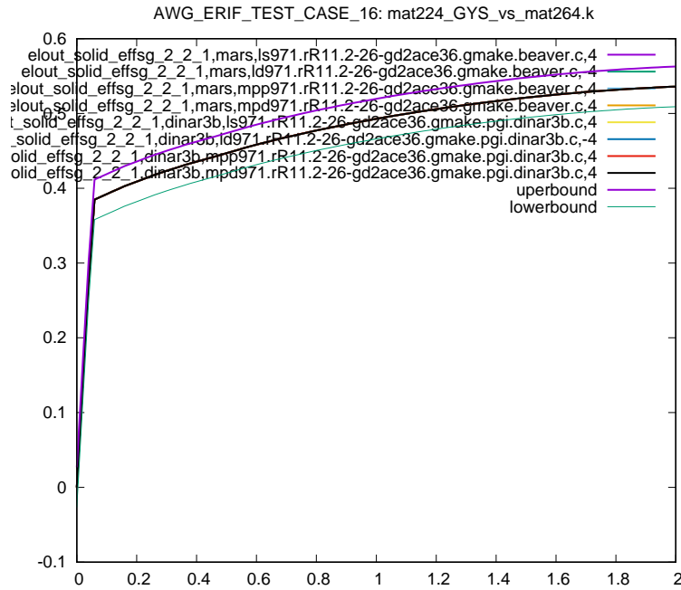
Figure 13: Cross platform results, Von Mises Stress, element ID 2, sub test case ID 1
