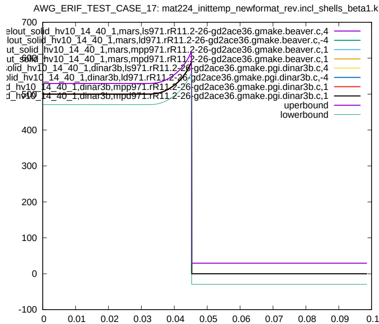
Figure 13: Cross platform results, History Variable 10 (temperature), element ID 14, sub test case ID 2
