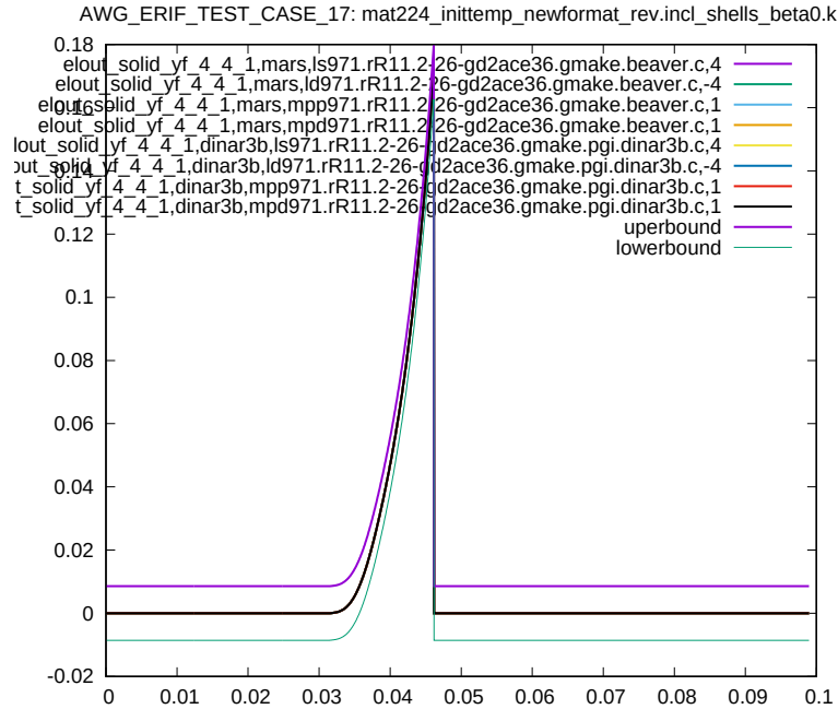
Figure 4: Cross platform results, Effective Plastic Strain, element ID 4, sub test case ID 1
