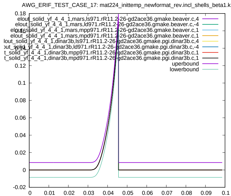
Figure 5: Cross platform results, Effective Plastic Strain, element ID 4, sub test case ID 2
