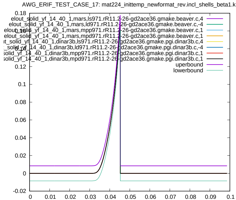
Figure 11: Cross platform results, Effective Plastic Strain, element ID 14, sub test case ID 2
