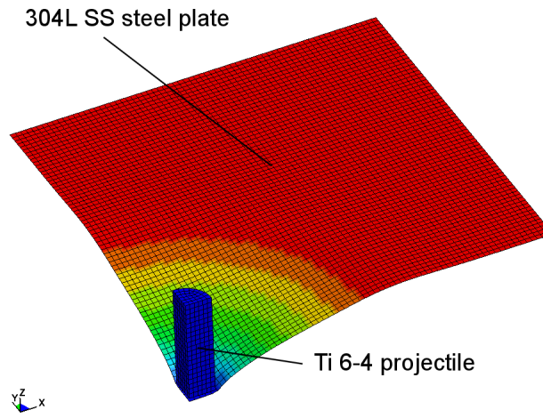
Figure 3: FEA model: Ballistic Impact - Ti 6-4 Projectile impacts a 304L SS plate
