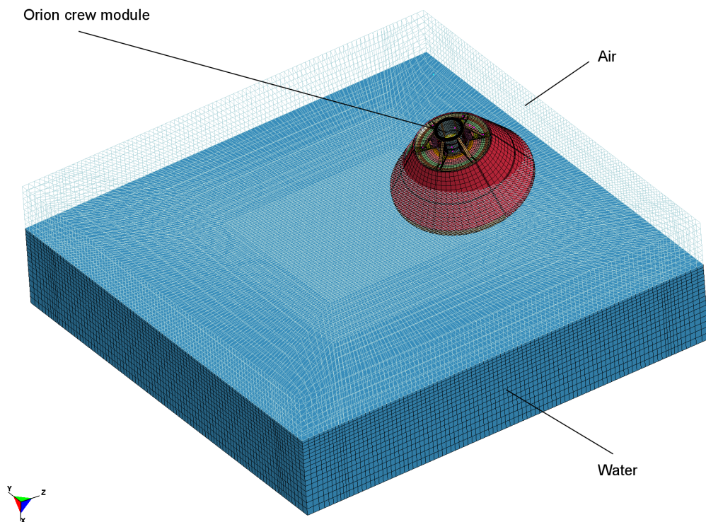
Figure 2: FEA model: Orion crew module water landing
