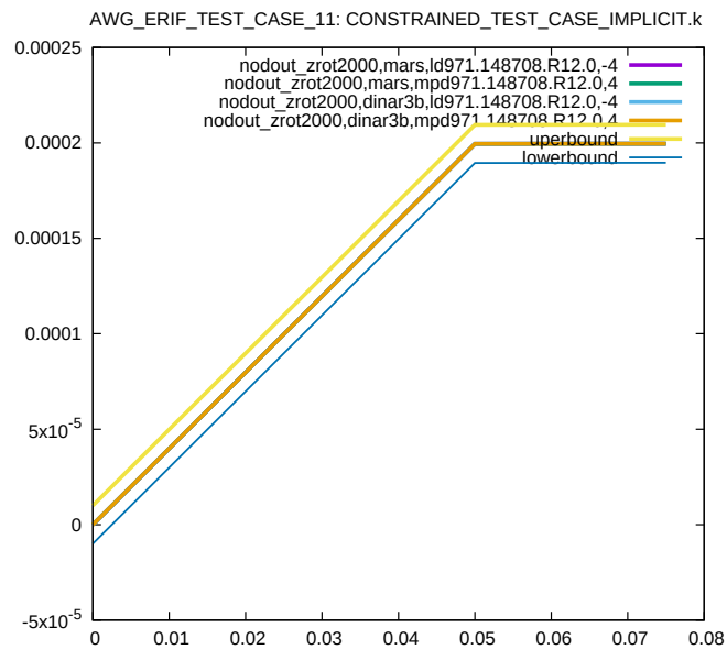
Figure 26: Cross platform results, nodal rotation around z-axis, node 2000, sub test case ID 2
