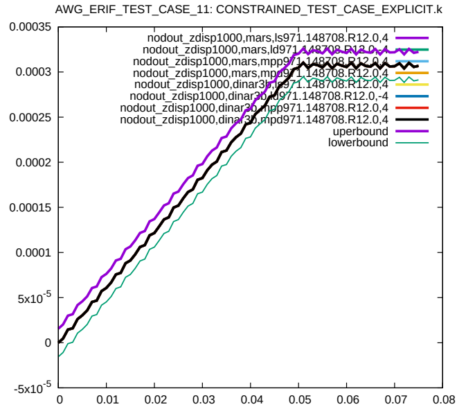
Figure 5: Cross platform results, nodal displacement in z-direction, node 1000, sub test case ID 1
