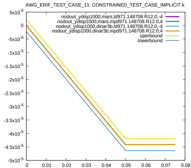
Figure 16: Cross platform results, nodal displacement in y-direction, node 1000, sub test case ID 2
