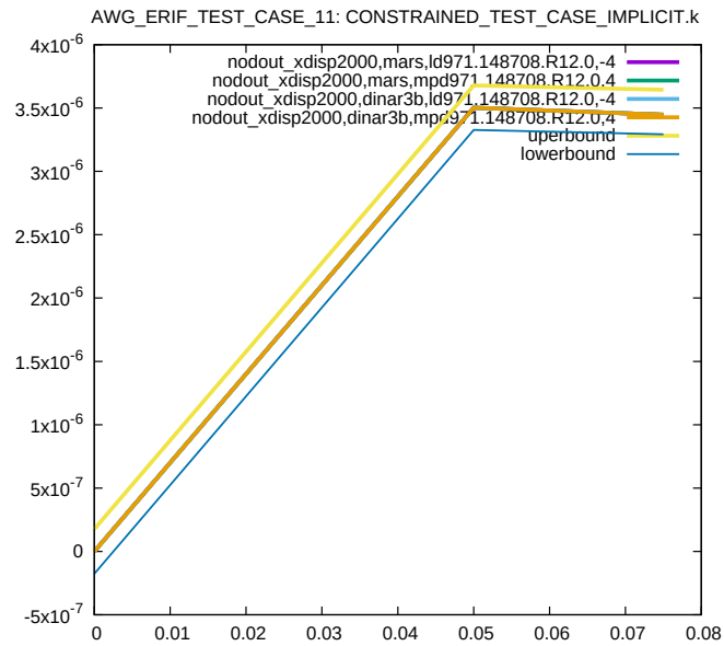
Figure 21: Cross platform results, nodal displacement in x-direction, node 2000, sub test case ID 2
