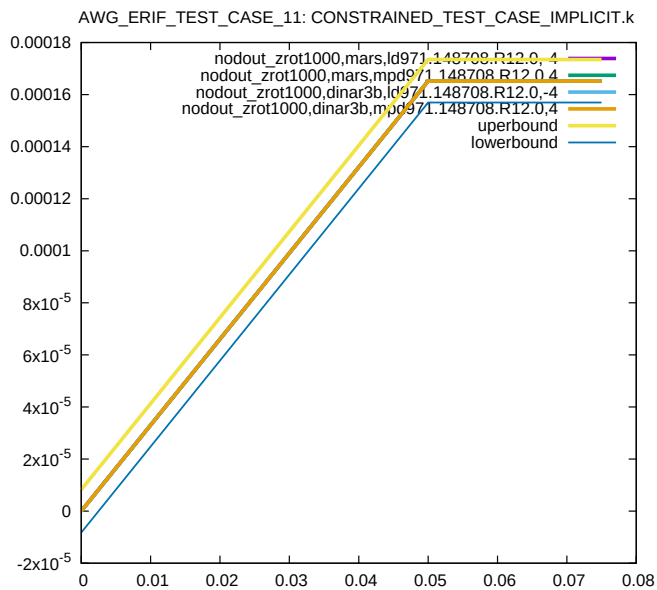
Figure 20: Cross platform results, nodal rotation around z-axis, node 1000, sub test case ID 2
