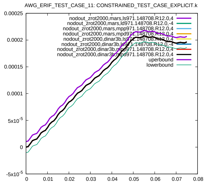
Figure 14: Cross platform results, nodal rotation around z-axis, node 2000, sub test case ID 1
