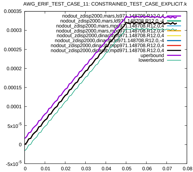
Figure 11: Cross platform results, nodal displacement in z-direction, node 2000, sub test case ID 1
