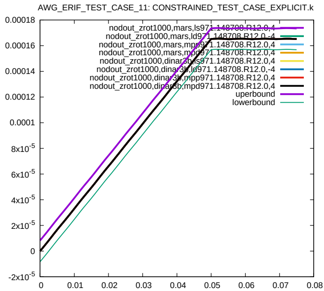
Figure 8: Cross platform results, nodal rotation around z-axis, node 1000, sub test case ID 1
