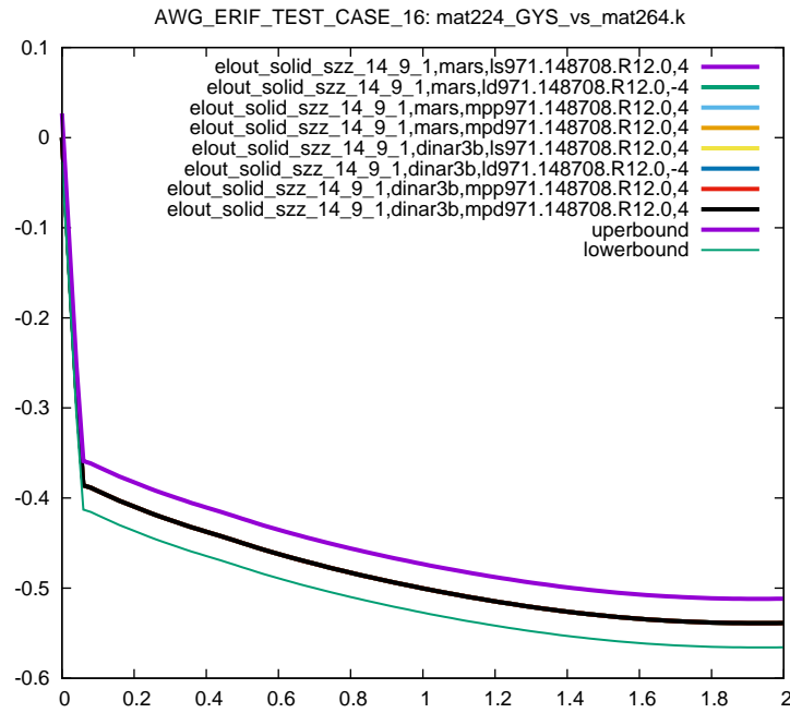
Figure 10: Cross platform results, z-component Stress, element ID 14, sub test case ID 1
