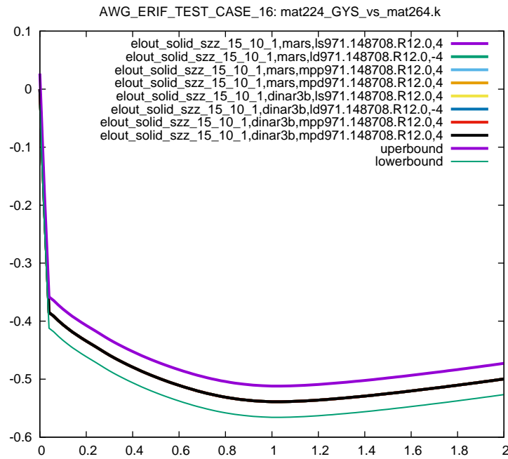
Figure 11: Cross platform results, z-component Stress, element ID 10, sub test case ID 1
