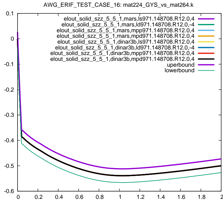
Figure 6: Cross platform results, z-component Stress, element ID 5, sub test case ID 1
