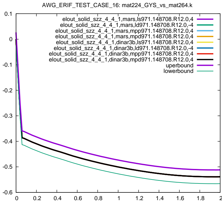
Figure 5: Cross platform results, z-component Stress, element ID 4, sub test case ID 1
