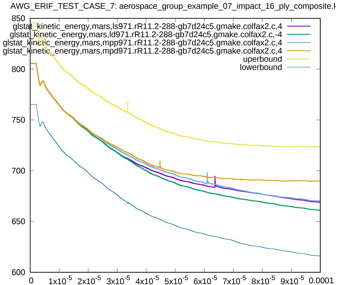
Figure 4: Cross platform results, global kinetic energy, sub test case ID 1
