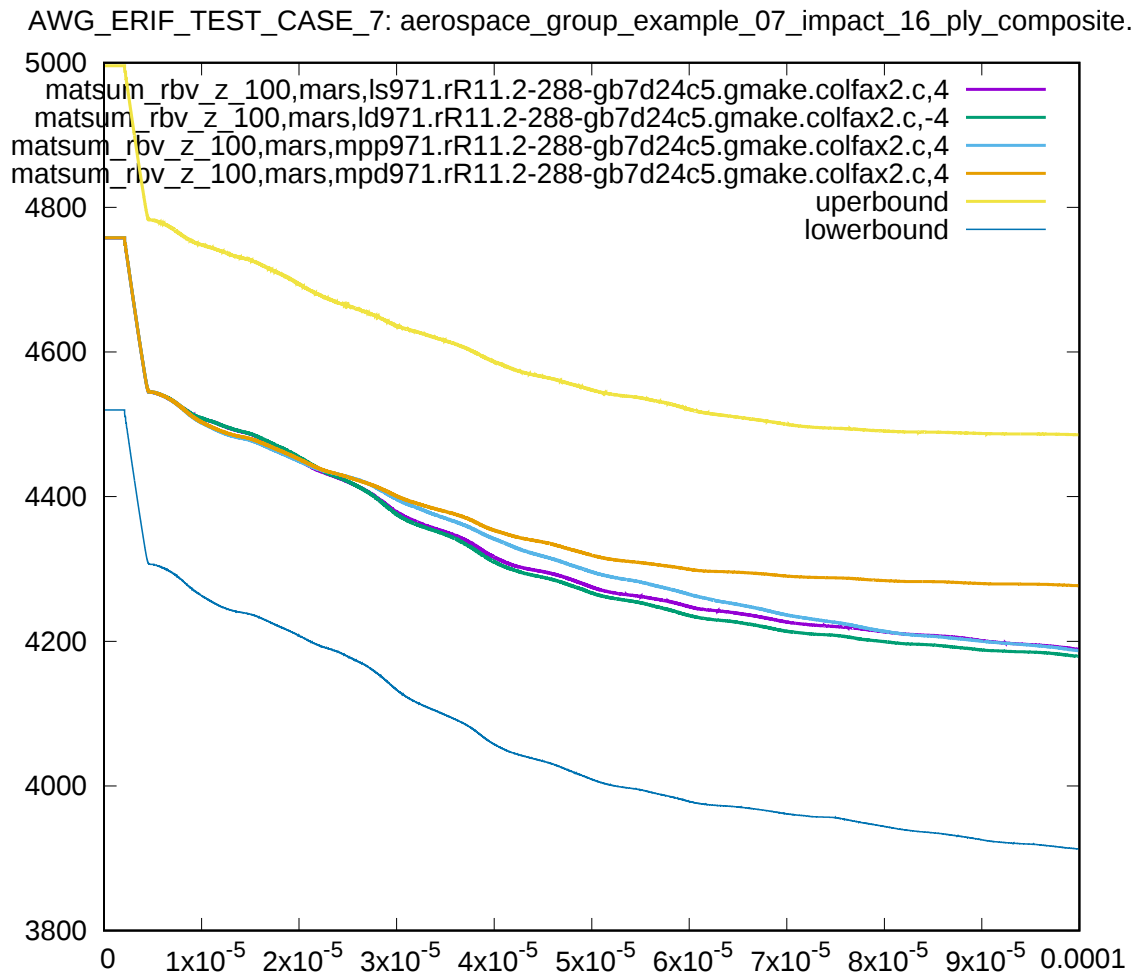
Figure 8: Cross platform results, z-velocity part 100, sub test case ID 1
