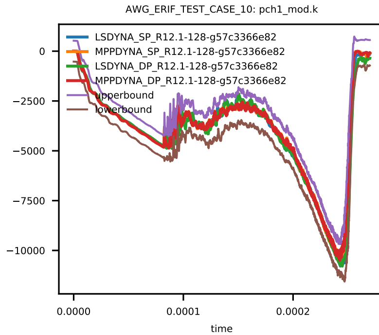
Figure 3: Cross platform results, resultant force in z-direction, sub test case ID 1
