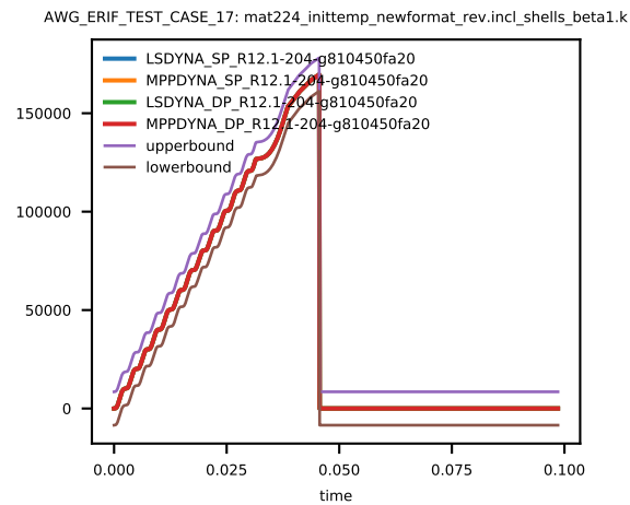
Figure 3: Cross platform results, Von Mises Stress, element ID 4, sub test case ID 2
