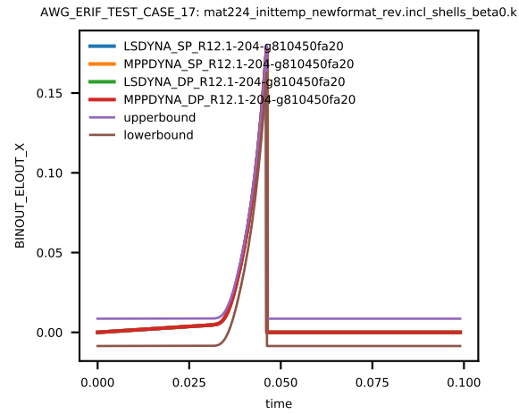
Figure 4: Cross platform results, Effective Plastic Strain, element ID 4, sub test case ID 1
