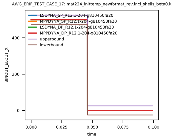
Figure 12: Cross platform results, History Variable 10 (temperature), element ID 14, sub test case ID 1
