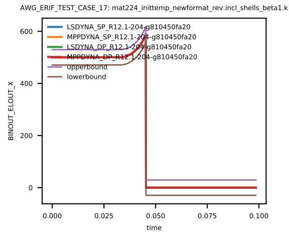
Figure 13: Cross platform results, History Variable 10 (temperature), element ID 14, sub test case ID 2
