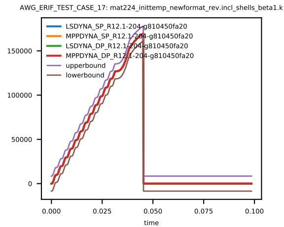
Figure 9: Cross platform results, Von Mises Stress, element ID 14, sub test case ID 2
