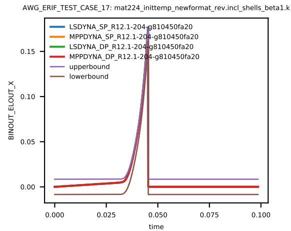
Figure 11: Cross platform results, Effective Plastic Strain, element ID 14, sub test case ID 2
