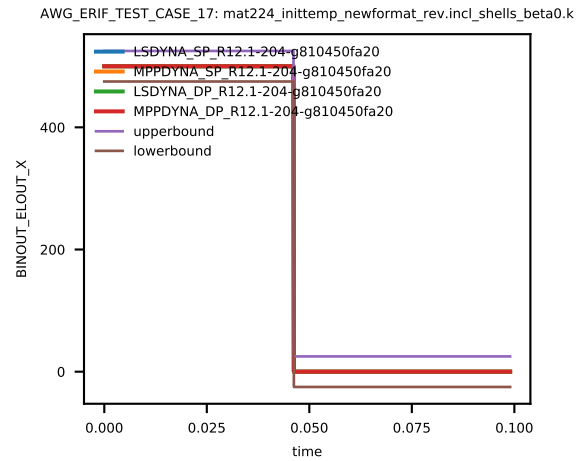
Figure 6: Cross platform results, History Variable 14 (temperature), element ID 4, sub test case ID 1
