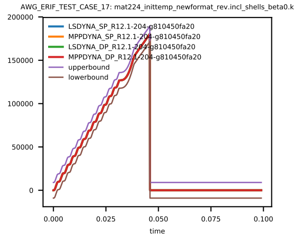
Figure 8: Cross platform results, Von Mises Stress, element ID 14, sub test case ID 1
