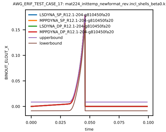
Figure 10: Cross platform results, Effective Plastic Strain, element ID 14, sub test case ID 1
