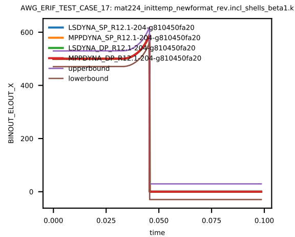
Figure 7: Cross platform results, History Variable 14 (temperature), element ID 4, sub test case ID 2
