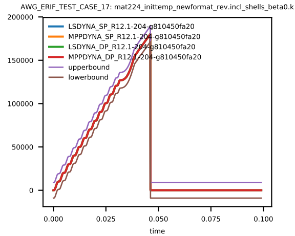
Figure 2: Cross platform results, Von Mises Stress, element ID 4, sub test case ID 1
