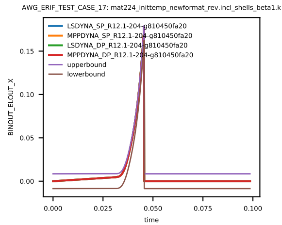
Figure 5: Cross platform results, Effective Plastic Strain, element ID 4, sub test case ID 2
