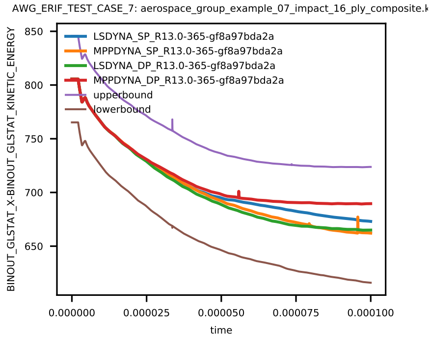
Figure 4: Cross platform results, global kinetic energy, sub test case ID 1
