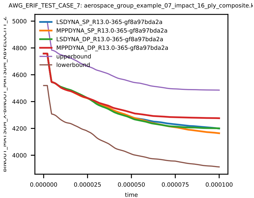
Figure 8: Cross platform results, z-velocity part 100, sub test case ID 1
