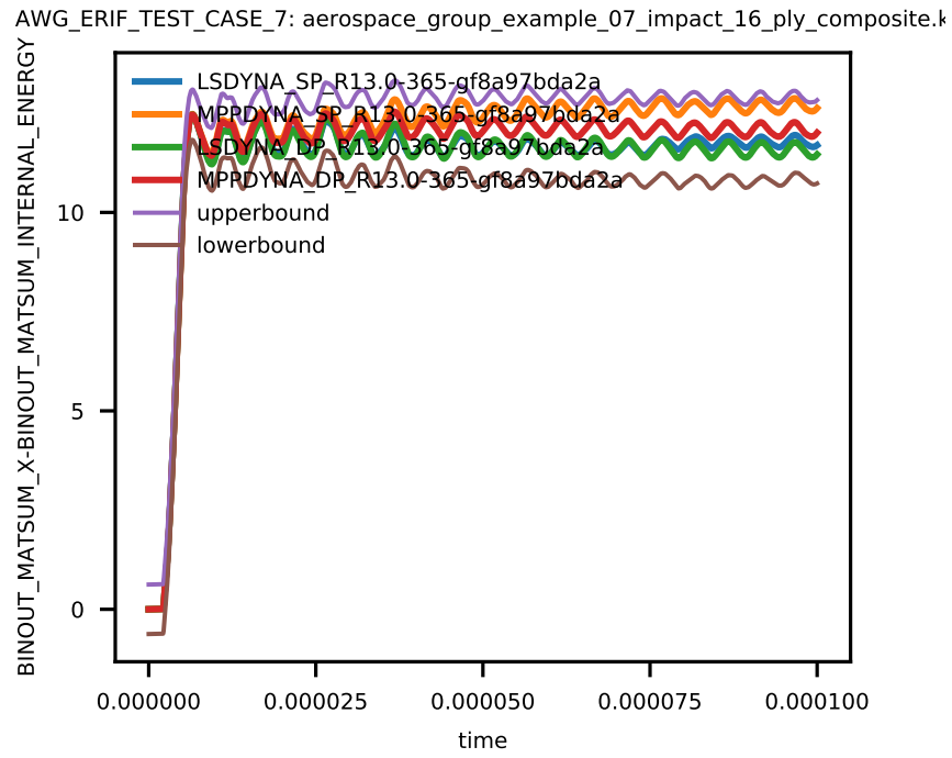
Figure 6: Cross platform results, internal energy part 100, sub test case ID 1
