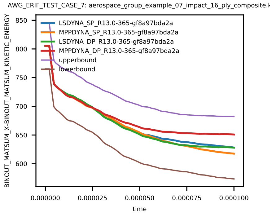
Figure 7: Cross platform results, kinetic energy part 100, sub test case ID 1
