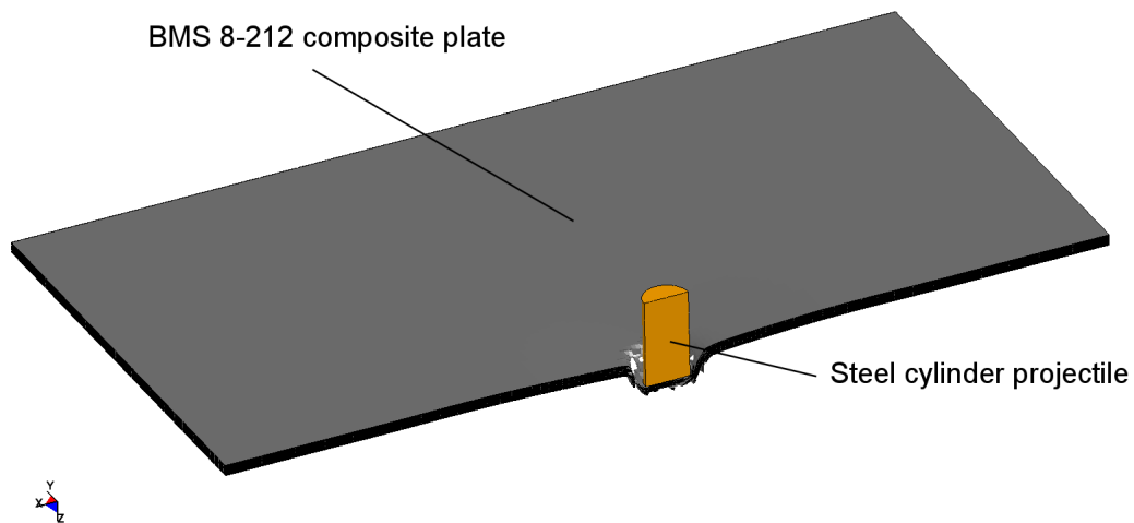
Figure 1: Model sketch: Tool steel cylinder projectile impacting 16 ply BMS 8-212 composite plate
