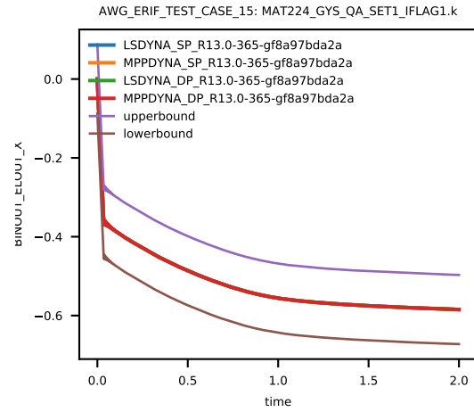
Figure 28: Cross platform results, z-component Stress, element ID 5, sub test case ID 2
