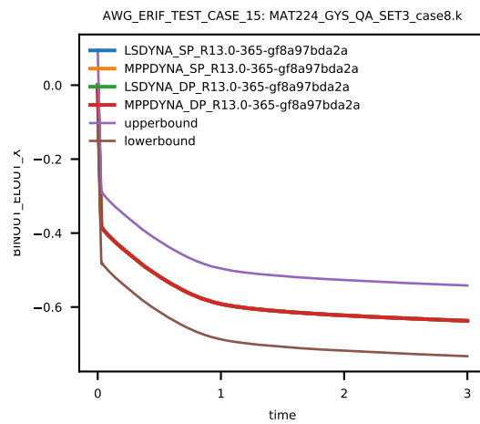
Figure 145: Cross platform results, z-component Stress, element ID 14, sub test case ID 10
