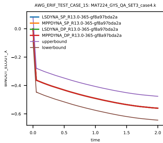
Figure 97: Cross platform results, z-component Stress, element ID 14, sub test case ID 6
