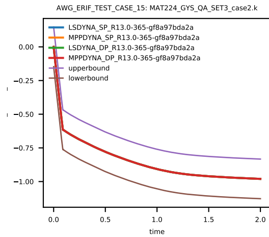
Figure 77: Cross platform results, z-component Stress, element ID 4, sub test case ID 4
