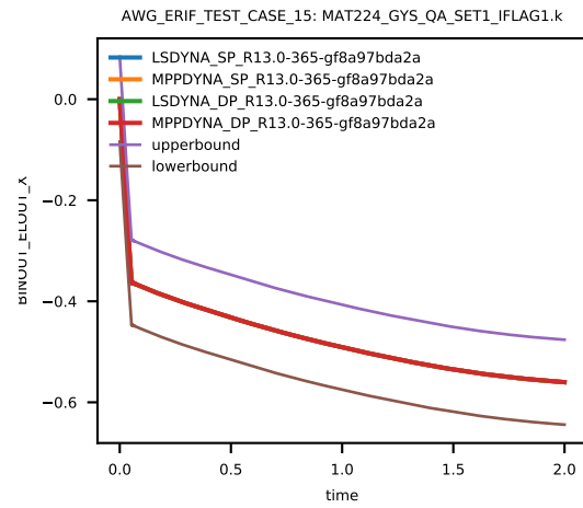
Figure 32: Cross platform results, z-component Stress, element ID 9, sub test case ID 2
