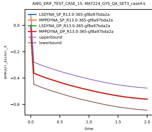
Figure 94: Cross platform results, z-component Stress, element ID 4, sub test case ID 6
