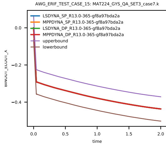
Figure 130: Cross platform results, z-component Stress, element ID 4, sub test case ID 9
