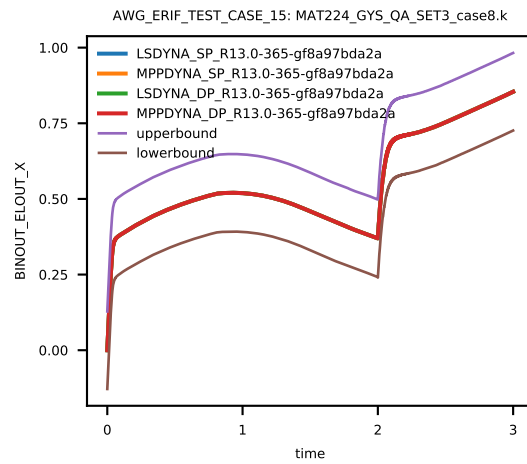
Figure 141: Cross platform results, z-component Stress, element ID 3, sub test case ID 10
