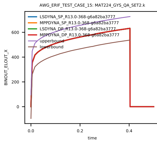
Figure 67: Cross platform results, Von Mises Stress, element ID 16, sub test case ID 3
