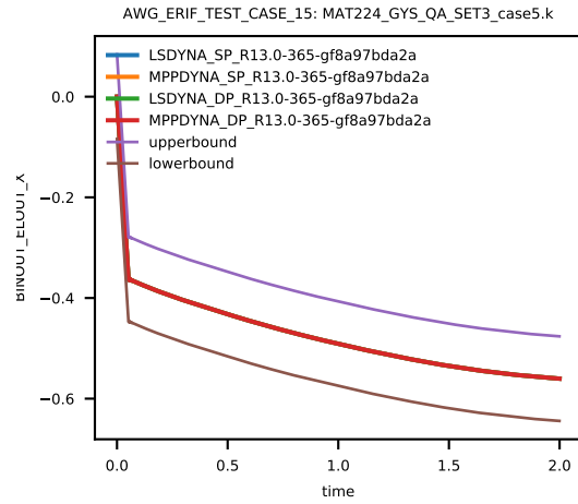
Figure 106: Cross platform results, z-component Stress, element ID 4, sub test case ID 7
