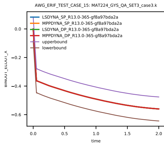
Figure 87: Cross platform results, z-component Stress, element ID 14, sub test case ID 5
