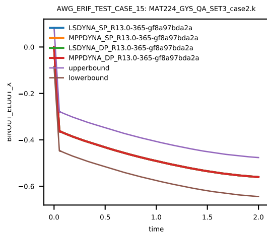
Figure 79: Cross platform results, z-component Stress, element ID 14, sub test case ID 4
