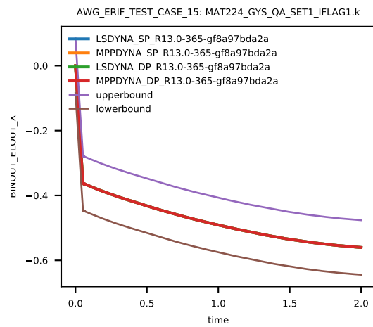
Figure 27: Cross platform results, z-component Stress, element ID 4, sub test case ID 2
