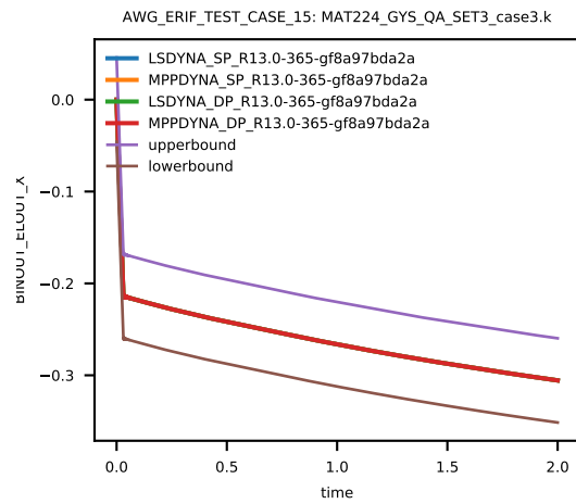
Figure 85: Cross platform results, z-component Stress, element ID 4, sub test case ID 5
