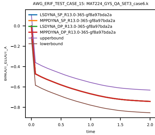
Figure 118: Cross platform results, z-component Stress, element ID 4, sub test case ID 8
