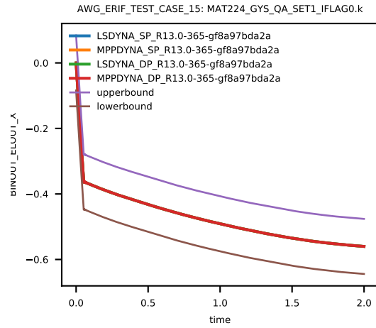
Figure 12: Cross platform results, z-component Stress, element ID 9, sub test case ID 1
