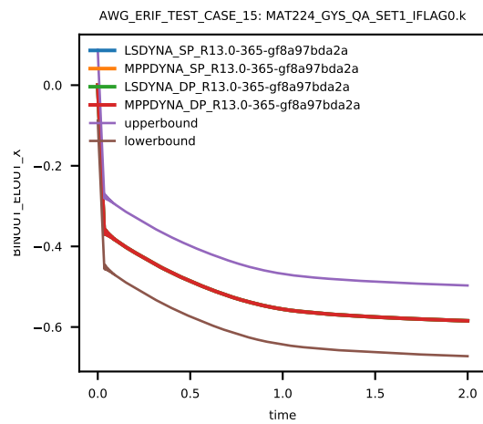
Figure 13: Cross platform results, z-component Stress, element ID 10, sub test case ID 1
