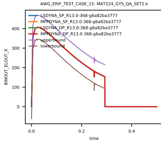
Figure 70: Cross platform results, Von Mises Stress, element ID 19, sub test case ID 3
