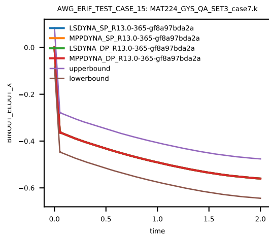
Figure 133: Cross platform results, z-component Stress, element ID 14, sub test case ID 9
