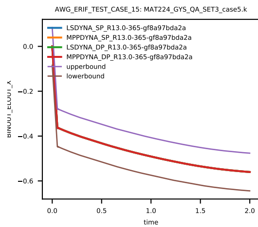
Figure 109: Cross platform results, z-component Stress, element ID 14, sub test case ID 7
