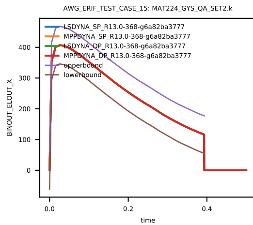
Figure 71: Cross platform results, Von Mises Stress, element ID 20, sub test case ID 3
