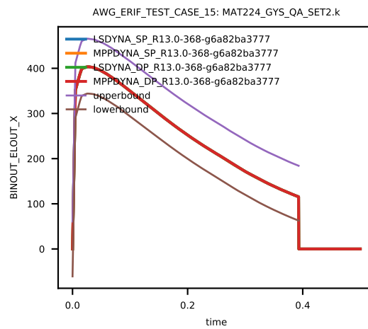
Figure 63: Cross platform results, Von Mises Stress, element ID 12, sub test case ID 3
