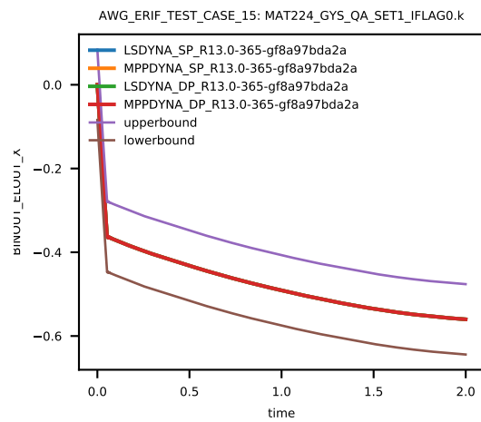
Figure 7: Cross platform results, z-component Stress, element ID 4, sub test case ID 1
