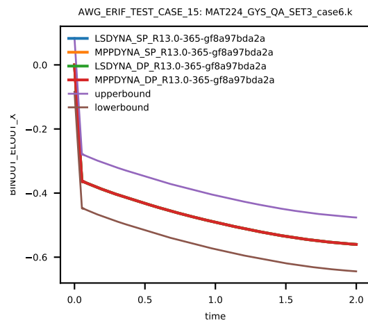
Figure 121: Cross platform results, z-component Stress, element ID 14, sub test case ID 8
