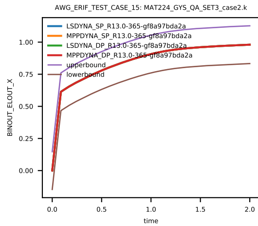
Figure 81: Cross platform results, Von Mises Stress, element ID 4, sub test case ID 4
