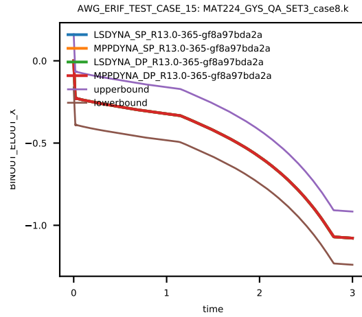
Figure 142: Cross platform results, z-component Stress, element ID 4, sub test case ID 10
