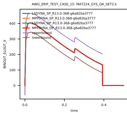
Figure 47: Cross platform results, z-component Stress, element ID 12, sub test case ID 3
