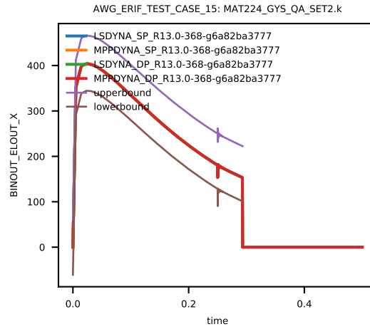
Figure 62: Cross platform results, Von Mises Stress, element ID 11, sub test case ID 3
