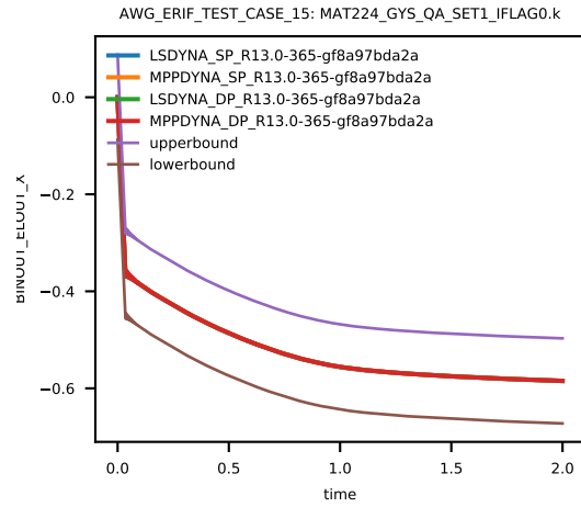
Figure 8: Cross platform results, z-component Stress, element ID 5, sub test case ID 1
