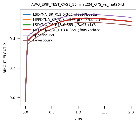
Figure 7: Cross platform results, z-component Stress, element ID 11, sub test case ID 1
