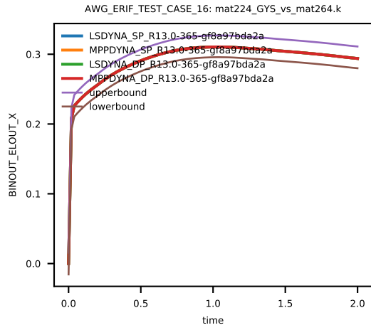
Figure 4: Cross platform results, z-component Stress, element ID 3, sub test case ID 1
