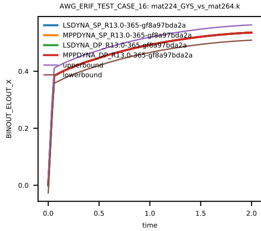
Figure 18: Cross platform results, Von Mises Stress, element ID 12, sub test case ID 1
