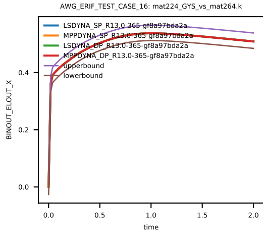
Figure 14: Cross platform results, Von Mises Stress, element ID 3, sub test case ID 1
