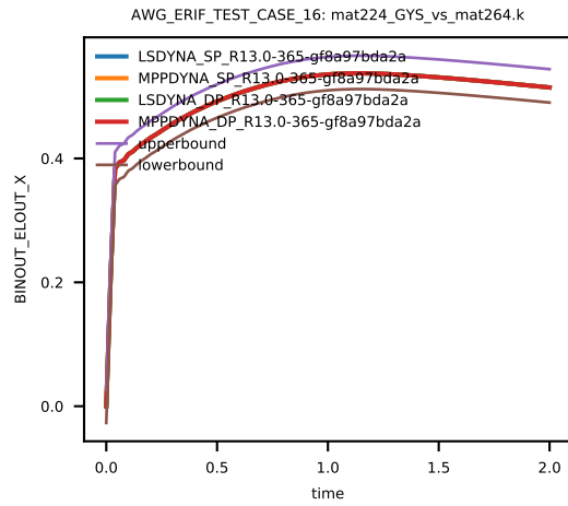
Figure 2: Cross platform results, z-component Stress, element ID 1, sub test case ID 1
