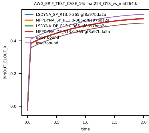
Figure 8: Cross platform results, z-component Stress, element ID 12, sub test case ID 1
