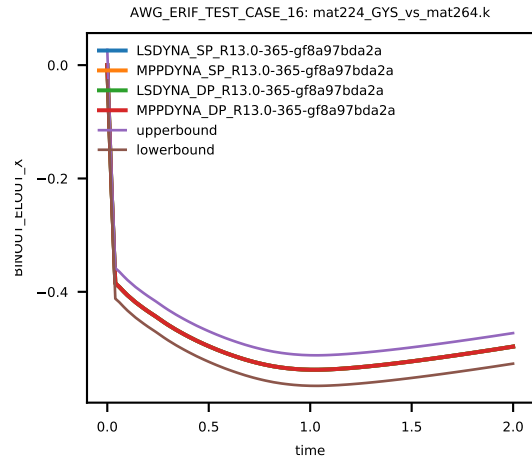
Figure 6: Cross platform results, z-component Stress, element ID 5, sub test case ID 1
