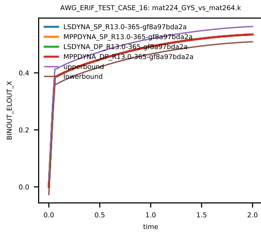
Figure 3: Cross platform results, z-component Stress, element ID 2, sub test case ID 1
