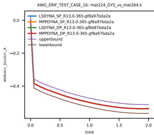
Figure 5: Cross platform results, z-component Stress, element ID 4, sub test case ID 1
