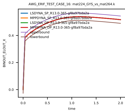
Figure 17: Cross platform results, Von Mises Stress, element ID 11, sub test case ID 1
