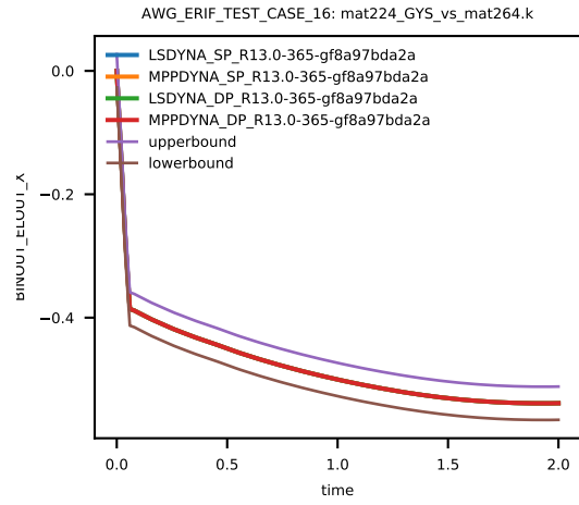
Figure 10: Cross platform results, z-component Stress, element ID 14, sub test case ID 1
