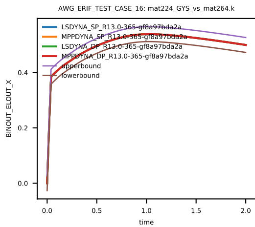
Figure 21: Cross platform results, Von Mises Stress, element ID 10, sub test case ID 1
