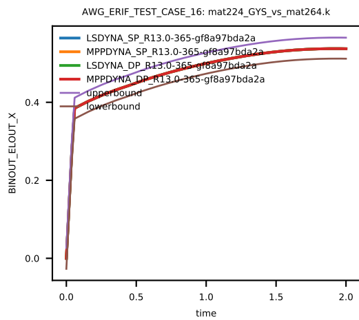
Figure 15: Cross platform results, Von Mises Stress, element ID 4, sub test case ID 1
