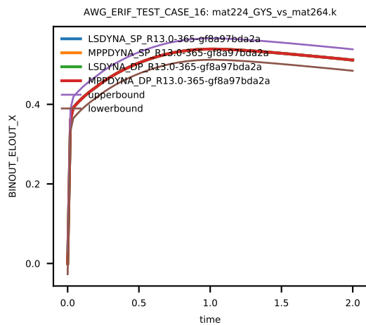
Figure 19: Cross platform results, Von Mises Stress, element ID 13, sub test case ID 1
