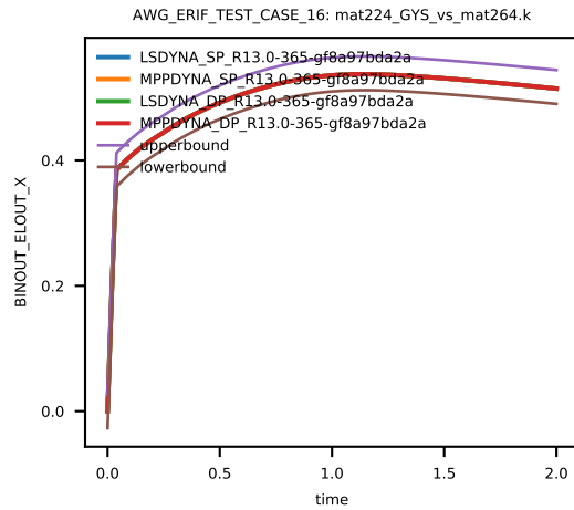
Figure 12: Cross platform results, Von Mises Stress, element ID 1, sub test case ID 1
