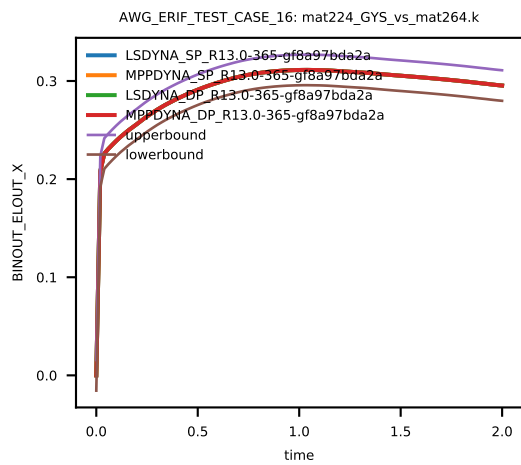
Figure 9: Cross platform results, z-component Stress, element ID 13, sub test case ID 1
