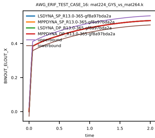
Figure 13: Cross platform results, Von Mises Stress, element ID 2, sub test case ID 1
