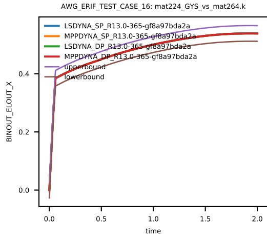
Figure 20: Cross platform results, Von Mises Stress, element ID 14, sub test case ID 1
