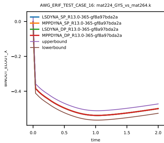
Figure 11: Cross platform results, z-component Stress, element ID 10, sub test case ID 1
