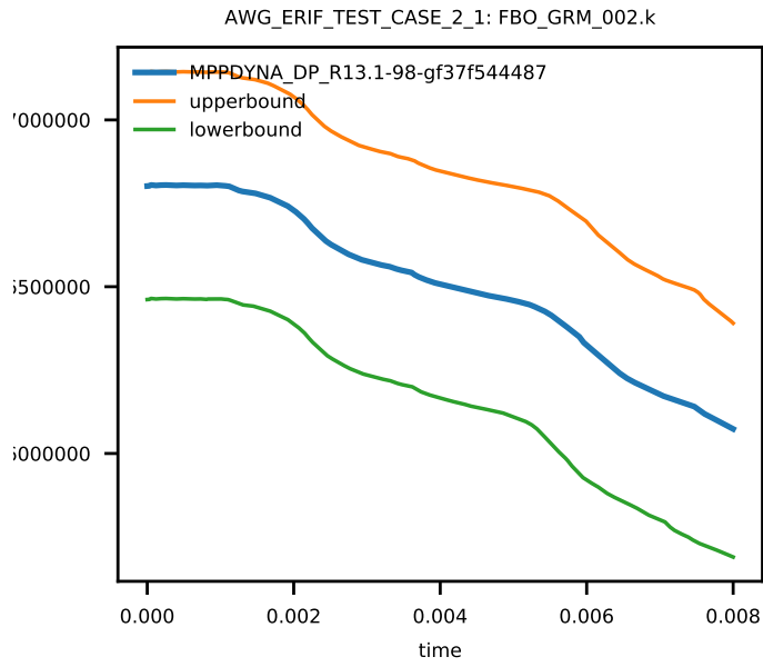
Figure 3: Global kinetic energy, sub test case ID 1
