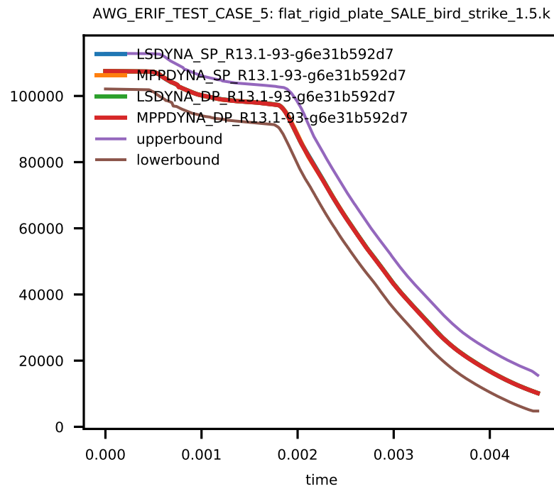
Figure 13: Cross platform results, kinetic energy part 910002 (bird body), sub test case ID 5
