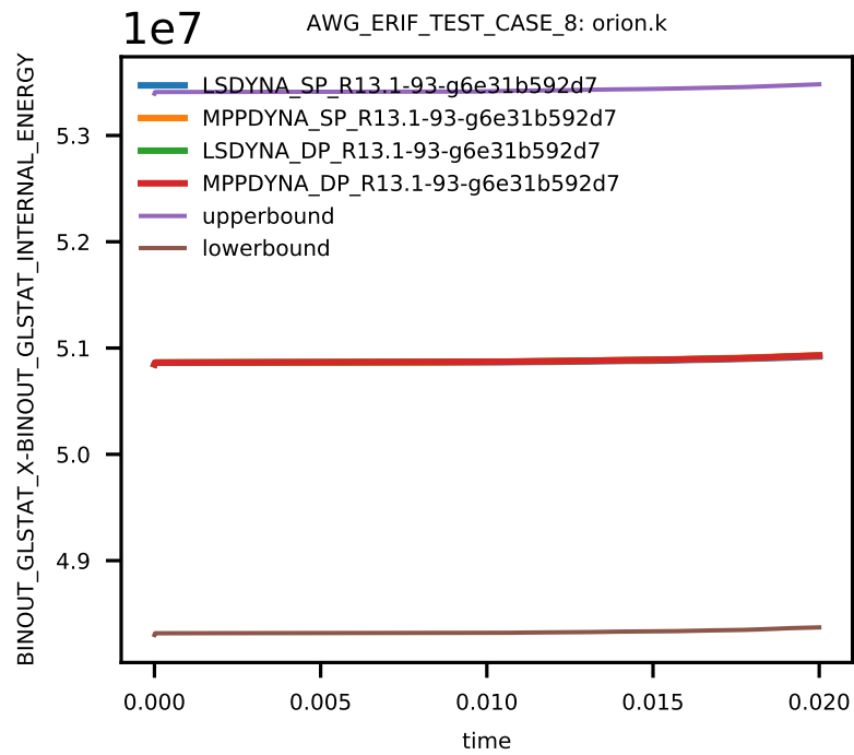
Figure 4: Cross platform results, global internal energy, sub test case ID 1
