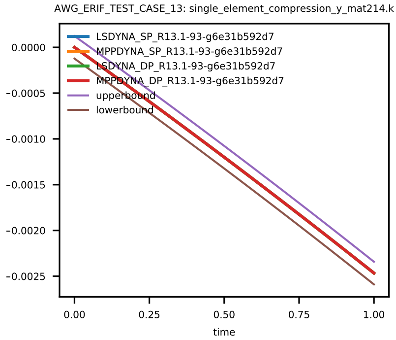
Figure 6: Cross platform results, stress in y-direction, integration point 1, sub test case ID 4
