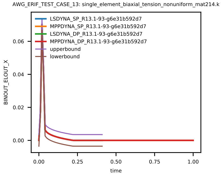
Figure 11: Cross platform results, stress in x-direction, integration point 1, sub test case ID 7
