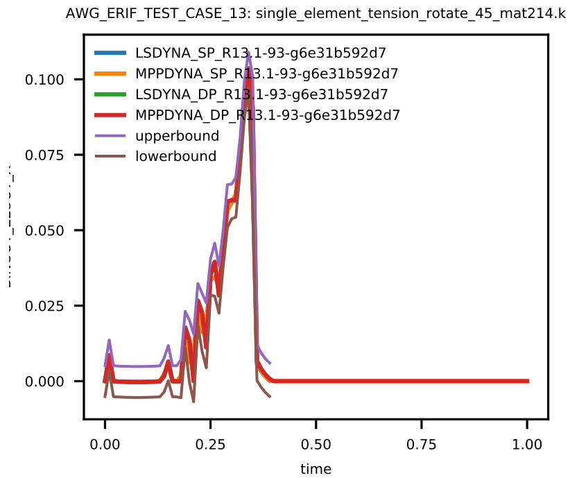
Figure 8: Cross platform results, stress in y-direction, integration point 1, sub test case ID 5
