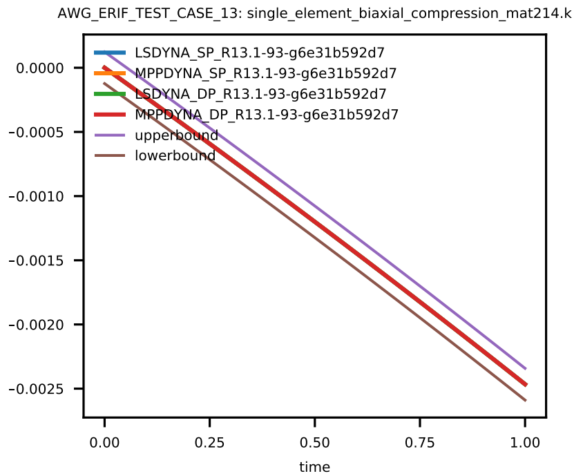
Figure 14: Cross platform results, stress in y-direction, integration point 1, sub test case ID 8
