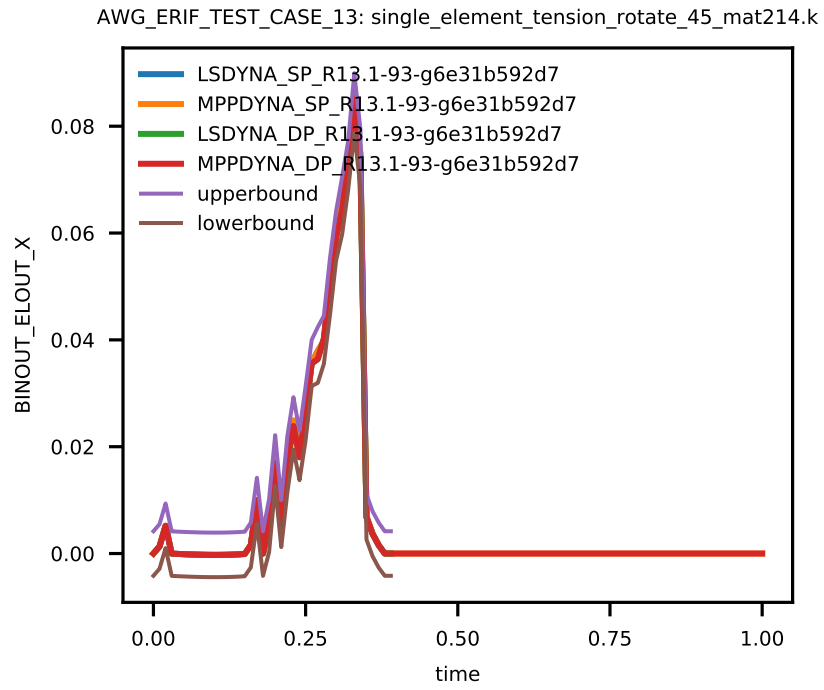
Figure 7: Cross platform results, stress in x-direction, integration point 1, sub test case ID 5
