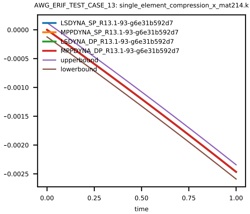
Figure 5: Cross platform results, stress in x-direction, integration point 1, sub test case ID 3
