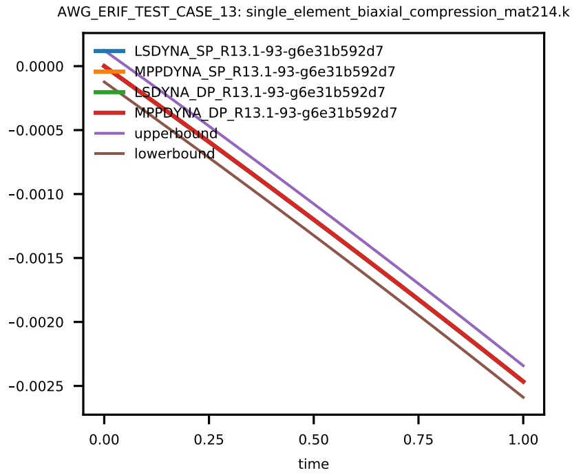
Figure 13: Cross platform results, stress in x-direction, integration point 1, sub test case ID 8
