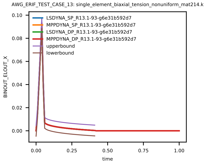
Figure 12: Cross platform results, stress in y-direction, integration point 1, sub test case ID 7
