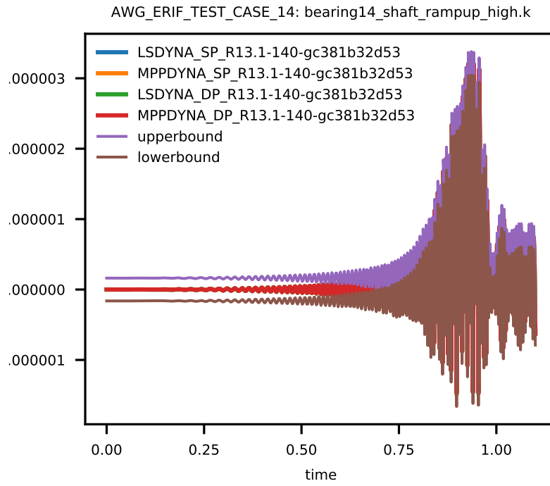
Figure 2: Cross platform results, node displacement in y-direction, node id 1, sub test case ID 1
