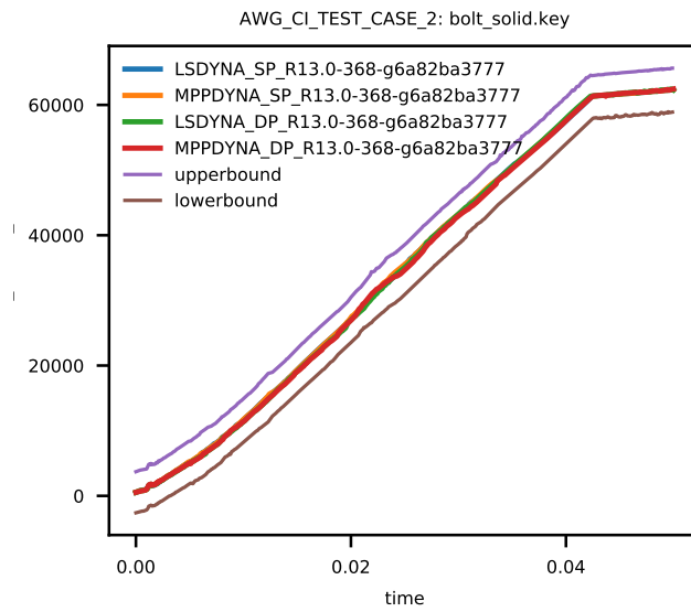
Figure 3: Cross platform results, Von Mises stress of element 65559, sub test case ID 1
