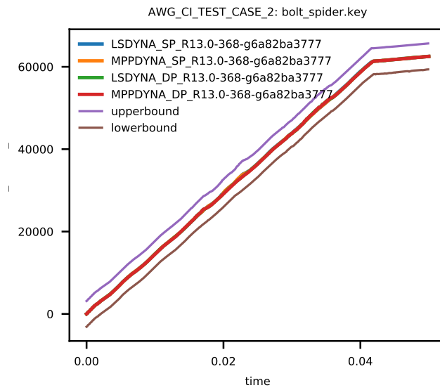
Figure 5: Cross platform results, Von Mises stress of element 66872, sub test case ID 2
