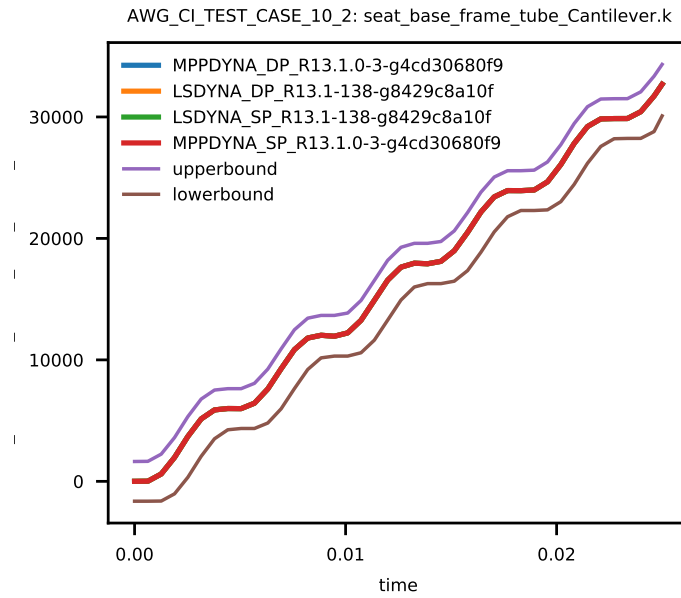
Figure 8: Von Mises Stress of Element 353.
