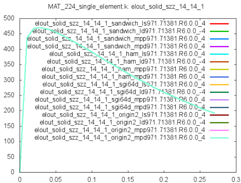
Figure 16: Cross platform results, zz stress element id 14, sub test case ID 1
