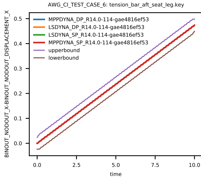
Figure 3: X-component Displacement of Node 1301.
