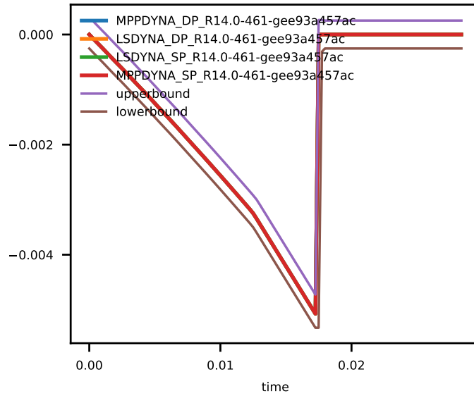
Figure 9: Solid Element Strain zz.
