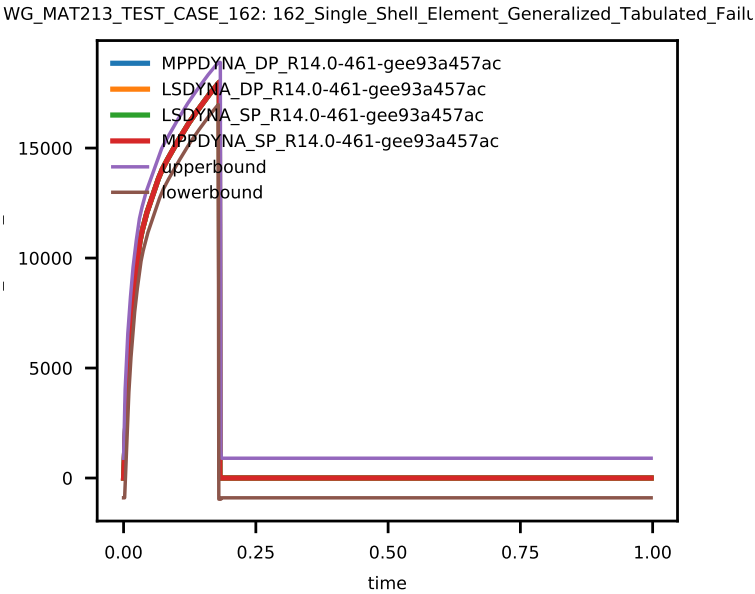
Figure 5: Shell Element Stress yy at integration point 2.
