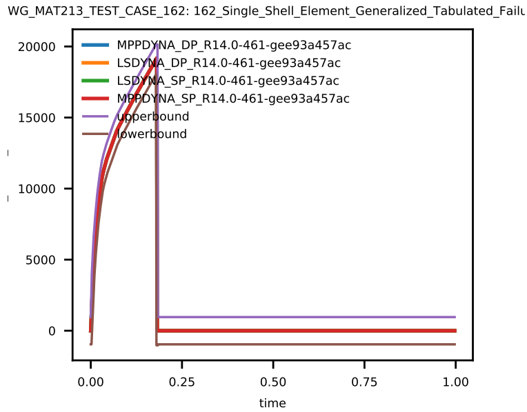
Figure 11: Shell Element Stress yy at integration point 4.
