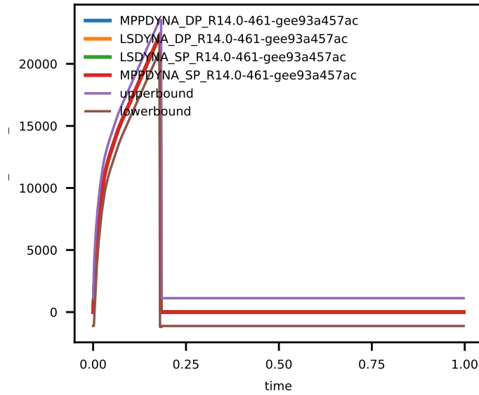
Figure 2: Shell Element Stress yy at integration point 1.
