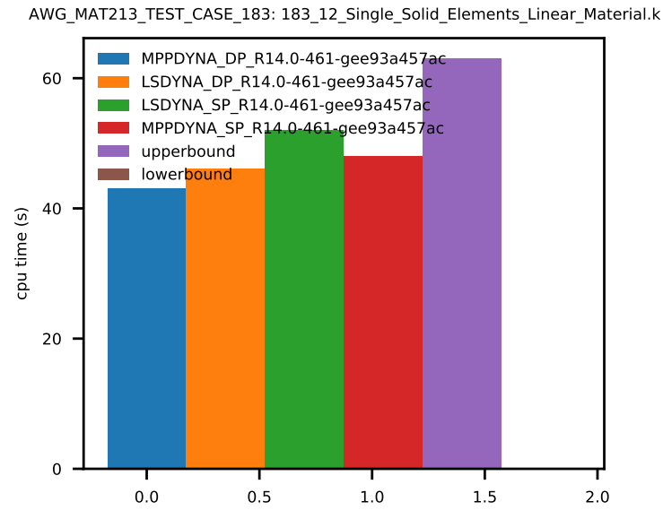
Figure 28: CPU Time.
