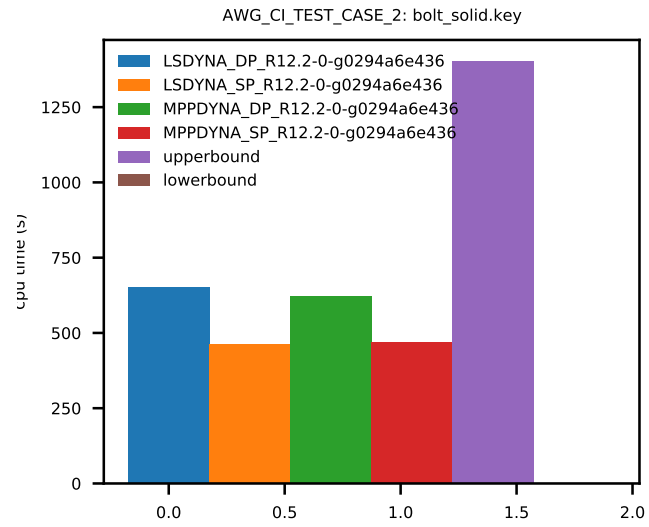
Figure 6: Cross platform results, CPU time
