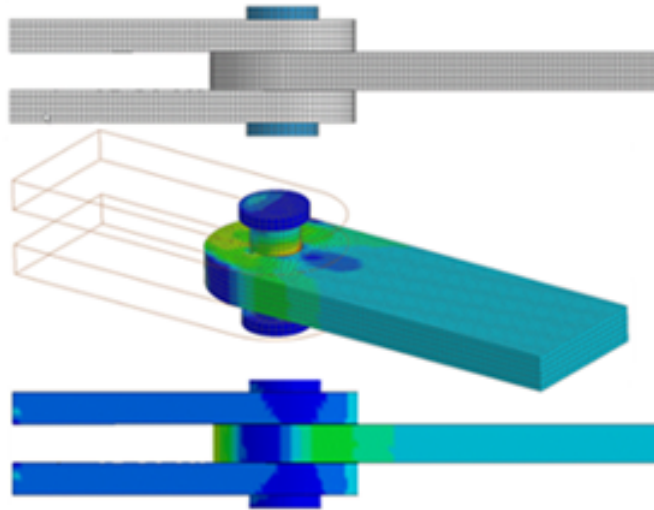
Figure 1: Lug Joint.
