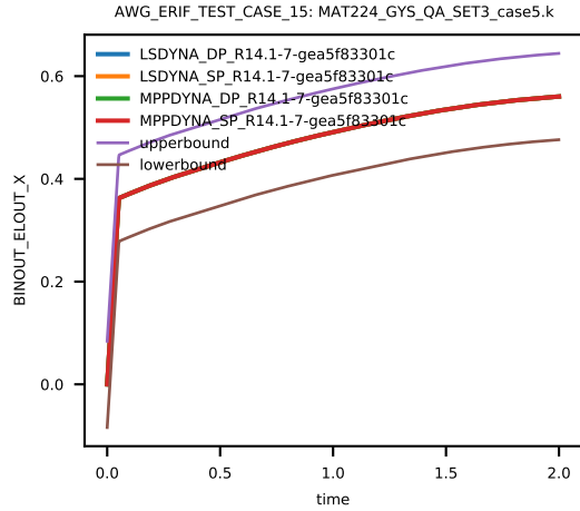
Figure 112: Cross platform results, Von Mises Stress, element ID 4, sub test case ID 7
