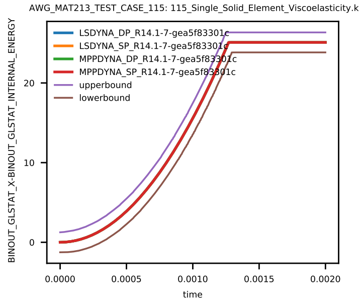
Figure 8: Global Internal Energy.
