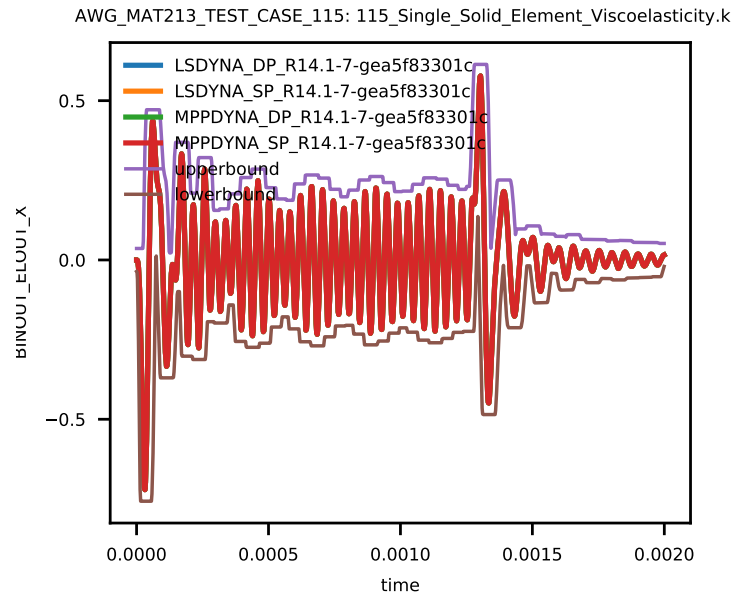
Figure 6: Solid Element Stress \sigma_{zx} .
