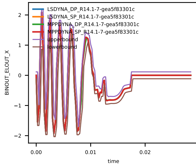
Figure 12: Solid Element Strain zx.
