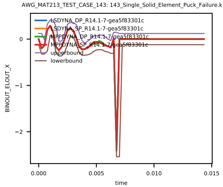
Figure 6: Solid Element Stress \sigma_{zx} .
