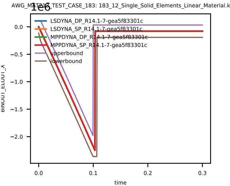
Figure 5: Stress xx of Solid Element 5.
