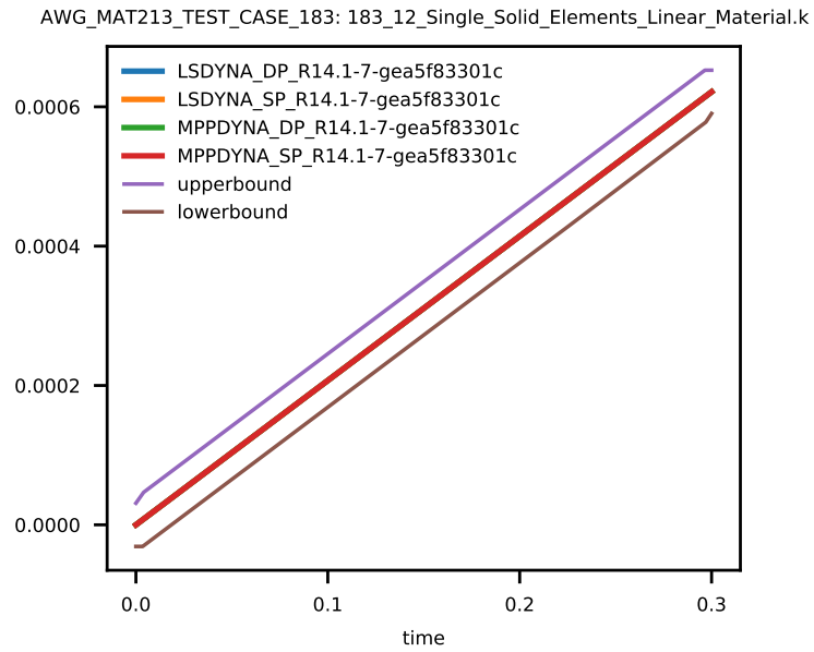
Figure 21: Strain xx of Solid Element 9.
