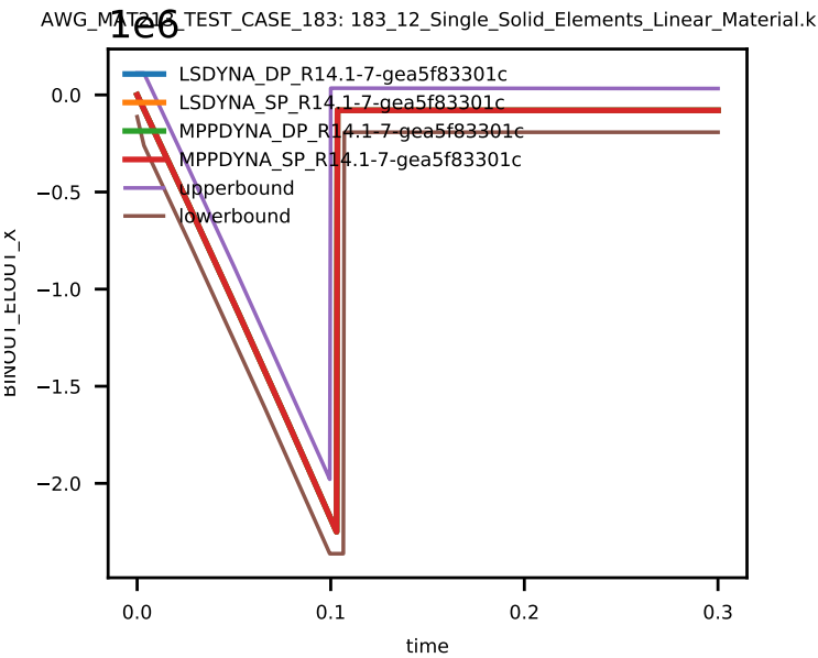
Figure 10: Stress xx of Solid Element 10.
