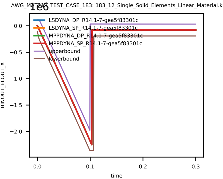
Figure 7: Stress xx of Solid Element 7.
