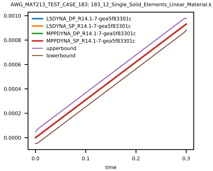
Figure 19: Strain xx of Solid Element 7.
