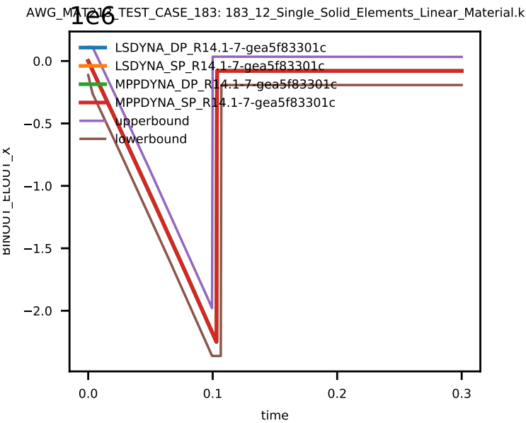
Figure 11: Stress xx of Solid Element 11.
