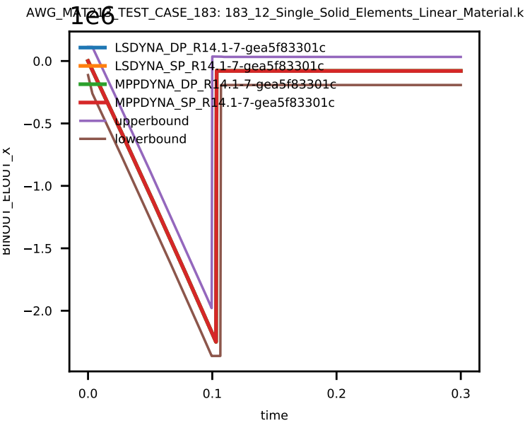
Figure 9: Stress xx of Solid Element 9.
