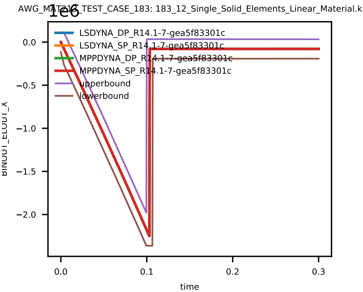
Figure 4: Stress xx of Solid Element 4.
