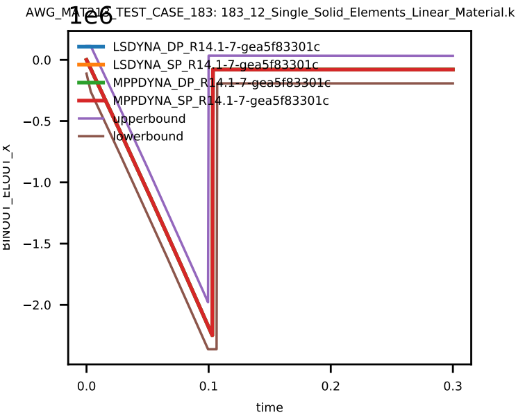
Figure 6: Stress xx of Solid Element 6.
