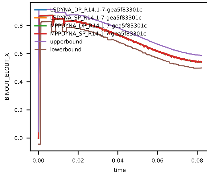
Figure 3: Solid Element Stress zz.
