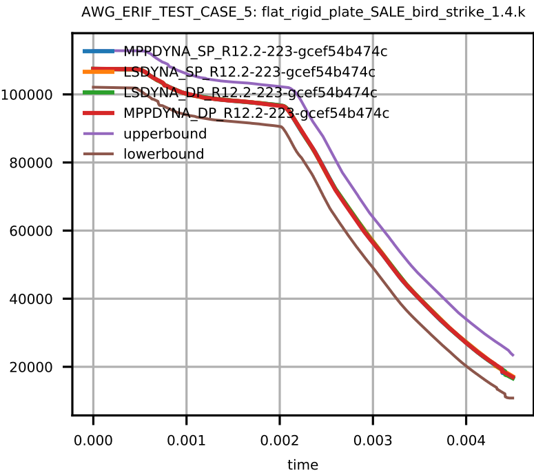
Figure 11: Cross platform results, kinetic energy part 910002 (bird body), sub test case ID 4
