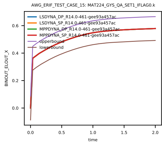
Figure 14: Cross platform results, Von Mises Stress, element ID 1, sub test case ID 1
