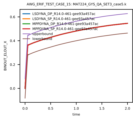
Figure 104: Cross platform results, z-component Stress, element ID 2, sub test case ID 7
