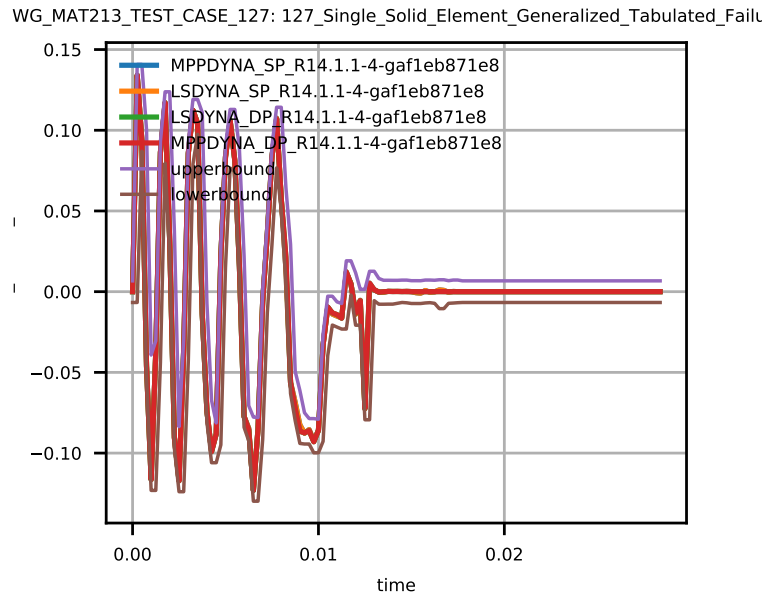
Figure 2: Solid Element Stress \sigma_{yy} .
